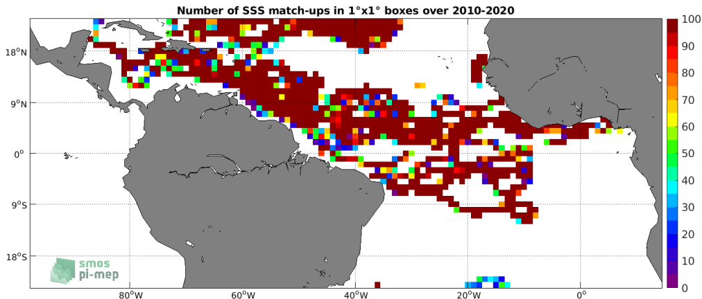
Figure 3: Number of SSS match-ups between Surface drifters SSS and the SMOS SSS L3 v5 - 18 Days (CATDS-CECOS-LOCEAN) SSS product for the Tropical Atlantic Ocean Pi-MEP region over 1^\circ \times 1^\circ boxes and for the full satellite product period.
