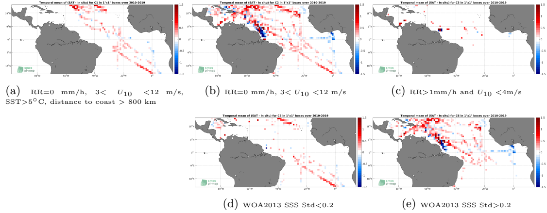
Figure 12: Temporal mean gridded over spatial boxes of size 1^{\circ}\times 1^{\circ} of \Delta\text{SSS} (SMOS SSS L3 v4 - 9 Days (CATDS-CECOS-LOCEAN) - TSG (SAMOS)) for 5 different subdatasets corresponding to: RR=0 mm/h, 3 < U_{10} < 12 m/s, SST >5^{\circ}\text{C} , distance to coast > 800 km (a), RR=0 mm/h, 3 < U_{10} < 12 m/s (b), RR >1 mm/h and U_{10} < 4 m/s (c), WOA2013 SSS Std <0.2 (d), WOA2013 SSS Std >0.2 (e).
