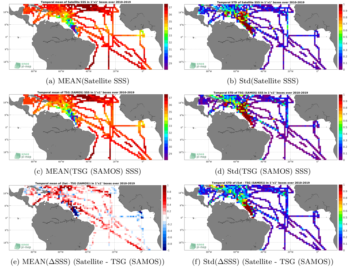
Figure 6: Temporal mean (left) and Std (right) of SSS from SMOS SSS L3 v4 - 9 Days (CATDS-CECOS-LOCEAN) (top), TSG (SAMOS) (middle), and of \Delta SSS (Satellite - TSG (SAMOS)). Only match-up pairs are used to generate these maps.
