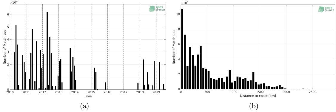
Figure 1: Number of match-ups between TSG (SAMOS) and SMOS SSS L3 v4 - 9 Days (CATDS-CECOS-LOCEAN) SSS as a function of time (a) and as function of the distance to coast (b) over the Tropical Atlantic Ocean Pi-MEP region and for the full satellite product period.
