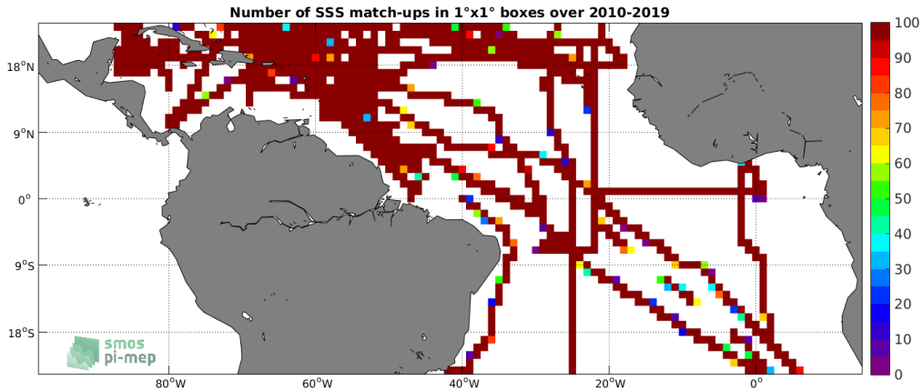
Figure 4: Number of SSS match-ups between TSG (SAMOS) SSS and the SMOS SSS L3 v4 - 9 Days (CATDS-CECOS-LOCEAN) SSS product for the Tropical Atlantic Ocean Pi-MEP region over 1^\circ \times 1^\circ boxes and for the full satellite product period.
