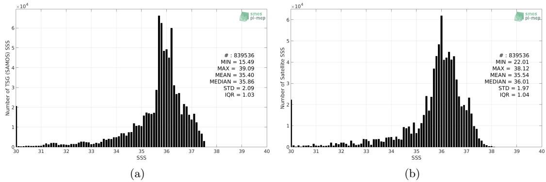
Figure 2: Histograms of SSS from TSG (SAMOS) (a) and SMOS SSS L3 v4 - 9 Days (CATDS-CECOS-LOCEAN) (b) considering all match-up pairs per bins of 0.1 over the Tropical Atlantic Ocean Pi-MEP region and for the full satellite product period.
