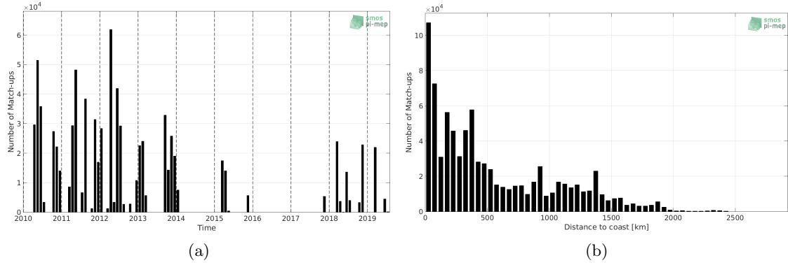
Figure 1: Number of match-ups between TSG-SAMOS and SMOS-L3-CATDS-CECOS-LOCEAN-V4-9DAYS-25KM SSS as a function of time (a) and as function of the distance to coast (b) over the Tropical Atlantic Ocean Pi-MEP region and for the full satellite product period.
