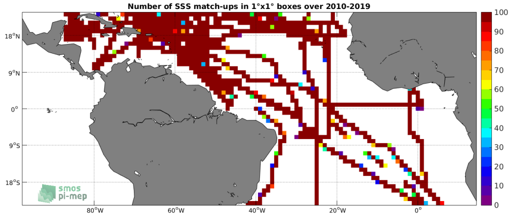
Figure 4: Number of SSS match-ups between TSG-SAMOS SSS and the SMOS-L3-CATDS-CECOS-LOCEAN-V4-9DAYS-25KM SSS product for the Tropical Atlantic Ocean Pi-MEP region over 1°x1° boxes and for the full satellite product period.
