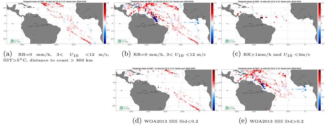
Figure 12: Temporal mean gridded over spatial boxes of size 1^{\circ}\times 1^{\circ} of \Delta\text{SSS} (SMOS-L3-CATDS-CECOS-LOCEAN-V4-9DAYS-25KM - TSG-SAMOS) for 5 different subdatasets corresponding to:RR=0 mm/h, 3 < U_{10} < 12 m/s, SST >5^{\circ}\text{C} , distance to coast > 800 km (a), RR=0 mm/h, 3 < U_{10} < 12 m/s (b), RR >1 mm/h and U_{10} < 4 m/s (c), WOA2013 SSS Std <0.2 (d), WOA2013 SSS Std >0.2 (e).
