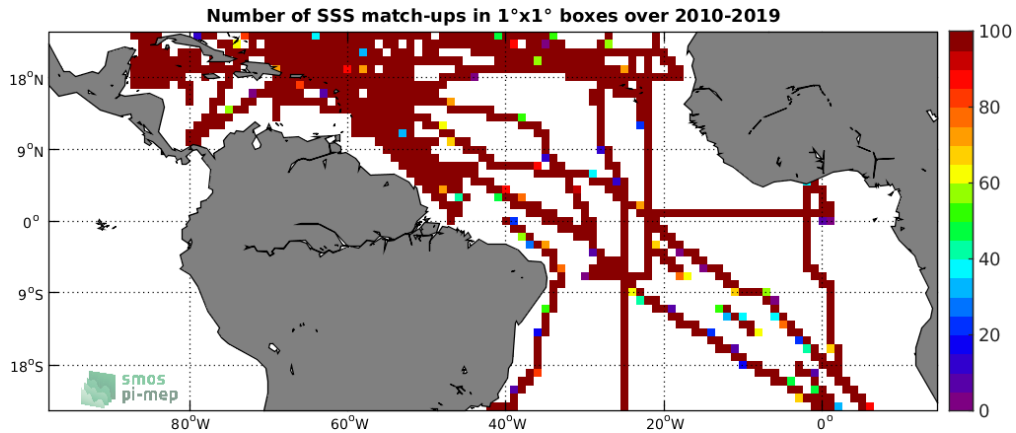
Figure 4: Number of SSS match-ups between TSG-SAMOS SSS and the SMOS-L3-CATDS-CECOS-LOCEAN-V4-9DAYS-25KM SSS product for the Tropical Atlantic Ocean Pi-MEP region over 1^\circ \times 1^\circ boxes and for the full satellite product period.
