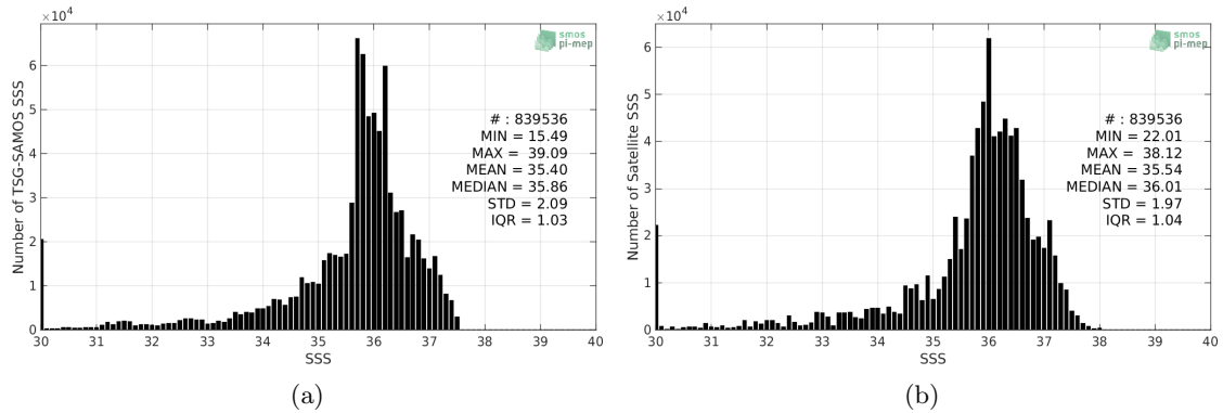
Figure 2: Histograms of SSS from TSG-SAMOS (a) and SMOS-L3-CATDS-CECOS-LOCEAN-V4-9DAYS-25KM (b) considering all match-up pairs per bins of 0.1 over the Tropical Atlantic Ocean Pi-MEP region and for the full satellite product period.
