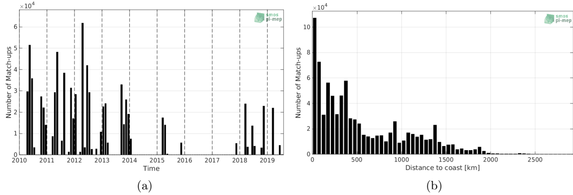
Figure 1: Number of match-ups between TSG-SAMOS and SMOS-L3-CATDS-CECOS-LOCEAN-V4-9DAYS-25KM SSS as a function of time (a) and as function of the distance to coast (b) over the Tropical Atlantic Ocean Pi-MEP region and for the full satellite product period.
