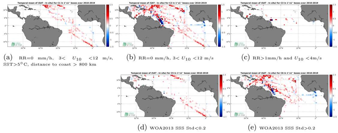
Figure 12: Temporal mean gridded over spatial boxes of size 1^\circ \times 1^\circ of \Delta SSS (SMOS-L3-CATDS-CECOS-LOCEAN-V4-9DAYS-25KM - TSG-SAMOS) for 5 different subdatasets corresponding to:RR=0 mm/h, 3 < U_{10} < 12 m/s, SST >5^\circ\text{C} , distance to coast > 800 km (a), RR=0 mm/h, 3 < U_{10} < 12 m/s (b), RR >1 mm/h and U_{10} < 4 m/s (c), WOA2013 SSS Std <0.2 (d), WOA2013 SSS Std >0.2 (e).
