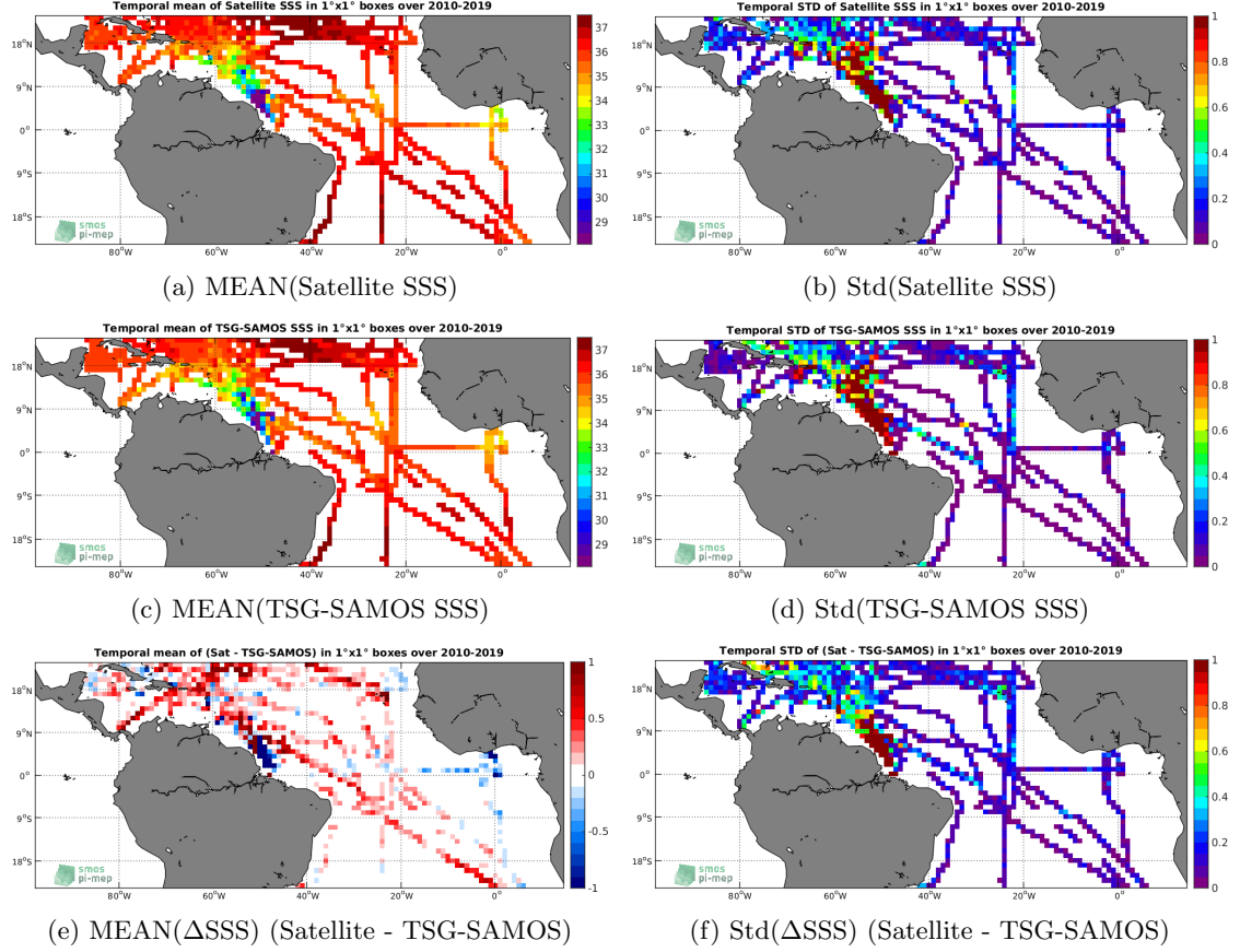
Figure 6: Temporal mean (left) and Std (right) of SSS from SMOS-L3-CATDS-CECOS-LOCEAN-V4-9DAYS-25KM (top), TSG-SAMOS (middle), and of \Delta SSS (Satellite - TSG-SAMOS). Only match-up pairs are used to generate these maps.
