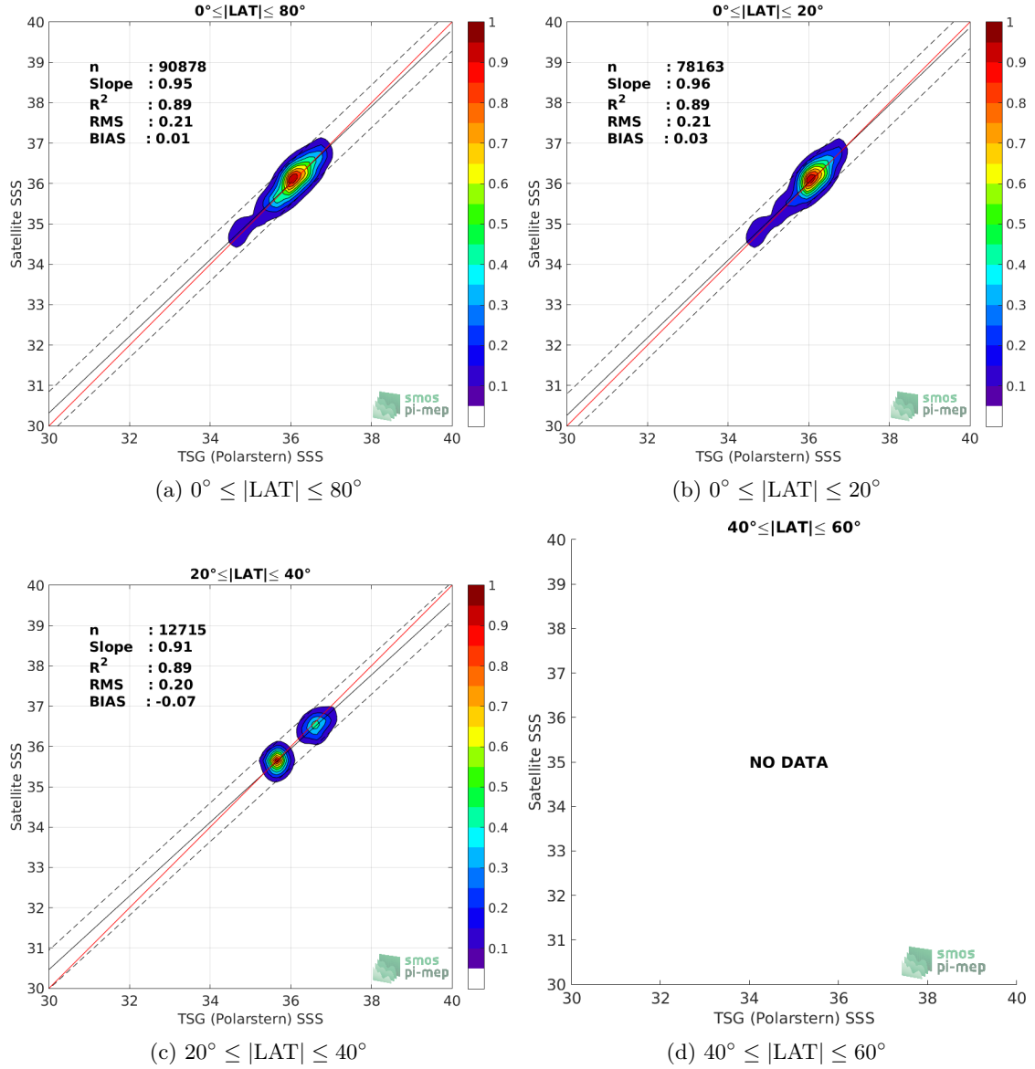
Figure 9: Contour maps of the concentration of SMOS SSS L3 v4 - 9 Days (CATDS-CECOS-LOCEAN) SSS (y-axis) versus TSG (Polarstern) SSS (x-axis) at match-up pairs for different latitude bands. For each plot, the red line shows x=y . The black thin and dashed lines indicate a linear fit through the data cloud and the \pm 95\% confidence levels, respectively. The number match-up pairs n , the slope and R^2 coefficient of the linear fit, the root mean square (RMS) and the mean bias between satellite and in situ data are indicated for each latitude band in each plots.
