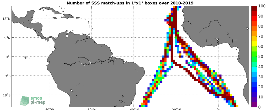
Figure 4: Number of SSS match-ups between TSG (Polarstern) SSS and the SMOS SSS L3 v4 - 9 Days (CATDS-CECOS-LOCEAN) SSS product for the Tropical Atlantic Ocean Pi-MEP region over 1^\circ \times 1^\circ boxes and for the full satellite product period.
