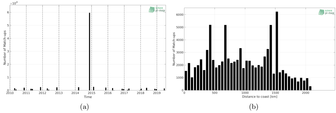
Figure 1: Number of match-ups between TSG (Polarstern) and SMOS SSS L3 v4 - 9 Days (CATDS-CECOS-LOCEAN) SSS as a function of time (a) and as function of the distance to coast (b) over the Tropical Atlantic Ocean Pi-MEP region and for the full satellite product period.
