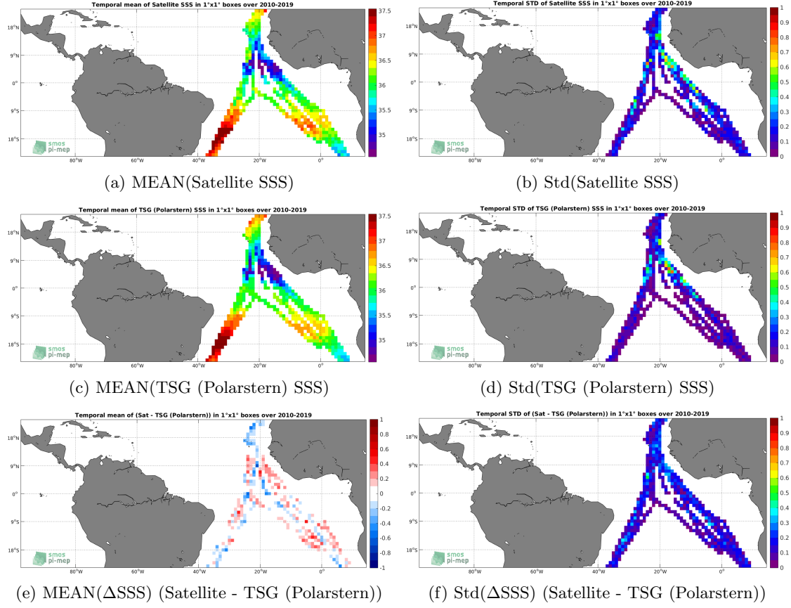
Figure 6: Temporal mean (left) and Std (right) of SSS from SMOS SSS L3 v4 - 9 Days (CATDS-CECOS-LOCEAN) (top), TSG (Polarstern) (middle), and of \Delta SSS (Satellite - TSG (Polarstern)). Only match-up pairs are used to generate these maps.
