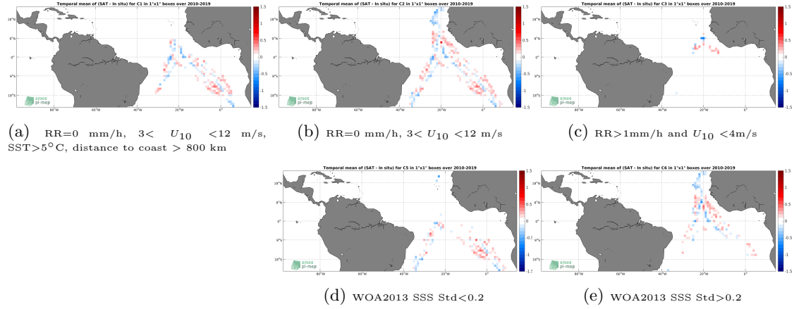
Figure 12: Temporal mean gridded over spatial boxes of size 1^{\circ}\times 1^{\circ} of \Delta\text{SSS} (SMOS SSS L3 v4 - 9 Days (CATDS-CECOS-LOCEAN) - TSG (Polarstern)) for 5 different subdatasets corresponding to: RR=0 mm/h, 3 < U_{10} < 12 m/s, SST >5^{\circ}\text{C} , distance to coast > 800 km (a), RR=0 mm/h, 3 < U_{10} < 12 m/s (b), RR >1 mm/h and U_{10} < 4 m/s (c), WOA2013 SSS Std <0.2 (d), WOA2013 SSS Std >0.2 (e).
