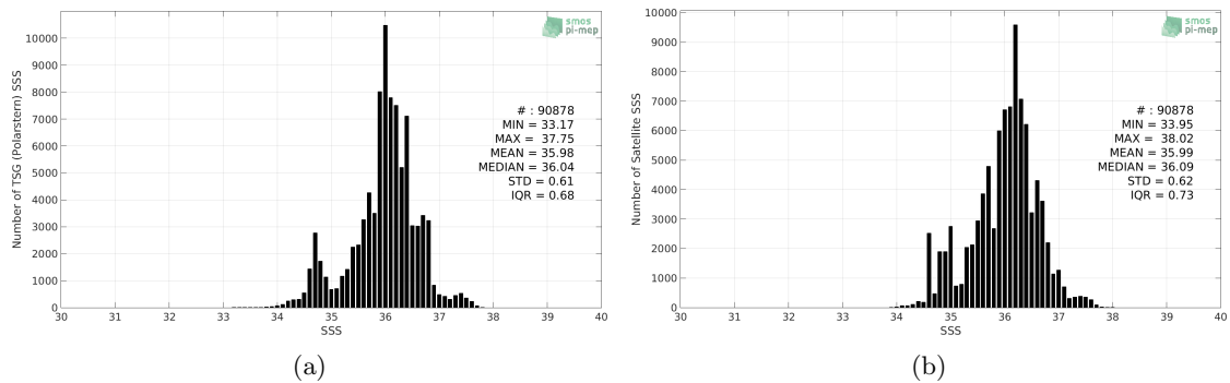
Figure 2: Histograms of SSS from TSG (Polarstern) (a) and SMOS SSS L3 v4 - 9 Days (CATDS-CECOS-LOCEAN) (b) considering all match-up pairs per bins of 0.1 over the Tropical Atlantic Ocean Pi-MEP region and for the full satellite product period.
