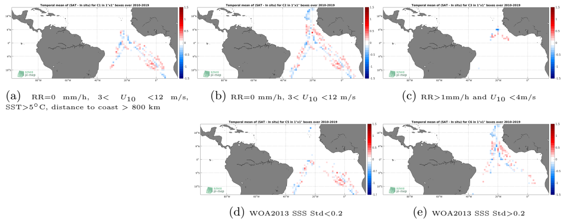
Figure 12: Temporal mean gridded over spatial boxes of size 1^{\circ}\times 1^{\circ} of \Delta\text{SSS} (SMOS-L3-CATDS-CECOS-LOCEAN-V4-9DAYS-25KM - TSG-POLARSTERN) for 5 different subdatasets corresponding to:RR=0 mm/h, 3 < U_{10} < 12 m/s, SST > 5^{\circ}\text{C} , distance to coast > 800 km (a), RR=0 mm/h, 3 < U_{10} < 12 m/s (b), RR > 1 mm/h and U_{10} < 4 m/s (c), WOA2013 SSS Std < 0.2 (d), WOA2013 SSS Std > 0.2 (e).
