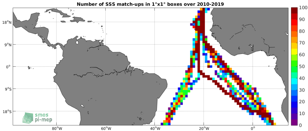
Figure 4: Number of SSS match-ups between TSG-POLARSTERN SSS and the SMOS-L3-CATDS-CECOS-LOCEAN-V4-9DAYS-25KM SSS product for the Tropical Atlantic Ocean Pi-MEP region over 1°x1° boxes and for the full satellite product period.
