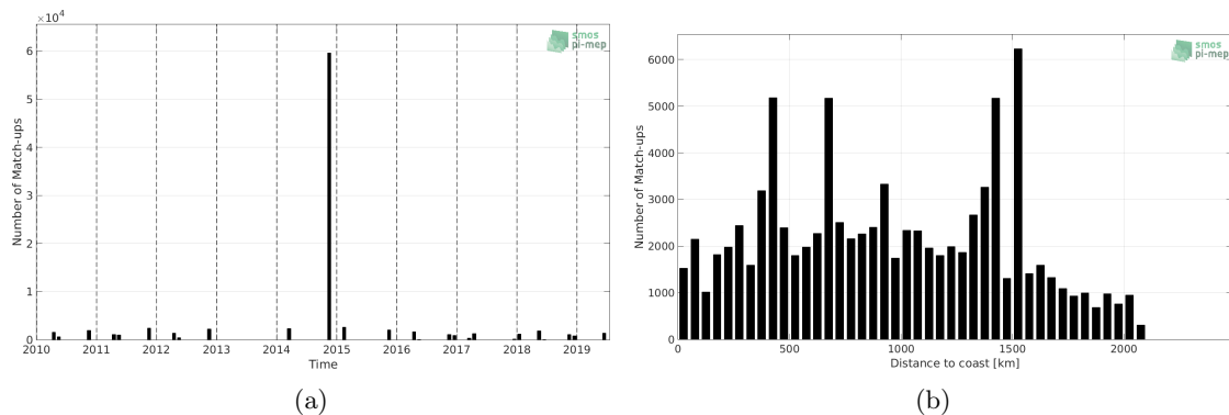
Figure 1: Number of match-ups between TSG-POLARSTERN and SMOS-L3-CATDS-CECOS-LOCEAN-V4-9DAYS-25KM SSS as a function of time (a) and as function of the distance to coast (b) over the Tropical Atlantic Ocean Pi-MEP region and for the full satellite product period.
