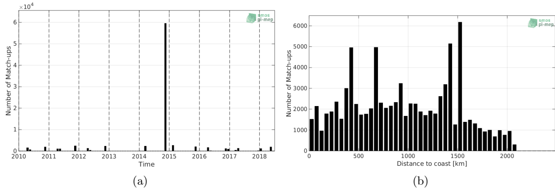
Figure 1: Number of match-ups between TSG-POLARSTERN and SMOS-L3-CATDS-CECOS-LOCEAN-V4-9DAYS-25KM SSS as a function of time (a) and as function of the distance to coast (b) over the Tropical Atlantic Ocean Pi-MEP region and for the full satellite product period.
