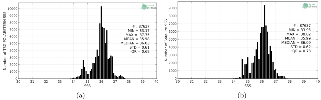
Figure 2: Histograms of SSS from TSG-POLARSTERN (a) and SMOS-L3-CATDS-CECOS-LOCEAN-V4-9DAYS-25KM (b) considering all match-up pairs per bins of 0.1 over the Tropical Atlantic Ocean Pi-MEP region and for the full satellite product period.
