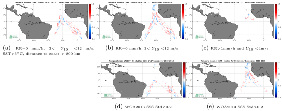
Figure 12: Temporal mean gridded over spatial boxes of size 1^\circ \times 1^\circ of \Delta SSS (SMOS-L3-CATDS-CECOS-LOCEAN-V4-9DAYS-25KM - TSG-POLARSTERN) for 5 different subdatasets corresponding to:RR=0 mm/h, 3 < U_{10} < 12 m/s, SST >5^\circ\text{C} , distance to coast > 800 km (a), RR=0 mm/h, 3 < U_{10} < 12 m/s (b), RR >1 mm/h and U_{10} < 4 m/s (c), WOA2013 SSS Std <0.2 (d), WOA2013 SSS Std >0.2 (e).
