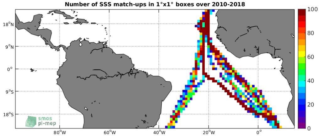
Figure 4: Number of SSS match-ups between TSG-POLARSTERN SSS and the SMOS-L3-CATDS-CECOS-LOCEAN-V4-9DAYS-25KM SSS product for the Tropical Atlantic Ocean Pi-MEP region over 1^\circ \times 1^\circ boxes and for the full satellite product period.
