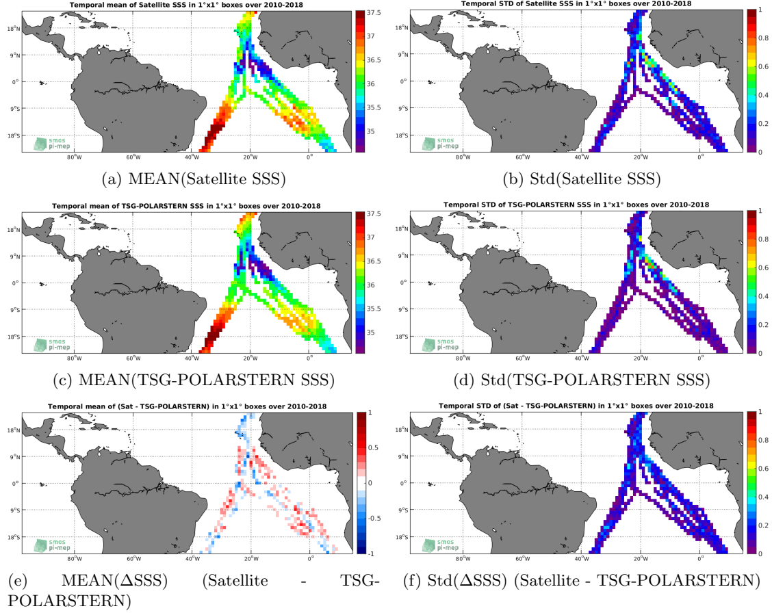
Figure 6: Temporal mean (left) and Std (right) of SSS from SMOS-L3-CATDS-CECOS-LOCEAN-V4-9DAYS-25KM (top), TSG-POLARSTERN (middle), and of \Delta SSS (Satellite - TSG-POLARSTERN). Only match-up pairs are used to generate these maps.
