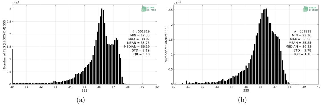
Figure 2: Histograms of SSS from TSG (LEGOS-DM) (a) and SMOS SSS L3 v4 - 9 Days (CATDS-CECOS-LOCEAN) (b) considering all match-up pairs per bins of 0.1 over the Tropical Atlantic Ocean Pi-MEP region and for the full satellite product period.
