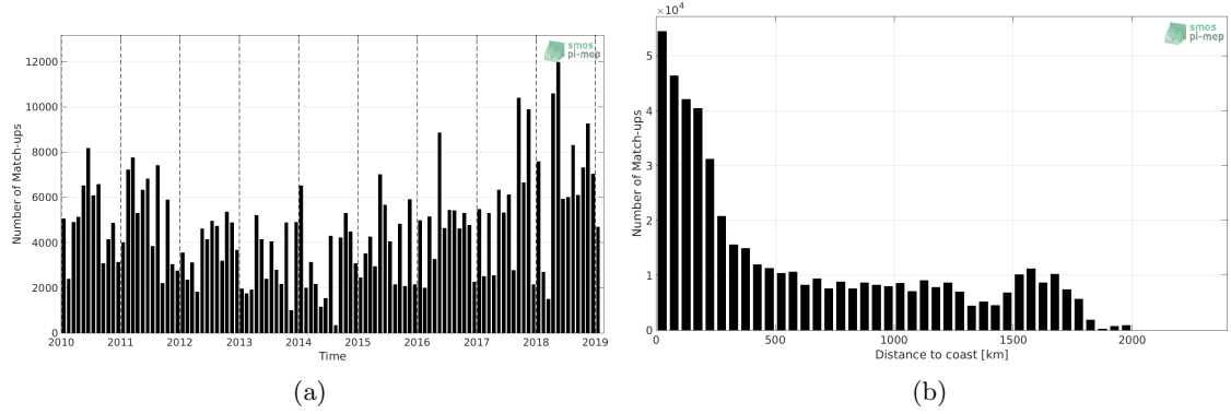
Figure 1: Number of match-ups between TSG (LEGOS-DM) and SMOS SSS L3 v4 - 9 Days (CATDS-CECOS-LOCEAN) SSS as a function of time (a) and as function of the distance to coast (b) over the Tropical Atlantic Ocean Pi-MEP region and for the full satellite product period.
