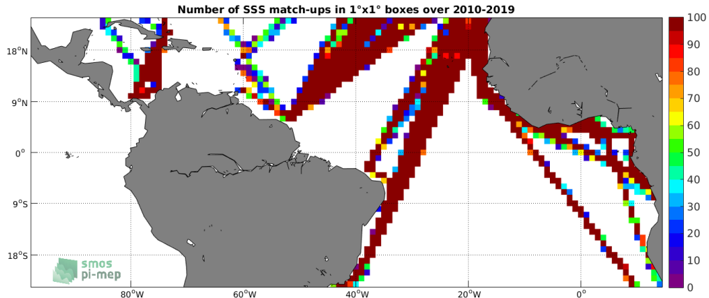
Figure 4: Number of SSS match-ups between TSG (LEGOS-DM) SSS and the SMOS SSS L3 v4 - 9 Days (CATDS-CECOS-LOCEAN) SSS product for the Tropical Atlantic Ocean Pi-MEP region over 1^\circ \times 1^\circ boxes and for the full satellite product period.
