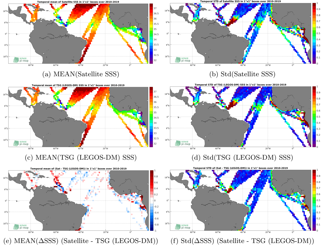
Figure 6: Temporal mean (left) and Std (right) of SSS from SMOS SSS L3 v4 - 9 Days (CATDS-CECOS-LOCEAN) (top), TSG (LEGOS-DM) (middle), and of \Delta SSS (Satellite - TSG (LEGOS-DM)). Only match-up pairs are used to generate these maps.
