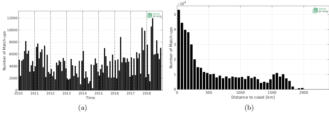
Figure 1: Number of match-ups between TSG-LEGOS-DM and SMOS-L3-CATDS-CECOS-LOCEAN-V4-9DAYS-25KM SSS as a function of time (a) and as function of the distance to coast (b) over the Tropical Atlantic Ocean Pi-MEP region and for the full satellite product period.
