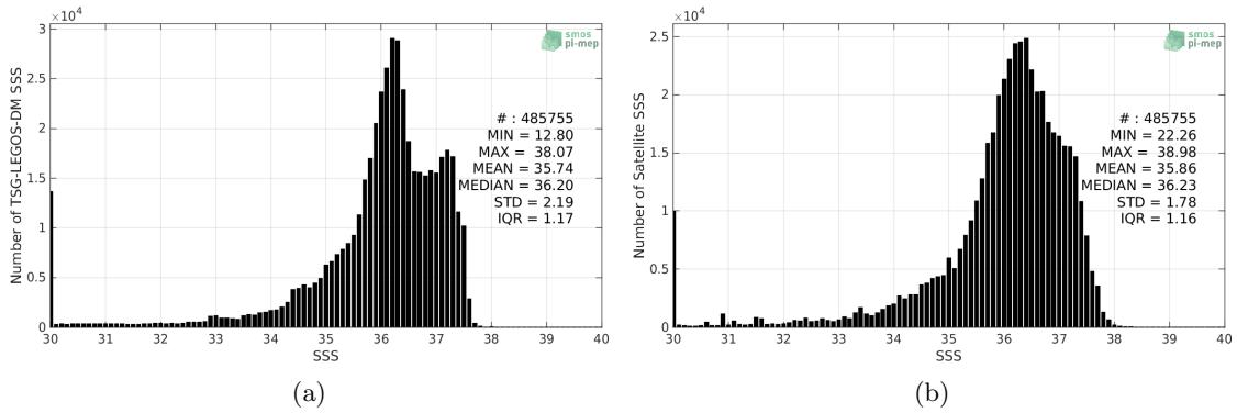
Figure 2: Histograms of SSS from TSG-LEGOS-DM (a) and SMOS-L3-CATDS-CECOS-LOCEAN-V4-9DAYS-25KM (b) considering all match-up pairs per bins of 0.1 over the Tropical Atlantic Ocean Pi-MEP region and for the full satellite product period.
