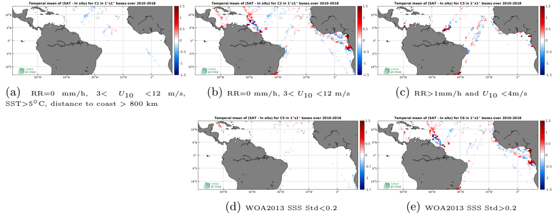
Figure 12: Temporal mean gridded over spatial boxes of size 1^\circ \times 1^\circ of \Delta SSS (SMOS-L3-CATDS-CECOS-LOCEAN-V4-9DAYS-25KM - TSG-LEGOS-DM) for 5 different subdatasets corresponding to:RR=0 mm/h, 3 < U_{10} < 12 m/s, SST >5^\circ\text{C} , distance to coast > 800 km (a), RR=0 mm/h, 3 < U_{10} < 12 m/s (b), RR >1 mm/h and U_{10} < 4 m/s (c), WOA2013 SSS Std <0.2 (d), WOA2013 SSS Std >0.2 (e).
