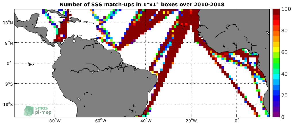
Figure 4: Number of SSS match-ups between TSG-LEGOS-DM SSS and the SMOS-L3-CATDS-CECOS-LOCEAN-V4-9DAYS-25KM SSS product for the Tropical Atlantic Ocean Pi-MEP region over 1^\circ \times 1^\circ boxes and for the full satellite product period.
