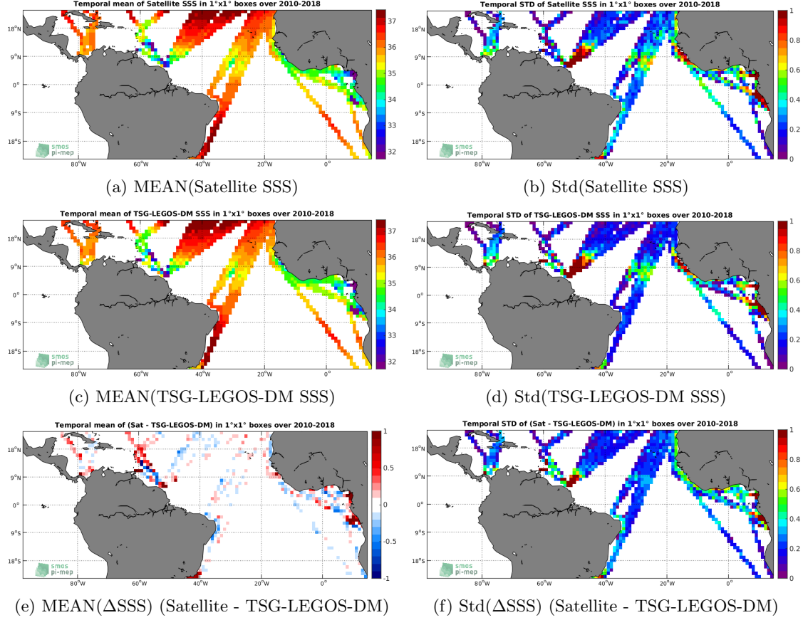
Figure 6: Temporal mean (left) and Std (right) of SSS from SMOS-L3-CATDS-CECOS-LOCEAN-V4-9DAYS-25KM (top), TSG-LEGOS-DM (middle), and of \Delta SSS (Satellite - TSG-LEGOS-DM). Only match-up pairs are used to generate these maps.
