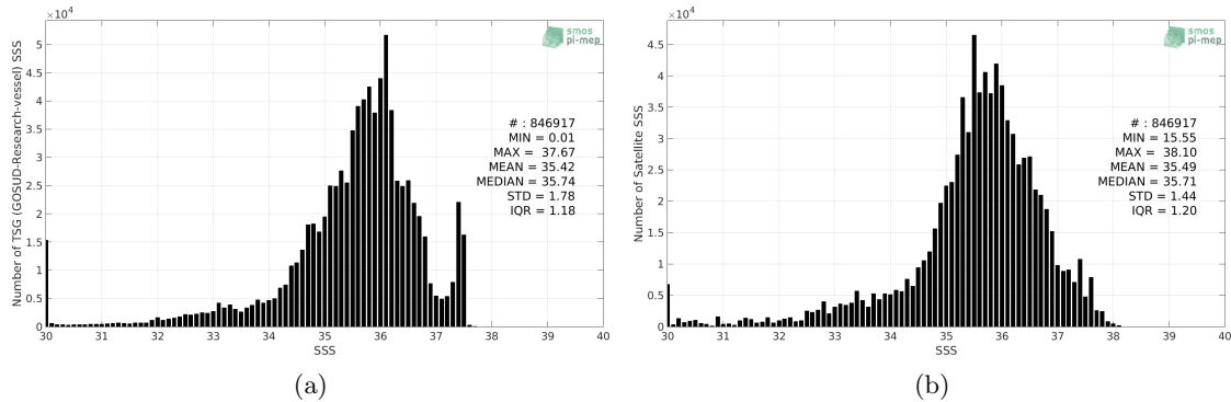
Figure 2: Histograms of SSS from TSG (GOSUD-Research-vessel) (a) and SMOS SSS L3 v4 - 9 Days (CATDS-CECOS-LOCEAN) (b) considering all match-up pairs per bins of 0.1 over the Tropical Atlantic Ocean Pi-MEP region and for the full satellite product period.
