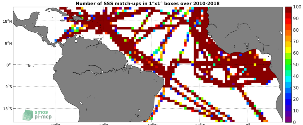
Figure 4: Number of SSS match-ups between TSG (GOSUD-Research-vessel) SSS and the SMOS SSS L3 v4 - 9 Days (CATDS-CECOS-LOCEAN) SSS product for the Tropical Atlantic Ocean Pi-MEP region over 1^\circ \times 1^\circ boxes and for the full satellite product period.
