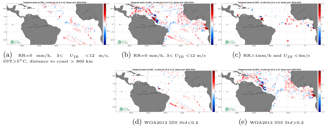
Figure 12: Temporal mean gridded over spatial boxes of size 1^\circ \times 1^\circ of \Delta SSS (SMOS SSS L3 v4 - 9 Days (CATDS-CECOS-LOCEAN) - TSG (GOSUD-Research-vessel)) for 5 different subdatasets corresponding to: RR=0 mm/h, 3 < U_{10} < 12 m/s, SST >5^\circ\text{C} , distance to coast > 800 km (a), RR=0 mm/h, 3 < U_{10} < 12 m/s (b), RR >1 mm/h and U_{10} < 4 m/s (c), WOA2013 SSS Std <0.2 (d), WOA2013 SSS Std >0.2 (e).
