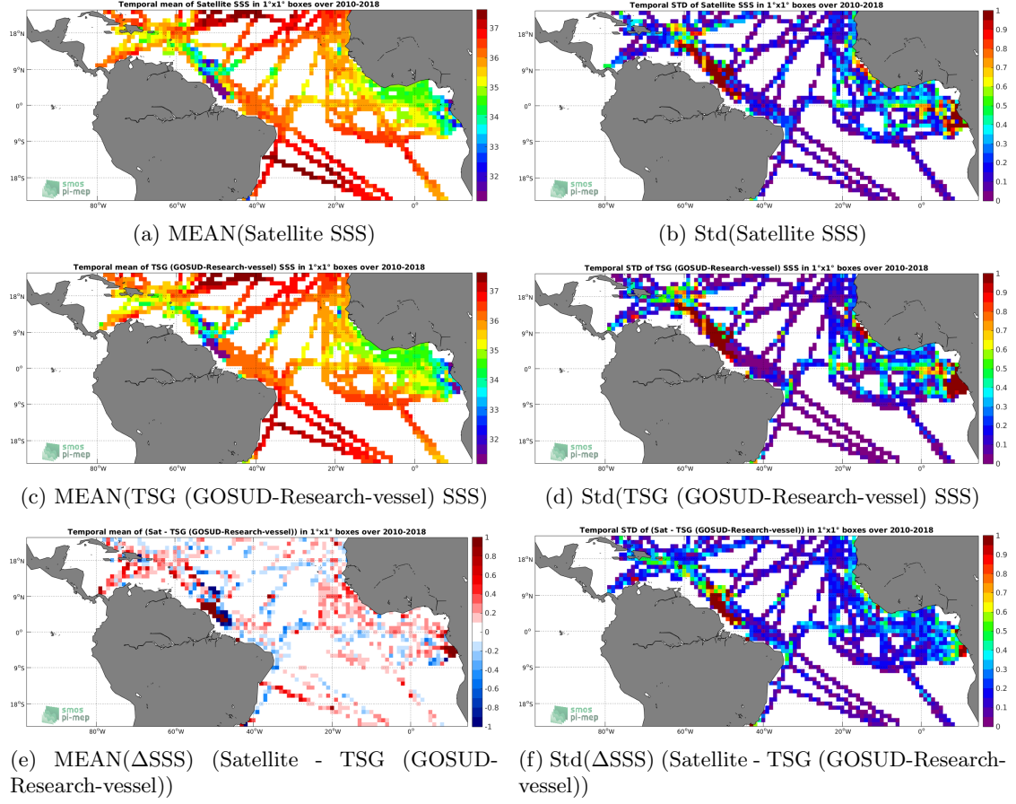
Figure 6: Temporal mean (left) and Std (right) of SSS from SMOS SSS L3 v4 - 9 Days (CATDS-CECOS-LOCEAN) (top), TSG (GOSUD-Research-vessel) (middle), and of \Delta SSS (Satellite - TSG (GOSUD-Research-vessel)). Only match-up pairs are used to generate these maps.
