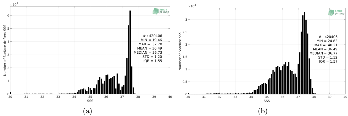
Figure 2: Histograms of SSS from Surface drifters (a) and SMOS SSS L3 v4 - 9 Days (CATDS-CECOS-LOCEAN) (b) considering all match-up pairs per bins of 0.1 over the Tropical Atlantic Ocean Pi-MEP region and for the full satellite product period.
