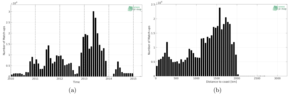
Figure 1: Number of match-ups between Surface drifters and SMOS SSS L3 v4 - 9 Days (CATDS-CECOS-LOCEAN) SSS as a function of time (a) and as function of the distance to coast (b) over the Tropical Atlantic Ocean Pi-MEP region and for the full satellite product period.
