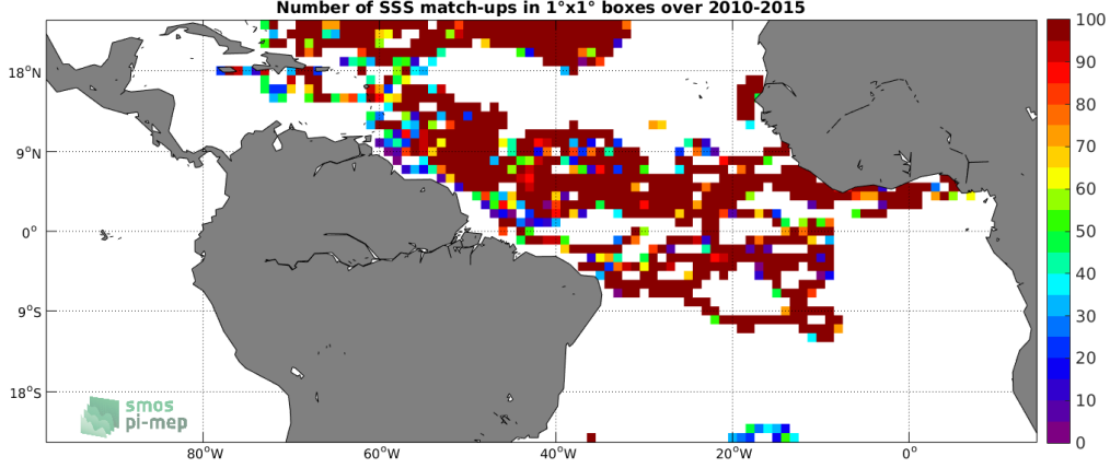
Figure 3: Number of SSS match-ups between Surface drifters SSS and the SMOS SSS L3 v4 - 9 Days (CATDS-CECOS-LOCEAN) SSS product for the Tropical Atlantic Ocean Pi-MEP region over 1°x1° boxes and for the full satellite product period.
