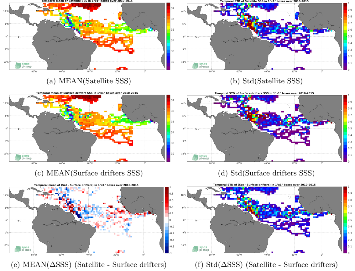
Figure 5: Temporal mean (left) and Std (right) of SSS from SMOS SSS L3 v4 - 9 Days (CATDS-CECOS-LOCEAN) (top), Surface drifters (middle), and of \Delta\text{SSS} (Satellite - Surface drifters). Only match-up pairs are used to generate these maps.
