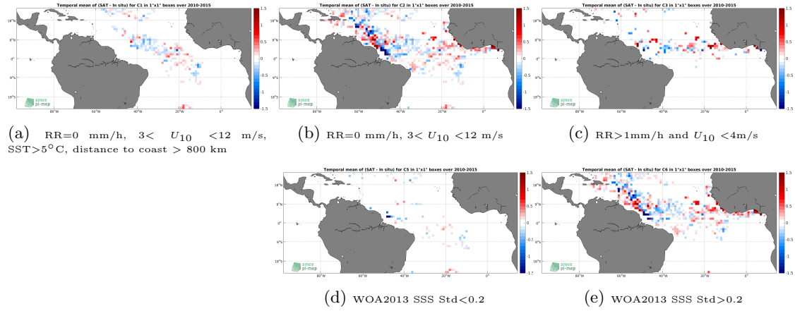
Figure 11: Temporal mean gridded over spatial boxes of size 1^{\circ}\times 1^{\circ} of \Delta\text{SSS} (SMOS-L3-CATDS-CECOS-LOCEAN-V4-9DAYS-25KM - Surface drifters) for 5 different subdatasets corresponding to:RR=0 mm/h, 3 < U_{10} < 12 m/s, SST >5^{\circ}\text{C} , distance to coast > 800 km (a), RR=0 mm/h, 3 < U_{10} < 12 m/s (b), RR >1 mm/h and U_{10} < 4 m/s (c), WOA2013 SSS Std <0.2 (d), WOA2013 SSS Std >0.2 (e).
