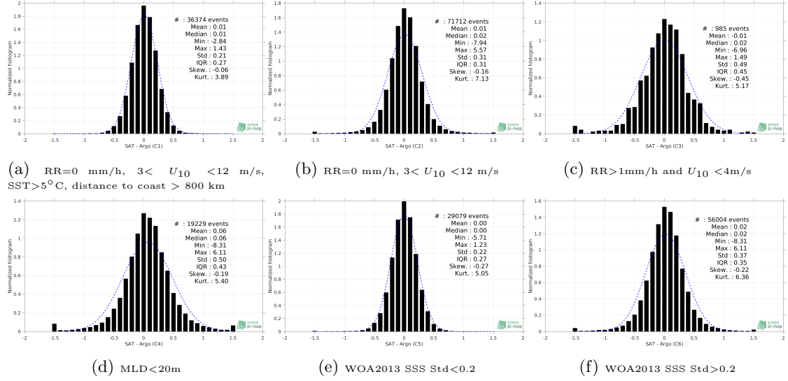
Figure 13: Normalized histogram of \Delta SSS (SMOS SSS L3 v4 - 9 Days (CATDS-CECOS-LOCEAN) - Argo) for 6 different subdatasets corresponding to: RR=0 mm/h, 3 < U_{10} < 12 m/s, SST>5°C, distance to coast > 800 km (a), RR=0 mm/h, 3 < U_{10} < 12 m/s (b), RR>1mm/h and U_{10} < 4 m/s (c), MLD<20m (d), WOA2013 SSS Std<0.2 (e), WOA2013 SSS Std>0.2 (f).
