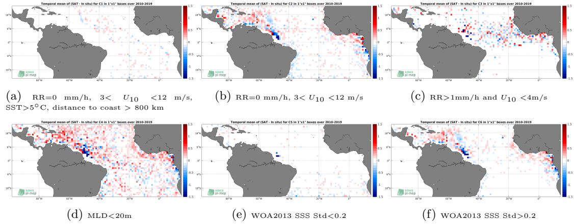
Figure 12: Temporal mean gridded over spatial boxes of size 1^\circ \times 1^\circ of \Delta SSS (SMOS SSS L3 v4 - 9 Days (CATDS-CECOS-LOCEAN) - Argo) for 6 different subdatasets corresponding to: RR=0 mm/h, 3 < U_{10} < 12 m/s, SST > 5^\circ C , distance to coast > 800 km (a), RR=0 mm/h, 3 < U_{10} < 12 m/s (b), RR > 1 mm/h and U_{10} < 4 m/s (c), MLD < 20 m (d), WOA2013 SSS Std < 0.2 (e), WOA2013 SSS Std > 0.2 (f).
