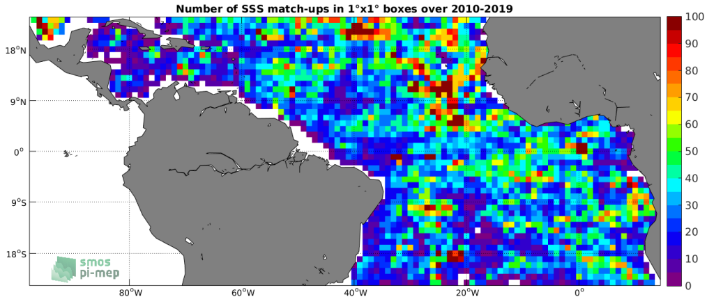
Figure 4: Number of SSS match-ups between Argo SSS and the SMOS SSS L3 v4 - 9 Days (CATDS-CECOS-LOCEAN) SSS product for the Tropical Atlantic Ocean Pi-MEP region over 1^\circ \times 1^\circ boxes and for the full satellite product period.
