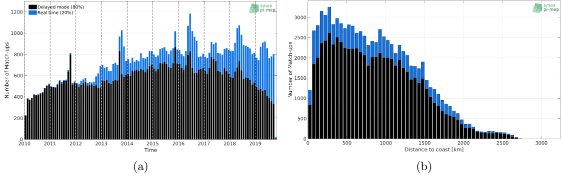
Figure 1: Number of match-ups between Argo and SMOS SSS L3 v4 - 9 Days (CATDS-CECOS-LOCEAN) SSS as a function of time (a) and as function of the distance to coast (b) over the Tropical Atlantic Ocean Pi-MEP region and for the full satellite product period.
