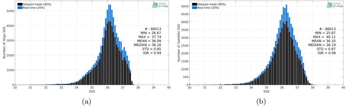
Figure 2: Histograms of SSS from Argo (a) and SMOS SSS L3 v4 - 9 Days (CATDS-CECOS-LOCEAN) (b) considering all match-up pairs per bins of 0.1 over the Tropical Atlantic Ocean Pi-MEP region and for the full satellite product period.
