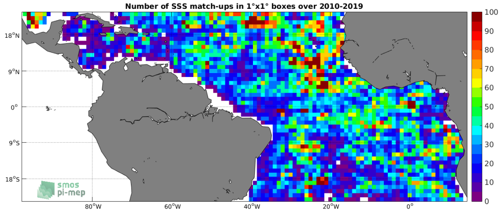
Figure 4: Number of SSS match-ups between Argo SSS and the SMOS-L3-CATDS-CECOS-LOCEAN-V4-9DAYS-25KM SSS product for the Tropical Atlantic Ocean Pi-MEP region over 1°x1° boxes and for the full satellite product period.
