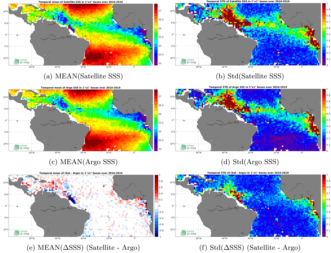
Figure 6: Temporal mean (left) and Std (right) of SSS from SMOS-L3-CATDS-CECOS-LOCEAN-V4-9DAYS-25KM (top), Argo (middle), and of \Delta SSS (Satellite - Argo). Only match-up pairs are used to generate these maps.
