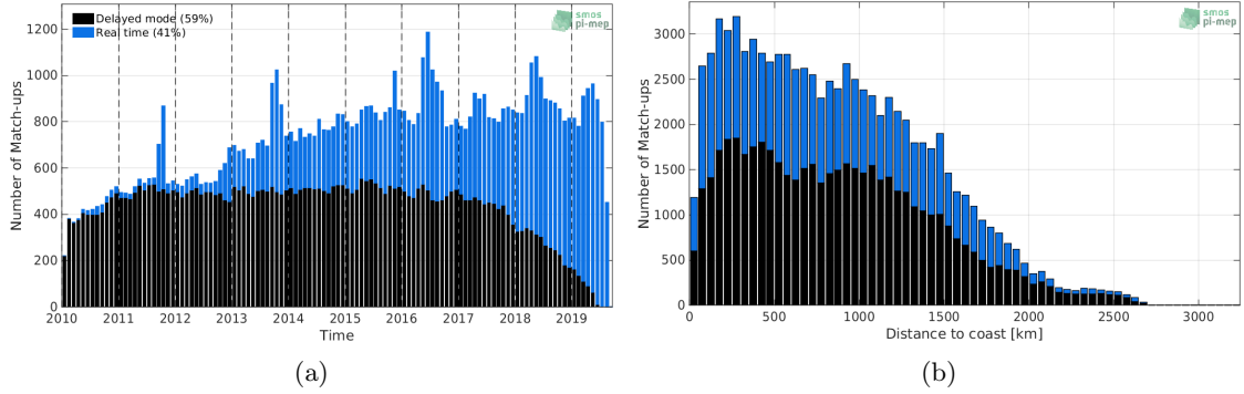
Figure 1: Number of match-ups between Argo and SMOS-L3-CATDS-CECOS-LOCEAN-V4-9DAYS-25KM SSS as a function of time (a) and as function of the distance to coast (b) over the Tropical Atlantic Ocean Pi-MEP region and for the full satellite product period.
