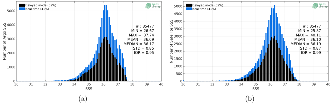
Figure 2: Histograms of SSS from Argo (a) and SMOS-L3-CATDS-CECOS-LOCEAN-V4-9DAYS-25KM (b) considering all match-up pairs per bins of 0.1 over the Tropical Atlantic Ocean Pi-MEP region and for the full satellite product period.
