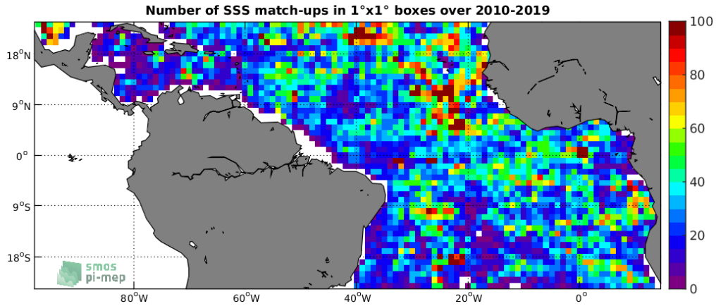
Figure 4: Number of SSS match-ups between Argo SSS and the SMOS-L3-CATDS-CECOS-LOCEAN-V4-9DAYS-25KM SSS product for the Tropical Atlantic Ocean Pi-MEP region over 1^\circ \times 1^\circ boxes and for the full satellite product period.
