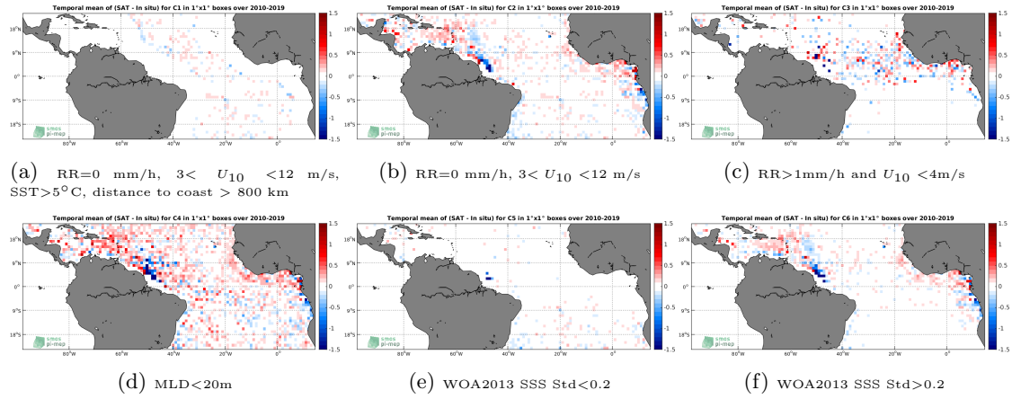
Figure 12: Temporal mean gridded over spatial boxes of size 1^\circ \times 1^\circ of \Delta SSS (SMOS-L3-CATDS-CECOS-LOCEAN-V4-9DAYS-25KM - Argo) for 6 different subdatasets corresponding to:RR=0 mm/h, 3 < U_{10} < 12 m/s, SST>5°C, distance to coast > 800 km (a), RR=0 mm/h, 3 < U_{10} < 12 m/s (b), RR>1mm/h and U_{10} < 4 m/s (c),MLD<20m (d),WOA2013 SSS Std<0.2 (e),WOA2013 SSS Std>0.2 (f).
