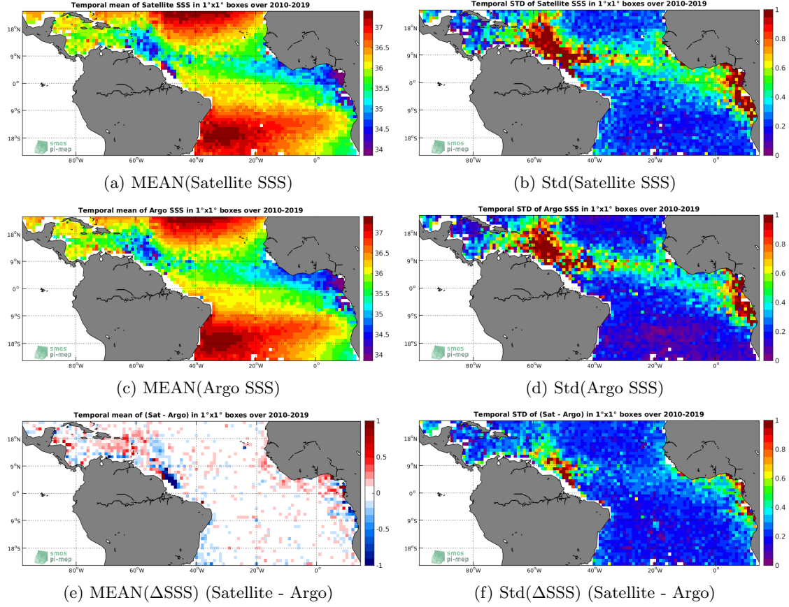
Figure 6: Temporal mean (left) and Std (right) of SSS from SMOS-L3-CATDS-CECOS-LOCEAN-V4-9DAYS-25KM (top), Argo (middle), and of ΔSSS (Satellite - Argo). Only match-up pairs are used to generate these maps.
