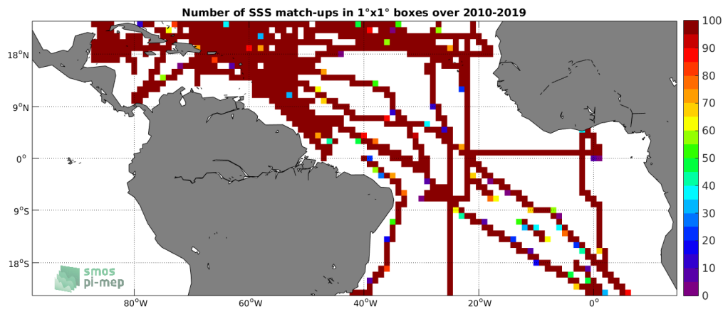
Figure 4: Number of SSS match-ups between TSG-SAMOS SSS and the SMOS-L3-CATDS-CECOS-LOCEAN-V4-18DAYS-25KM SSS product for the Tropical Atlantic Ocean Pi-MEP region over 1^\circ \times 1^\circ boxes and for the full satellite product period.
