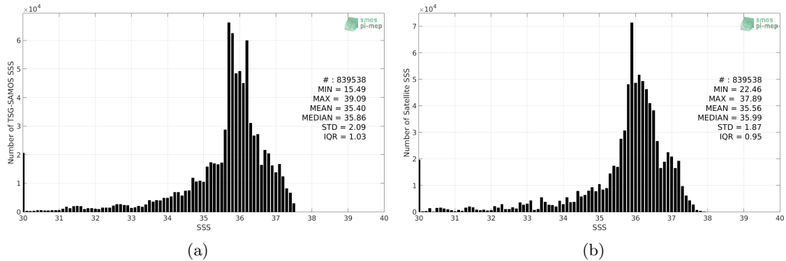
Figure 2: Histograms of SSS from TSG-SAMOS (a) and SMOS-L3-CATDS-CECOS-LOCEAN-V4-18DAYS-25KM (b) considering all match-up pairs per bins of 0.1 over the Tropical Atlantic Ocean Pi-MEP region and for the full satellite product period.
