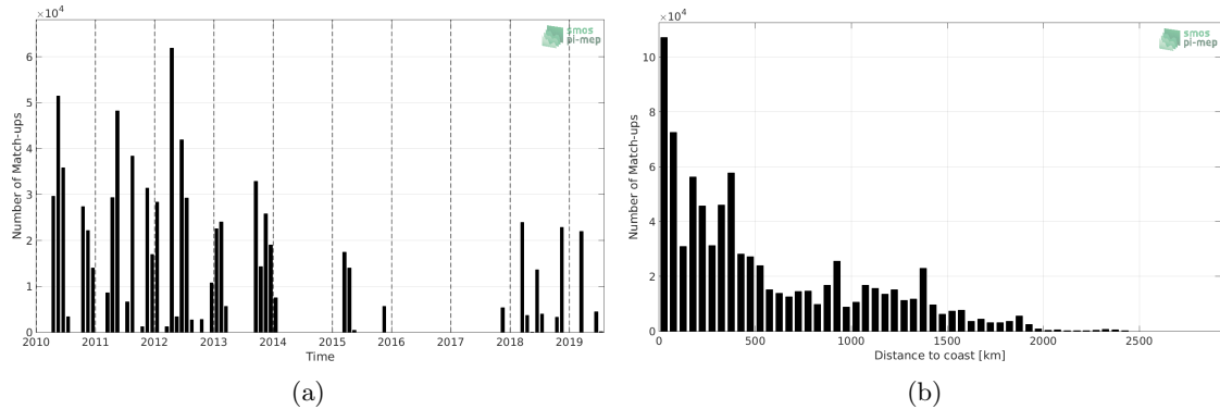
Figure 1: Number of match-ups between TSG-SAMOS and SMOS-L3-CATDS-CECOS-LOCEAN-V4-18DAYS-25KM SSS as a function of time (a) and as function of the distance to coast (b) over the Tropical Atlantic Ocean Pi-MEP region and for the full satellite product period.
