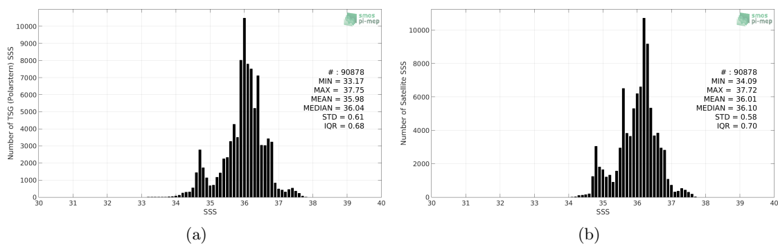
Figure 2: Histograms of SSS from TSG (Polarstern) (a) and SMOS SSS L3 v4 - 18 Days (CATDS-CECOS-LOCEAN) (b) considering all match-up pairs per bins of 0.1 over the Tropical Atlantic Ocean Pi-MEP region and for the full satellite product period.
