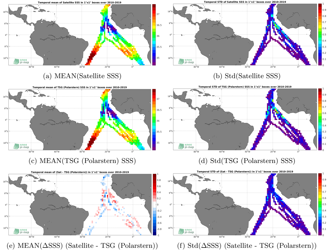
Figure 6: Temporal mean (left) and Std (right) of SSS from SMOS SSS L3 v4 - 18 Days (CATDS-CECOS-LOCEAN) (top), TSG (Polarstern) (middle), and of \Delta SSS (Satellite - TSG (Polarstern)). Only match-up pairs are used to generate these maps.
