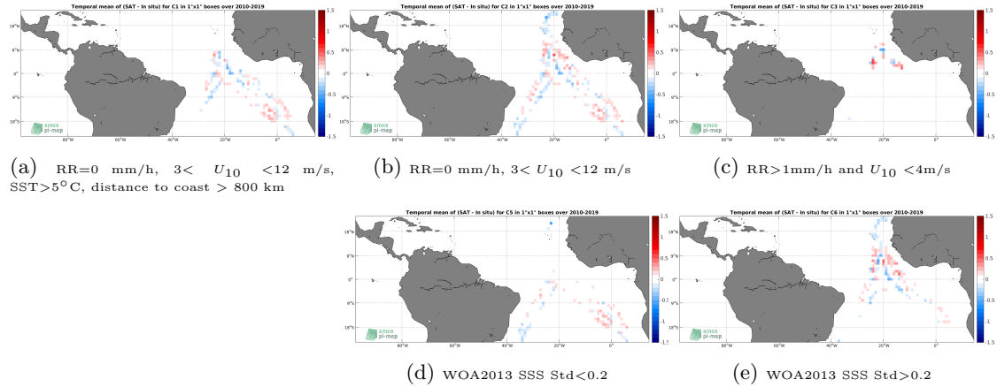
Figure 12: Temporal mean gridded over spatial boxes of size 1^{\circ}\times 1^{\circ} of \Delta\text{SSS} (SMOS SSS L3 v4 - 18 Days (CATDS-CECOS-LOCEAN) - TSG (Polarstern)) for 5 different subdatasets corresponding to:RR=0 mm/h, 3 < U_{10} < 12 m/s, SST >5^{\circ}\text{C} , distance to coast > 800 km (a), RR=0 mm/h, 3 < U_{10} < 12 m/s (b), RR >1 mm/h and U_{10} < 4 m/s (c), WOA2013 SSS Std <0.2 (d), WOA2013 SSS Std >0.2 (e).
