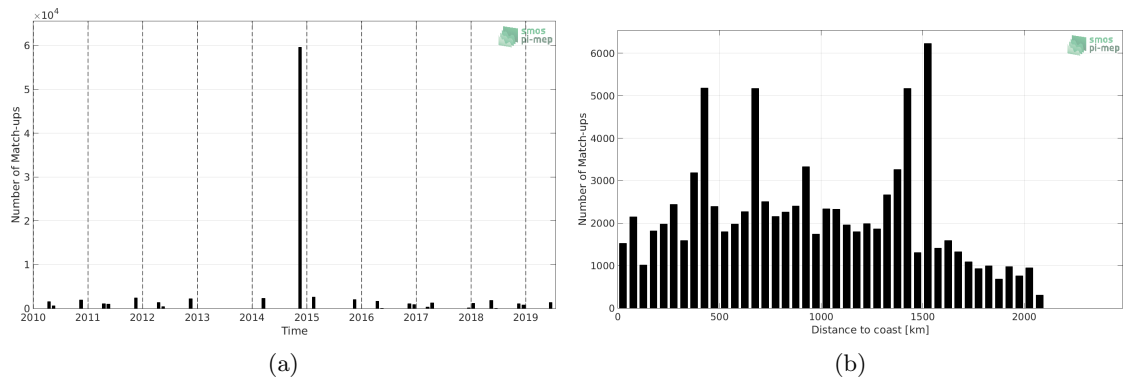
Figure 1: Number of match-ups between TSG (Polarstern) and SMOS SSS L3 v4 - 18 Days (CATDS-CECOS-LOCEAN) SSS as a function of time (a) and as function of the distance to coast (b) over the Tropical Atlantic Ocean Pi-MEP region and for the full satellite product period.
