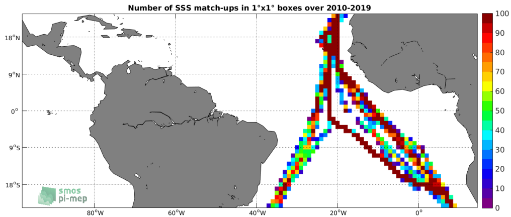
Figure 4: Number of SSS match-ups between TSG (Polarstern) SSS and the SMOS SSS L3 v4 - 18 Days (CATDS-CECOS-LOCEAN) SSS product for the Tropical Atlantic Ocean Pi-MEP region over 1^\circ \times 1^\circ boxes and for the full satellite product period.
