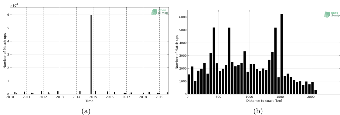
Figure 1: Number of match-ups between TSG-POLARSTERN and SMOS-L3-CATDS-CECOS-LOCEAN-V4-18DAYS-25KM SSS as a function of time (a) and as function of the distance to coast (b) over the Tropical Atlantic Ocean Pi-MEP region and for the full satellite product period.
