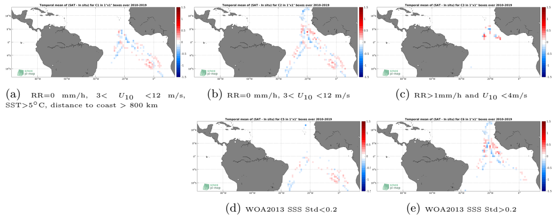
Figure 12: Temporal mean gridded over spatial boxes of size 1^{\circ}\times 1^{\circ} of \Delta\text{SSS} (SMOS-L3-CATDS-CECOS-LOCEAN-V4-18DAYS-25KM - TSG-POLARSTERN) for 5 different subdatasets corresponding to: \text{RR}=0 mm/h, 3 < U_{10} < 12 m/s, \text{SST} > 5^{\circ}\text{C} , distance to coast > 800 km (a), \text{RR}=0 mm/h, 3 < U_{10} < 12 m/s (b), \text{RR} > 1\text{mm/h} and U_{10} < 4\text{m/s} (c), WOA2013 SSS Std < 0.2 (d), WOA2013 SSS Std > 0.2 (e).
