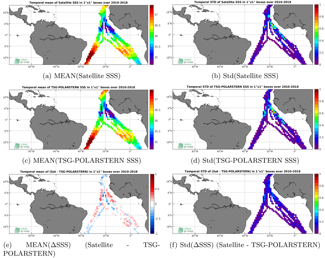
Figure 6: Temporal mean (left) and Std (right) of SSS from SMOS-L3-CATDS-CECOS-LOCEAN-V4-18DAYS-25KM (top), TSG-POLARSTERN (middle), and of \Delta SSS (Satellite - TSG-POLARSTERN). Only match-up pairs are used to generate these maps.
