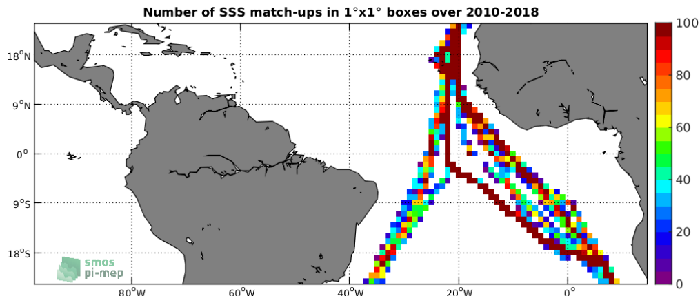
Figure 4: Number of SSS match-ups between TSG-POLARSTERN SSS and the SMOS-L3-CATDS-CECOS-LOCEAN-V4-18DAYS-25KM SSS product for the Tropical Atlantic Ocean Pi-MEP region over 1^\circ \times 1^\circ boxes and for the full satellite product period.
