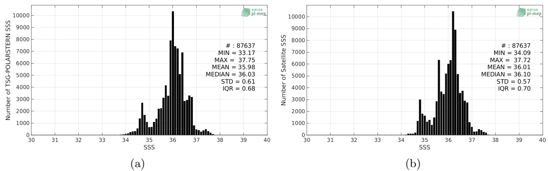
Figure 2: Histograms of SSS from TSG-POLARSTERN (a) and SMOS-L3-CATDS-CECOS-LOCEAN-V4-18DAYS-25KM (b) considering all match-up pairs per bins of 0.1 over the Tropical Atlantic Ocean Pi-MEP region and for the full satellite product period.
