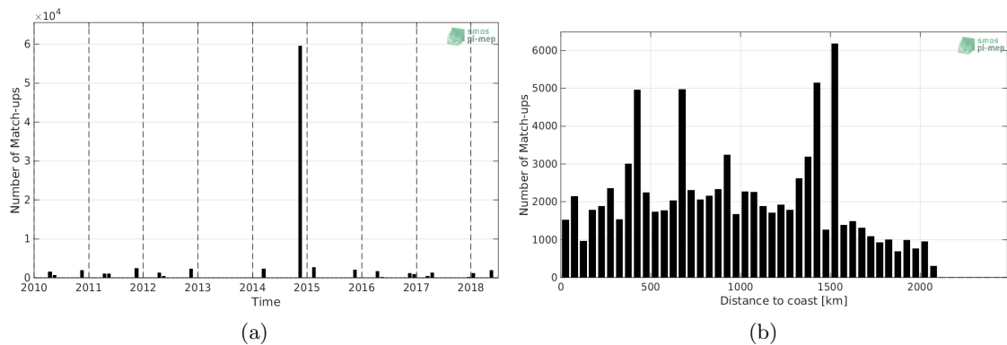
Figure 1: Number of match-ups between TSG-POLARSTERN and SMOS-L3-CATDS-CECOS-LOCEAN-V4-18DAYS-25KM SSS as a function of time (a) and as function of the distance to coast (b) over the Tropical Atlantic Ocean Pi-MEP region and for the full satellite product period.
