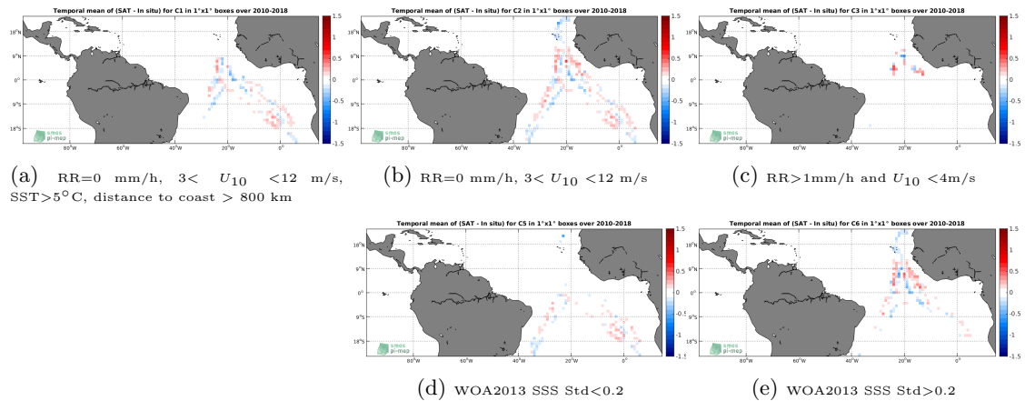
Figure 12: Temporal mean gridded over spatial boxes of size 1^\circ \times 1^\circ of \Delta SSS (SMOS-L3-CATDS-CECOS-LOCEAN-V4-18DAYS-25KM - TSG-POLARSTERN) for 5 different subdatasets corresponding to:RR=0 mm/h, 3 < U_{10} < 12 m/s, SST >5^\circ\text{C} , distance to coast > 800 km (a), RR=0 mm/h, 3 < U_{10} < 12 m/s (b), RR >1 mm/h and U_{10} < 4 m/s (c), WOA2013 SSS Std <0.2 (d), WOA2013 SSS Std >0.2 (e).
