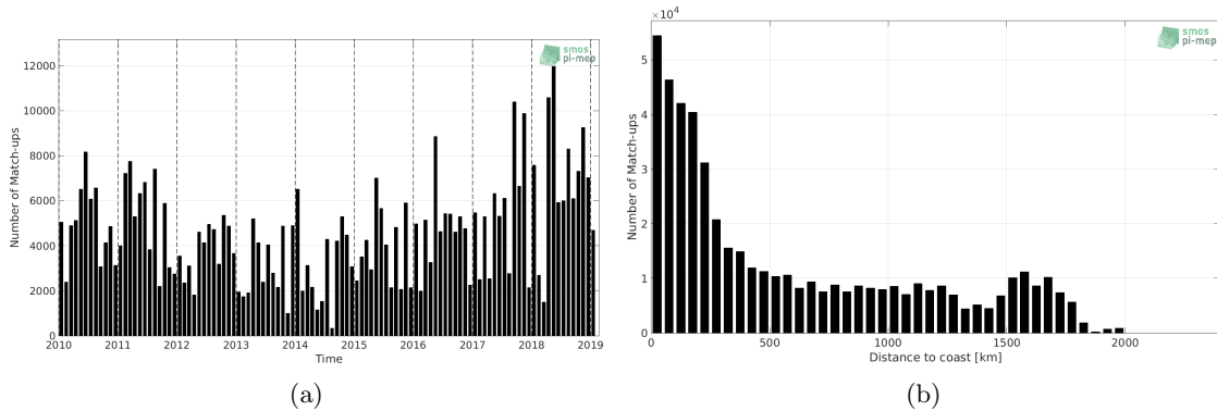
Figure 1: Number of match-ups between TSG (LEGOS-DM) and SMOS SSS L3 v4 - 18 Days (CATDS-CECOS-LOCEAN) SSS as a function of time (a) and as function of the distance to coast (b) over the Tropical Atlantic Ocean Pi-MEP region and for the full satellite product period.
