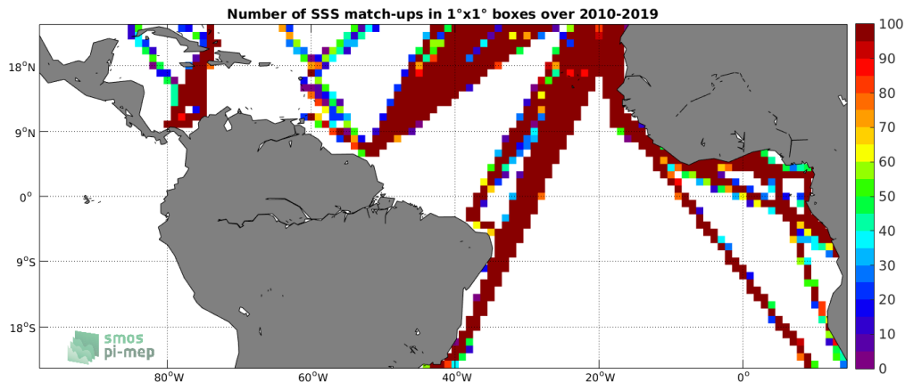
Figure 4: Number of SSS match-ups between TSG (LEGOS-DM) SSS and the SMOS SSS L3 v4 - 18 Days (CATDS-CECOS-LOCEAN) SSS product for the Tropical Atlantic Ocean Pi-MEP region over 1^\circ \times 1^\circ boxes and for the full satellite product period.
