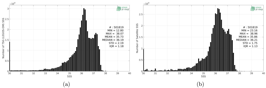
Figure 2: Histograms of SSS from TSG (LEGOS-DM) (a) and SMOS SSS L3 v4 - 18 Days (CATDS-CECOS-LOCEAN) (b) considering all match-up pairs per bins of 0.1 over the Tropical Atlantic Ocean Pi-MEP region and for the full satellite product period.
