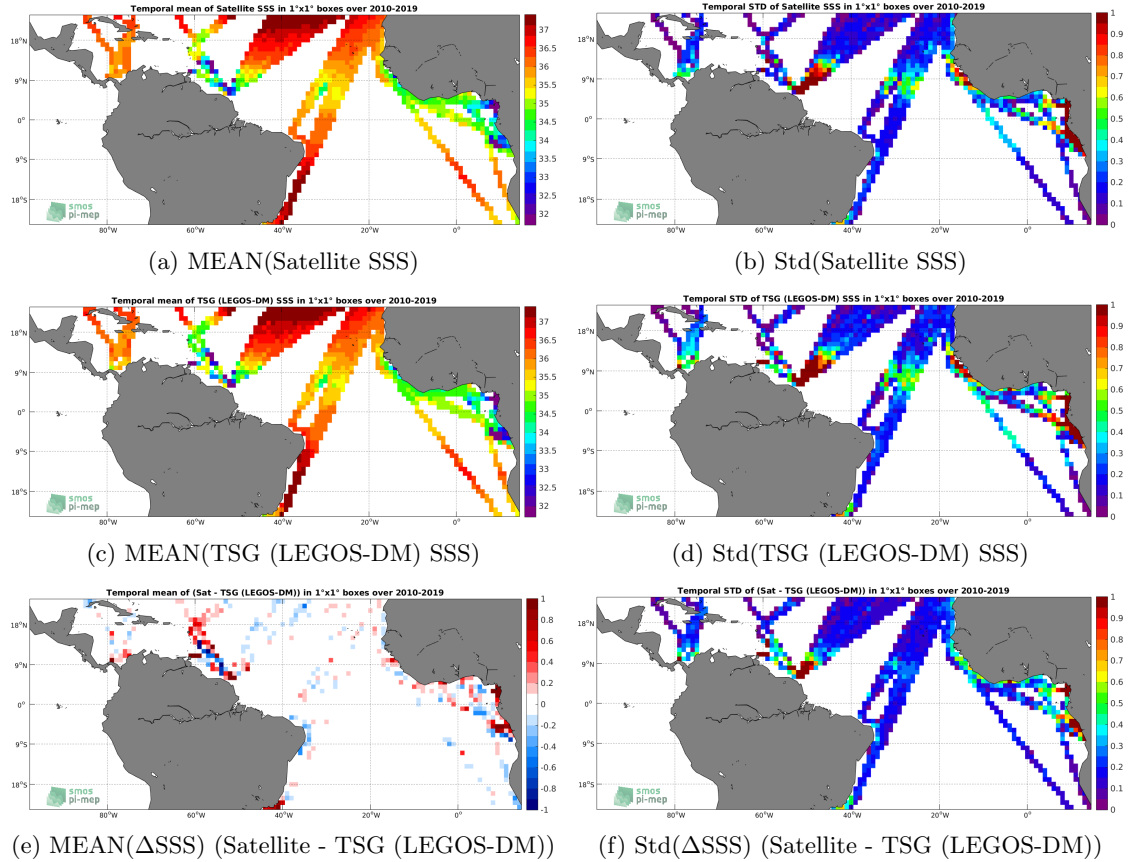
Figure 6: Temporal mean (left) and Std (right) of SSS from SMOS SSS L3 v4 - 18 Days (CATDS-CECOS-LOCEAN) (top), TSG (LEGOS-DM) (middle), and of \Delta SSS (Satellite - TSG (LEGOS-DM)). Only match-up pairs are used to generate these maps.
