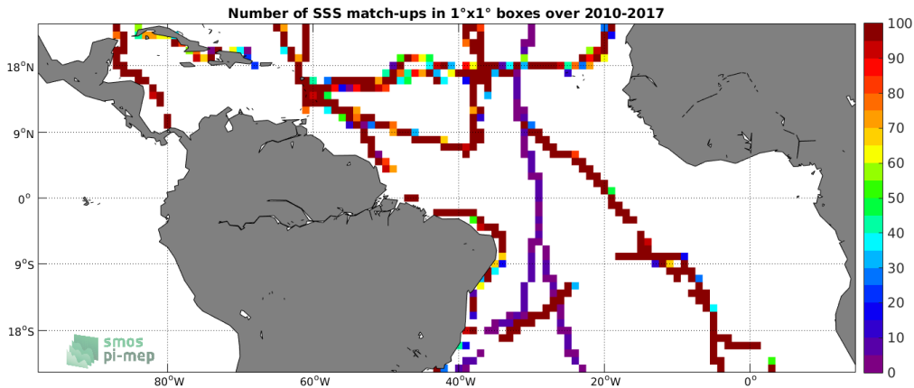
Figure 4: Number of SSS match-ups between TSG (GOSUD-Sailing-ship) SSS and the SMOS SSS L3 v4 - 18 Days (CATDS-CECOS-LOCEAN) SSS product for the Tropical Atlantic Ocean Pi-MEP region over 1^\circ \times 1^\circ boxes and for the full satellite product period.
