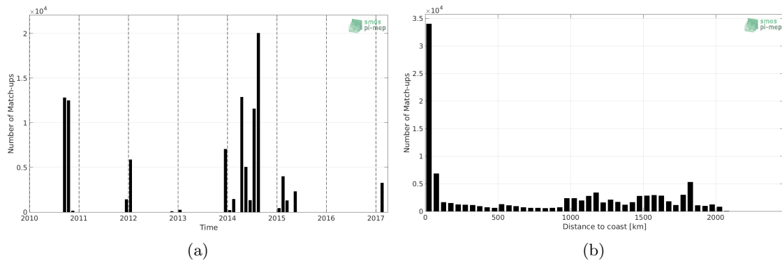
Figure 1: Number of match-ups between TSG (GOSUD-Sailing-ship) and SMOS SSS L3 v4 - 18 Days (CATDS-CECOS-LOCEAN) SSS as a function of time (a) and as function of the distance to coast (b) over the Tropical Atlantic Ocean Pi-MEP region and for the full satellite product period.
