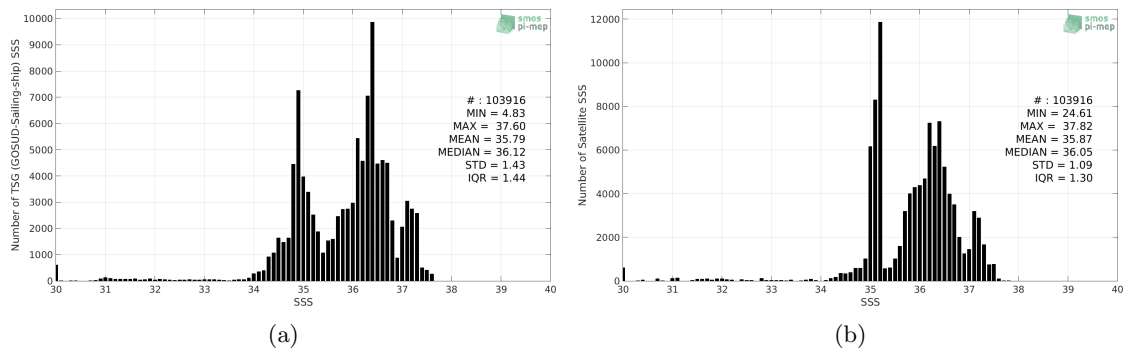
Figure 2: Histograms of SSS from TSG (GOSUD-Sailing-ship) (a) and SMOS SSS L3 v4 - 18 Days (CATDS-CECOS-LOCEAN) (b) considering all match-up pairs per bins of 0.1 over the Tropical Atlantic Ocean Pi-MEP region and for the full satellite product period.
