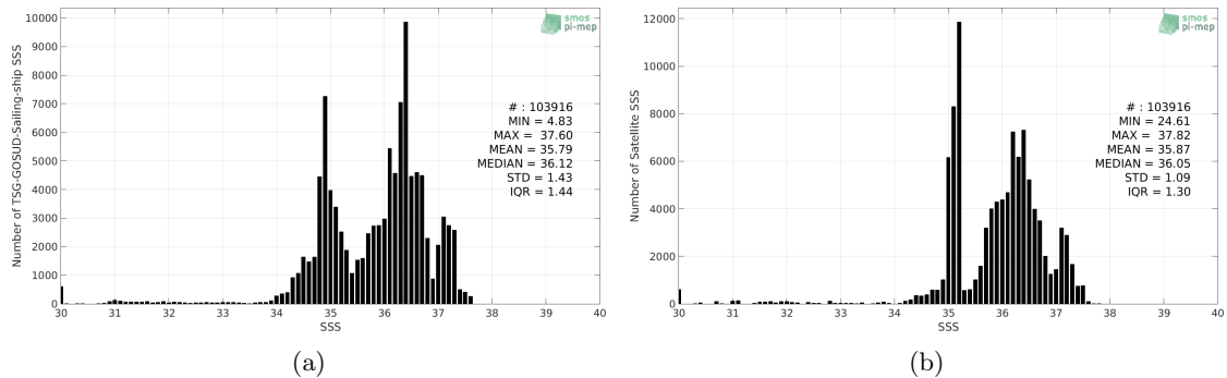
Figure 2: Histograms of SSS from TSG-GOSUD-Sailing-ship (a) and SMOS-L3-CATDS-CECOS-LOCEAN-V4-18DAYS-25KM (b) considering all match-up pairs per bins of 0.1 over the Tropical Atlantic Ocean Pi-MEP region and for the full satellite product period.
