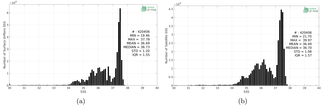
Figure 2: Histograms of SSS from Surface drifters (a) and SMOS SSS L3 v4 - 18 Days (CATDS-CECOS-LOCEAN) (b) considering all match-up pairs per bins of 0.1 over the Tropical Atlantic Ocean Pi-MEP region and for the full satellite product period.
