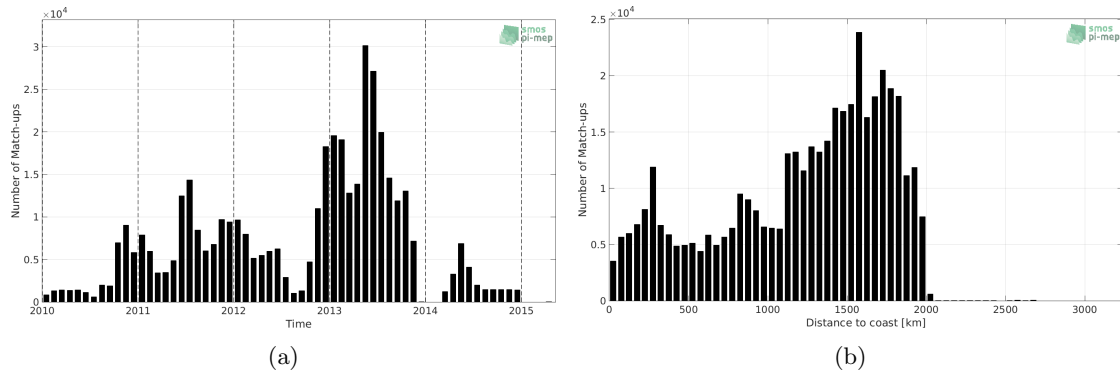
Figure 1: Number of match-ups between Surface drifters and SMOS SSS L3 v4 - 18 Days (CATDS-CECOS-LOCEAN) SSS as a function of time (a) and as function of the distance to coast (b) over the Tropical Atlantic Ocean Pi-MEP region and for the full satellite product period.
