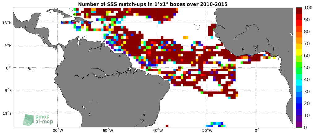
Figure 3: Number of SSS match-ups between Surface drifters SSS and the SMOS SSS L3 v4 - 18 Days (CATDS-CECOS-LOCEAN) SSS product for the Tropical Atlantic Ocean Pi-MEP region over 1^\circ \times 1^\circ boxes and for the full satellite product period.
