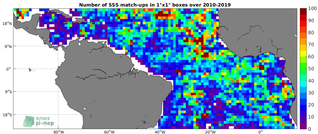
Figure 4: Number of SSS match-ups between Argo SSS and the SMOS SSS L3 v4 - 18 Days (CATDS-CECOS-LOCEAN) SSS product for the Tropical Atlantic Ocean Pi-MEP region over 1^\circ \times 1^\circ boxes and for the full satellite product period.
