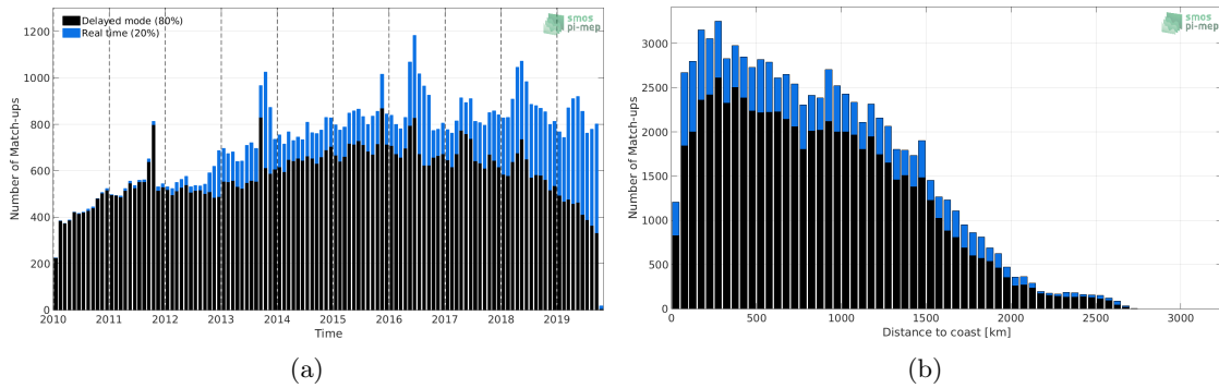
Figure 1: Number of match-ups between Argo and SMOS SSS L3 v4 - 18 Days (CATDS-CECOS-LOCEAN) SSS as a function of time (a) and as function of the distance to coast (b) over the Tropical Atlantic Ocean Pi-MEP region and for the full satellite product period.
