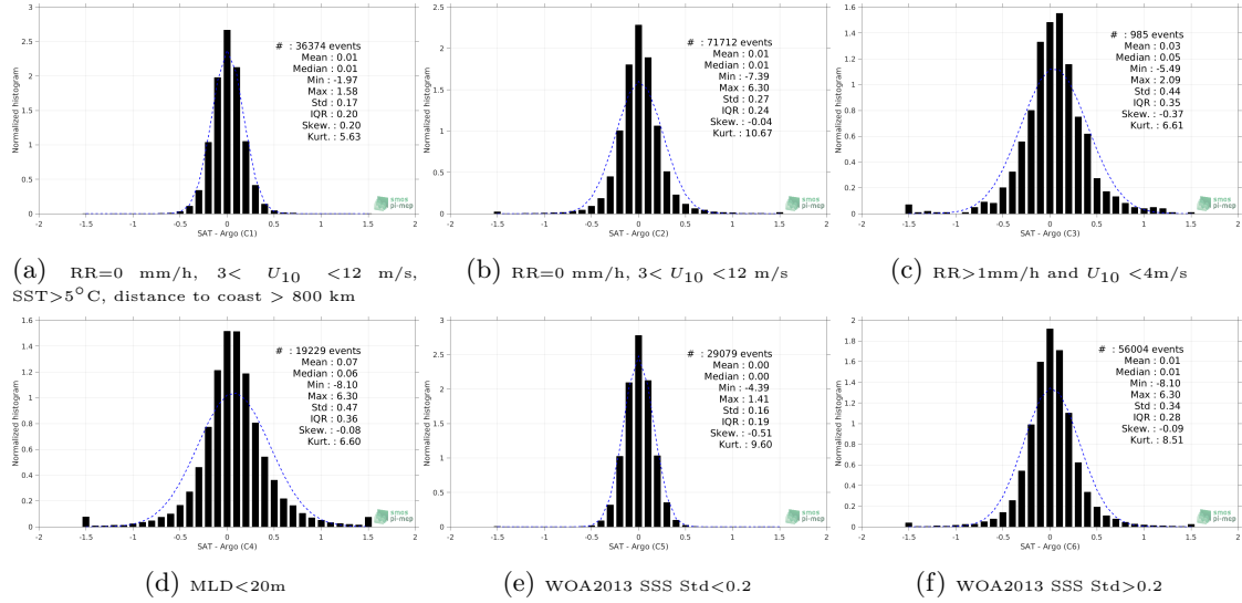
Figure 13: Normalized histogram of \Delta\text{SSS} (SMOS SSS L3 v4 - 18 Days (CATDS-CECOS-LOCEAN) - Argo) for 6 different subdatasets corresponding to: RR=0 mm/h, 3 < U_{10} < 12 m/s, SST>5°C, distance to coast > 800 km (a), RR=0 mm/h, 3 < U_{10} < 12 m/s (b), RR>1mm/h and U_{10} < 4 m/s (c), MLD<20m (d), WOA2013 SSS Std<0.2 (e), WOA2013 SSS Std>0.2 (f).
