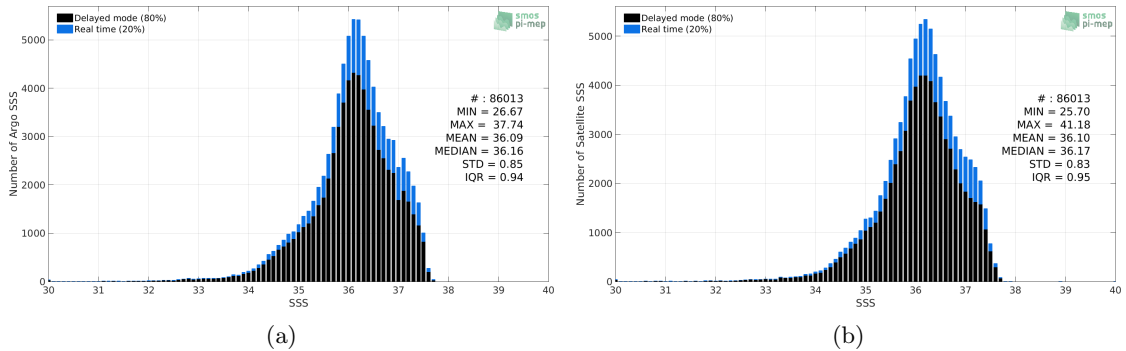
Figure 2: Histograms of SSS from Argo (a) and SMOS SSS L3 v4 - 18 Days (CATDS-CECOS-LOCEAN) (b) considering all match-up pairs per bins of 0.1 over the Tropical Atlantic Ocean Pi-MEP region and for the full satellite product period.
