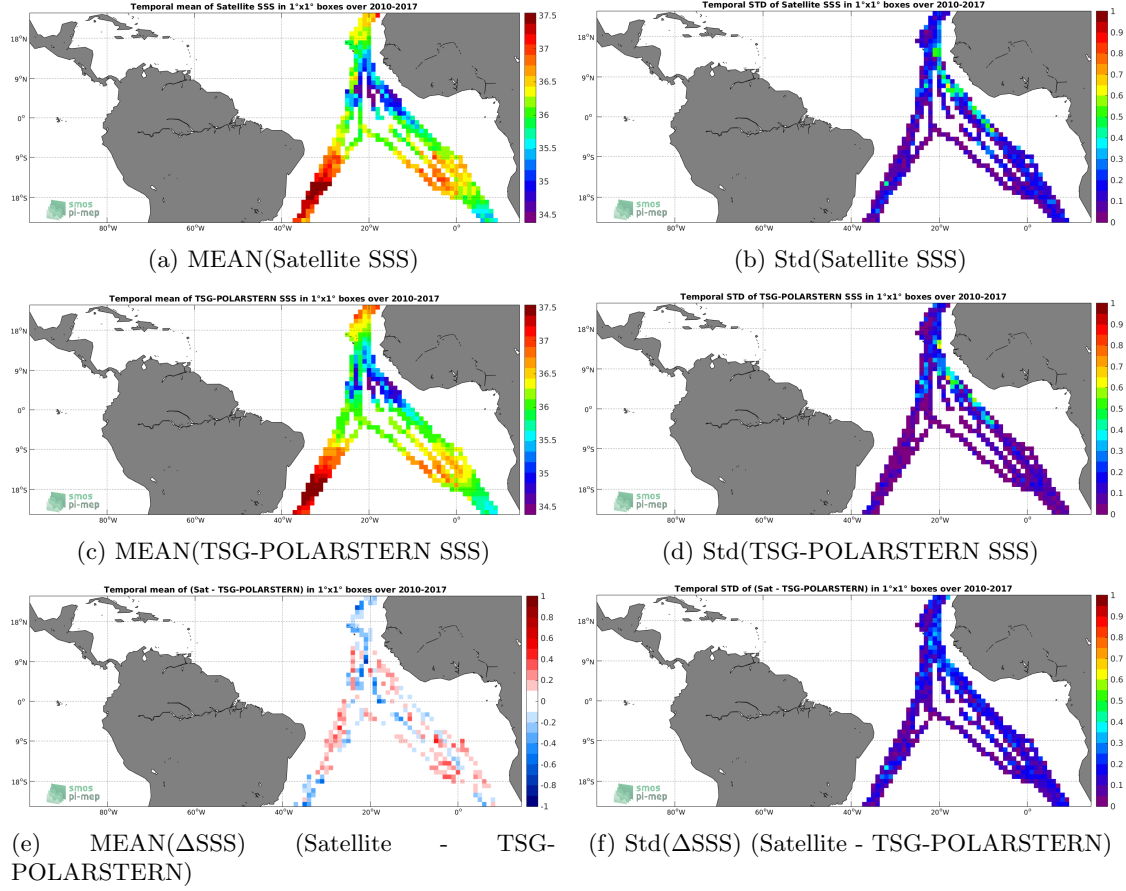
Figure 6: Temporal mean (left) and Std (right) of SSS from SMOS-L3-CATDS-CECOS-LOCEAN-V3-9DAYS-25KM (top), TSG-POLARSTERN (middle), and of \Delta SSS (Satellite - TSG-POLARSTERN). Only match-up pairs are used to generate these maps.
