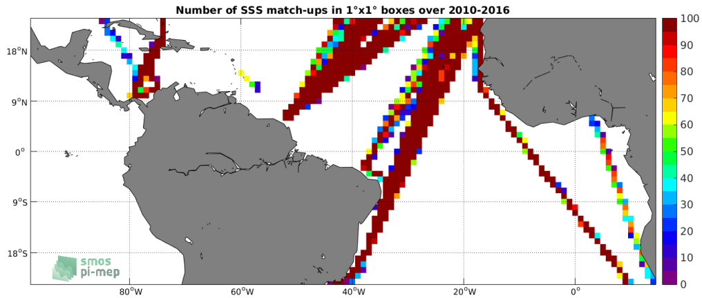
Figure 4: Number of SSS match-ups between TSG-LEGOS-DM SSS and the SMOS-L3-CATDS-CECOS-LOCEAN-V3-9DAYS-25KM SSS product for the Tropical Atlantic Ocean Pi-MEP region over 1^\circ \times 1^\circ boxes and for the full satellite product period.
