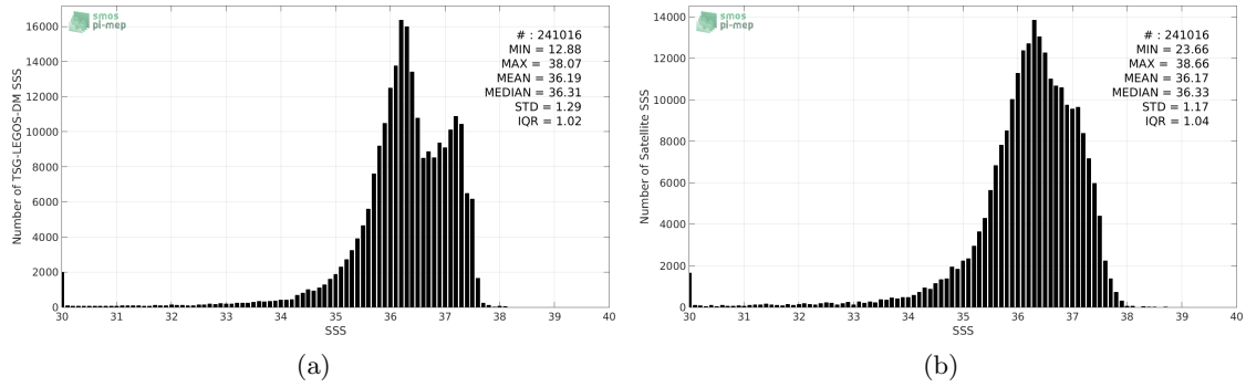
Figure 2: Histograms of SSS from TSG-LEGOS-DM (a) and SMOS-L3-CATDS-CECOS-LOCEAN-V3-9DAYS-25KM (b) considering all match-up pairs per bins of 0.1 over the Tropical Atlantic Ocean Pi-MEP region and for the full satellite product period.
