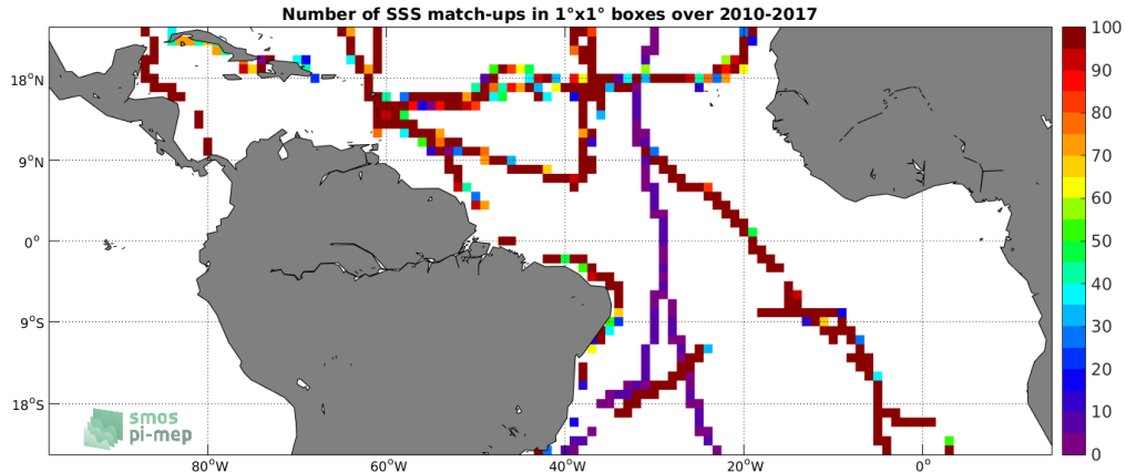
Figure 4: Number of SSS match-ups between TSG-GOSUD-Sailing-ship SSS and the SMOS-L3-CATDS-CECOS-LOCEAN-V3-9DAYS-25KM SSS product for the Tropical Atlantic Ocean Pi-MEP region over 1^\circ \times 1^\circ boxes and for the full satellite product period.
