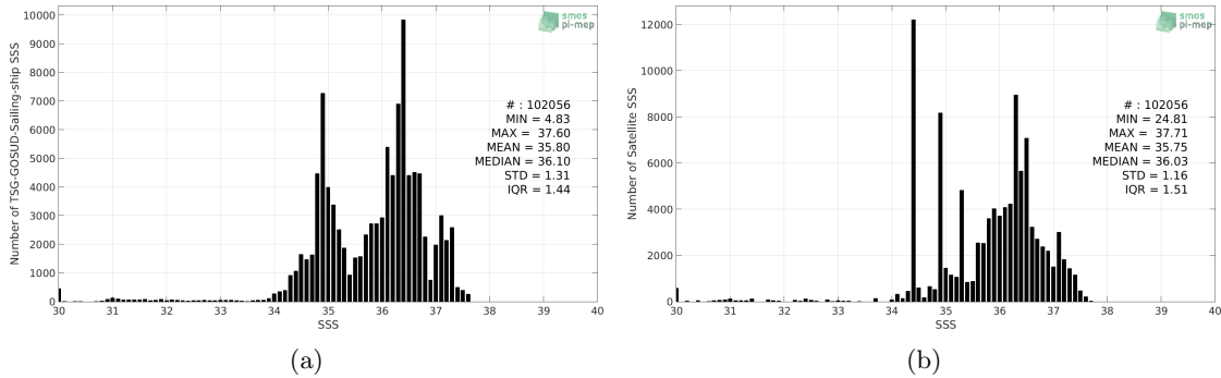
Figure 2: Histograms of SSS from TSG-GOSUD-Sailing-ship (a) and SMOS-L3-CATDS-CECOS-LOCEAN-V3-9DAYS-25KM (b) considering all match-up pairs per bins of 0.1 over the Tropical Atlantic Ocean Pi-MEP region and for the full satellite product period.
