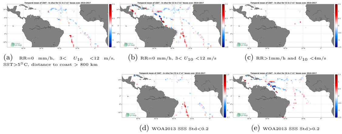
Figure 12: Temporal mean gridded over spatial boxes of size 1^\circ \times 1^\circ of \Delta SSS (SMOS-L3-CATDS-CECOS-LOCEAN-V3-9DAYS-25KM - TSG-GOSUD-Sailing-ship) for 5 different subdatasets corresponding to: RR=0 mm/h, 3 < U_{10} < 12 m/s, SST >5^\circ\text{C} , distance to coast > 800 km (a), RR=0 mm/h, 3 < U_{10} < 12 m/s (b), RR >1 mm/h and U_{10} < 4 m/s (c), WOA2013 SSS Std <0.2 (d), WOA2013 SSS Std >0.2 (e).
