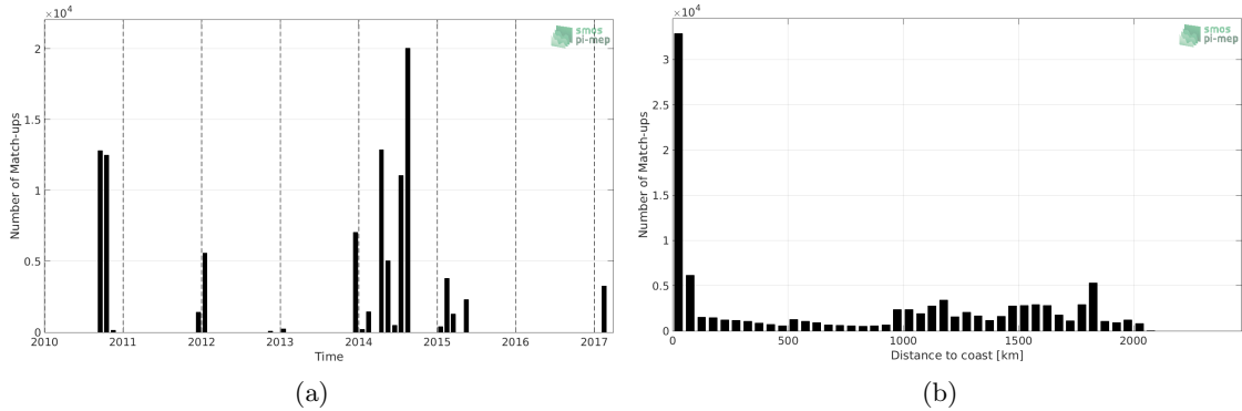
Figure 1: Number of match-ups between TSG-GOSUD-Sailing-ship and SMOS-L3-CATDS-CECOS-LOCEAN-V3-9DAYS-25KM SSS as a function of time (a) and as function of the distance to coast (b) over the Tropical Atlantic Ocean Pi-MEP region and for the full satellite product period.
