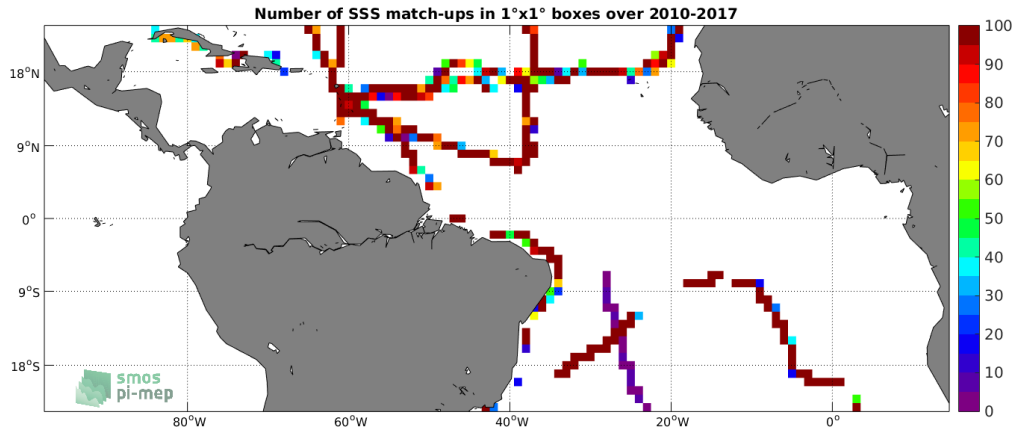
Figure 4: Number of SSS match-ups between TSG-GOSUD-Sailing-ship SSS and the SMOS-L3-CATDS-CECOS-LOCEAN-V3-9DAYS-25KM SSS product for the Tropical Atlantic Ocean Pi-MEP region over 1°x1° boxes and for the full satellite product period.
