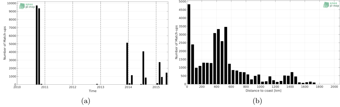
Figure 1: Number of match-ups between TSG-GOSUD-Sailing-ship and SMOS-L3-CATDS-CECOS-LOCEAN-V3-9DAYS-25KM SSS as a function of time (a) and as function of the distance to coast (b) over the Tropical Atlantic Ocean Pi-MEP region and for the full satellite product period.
