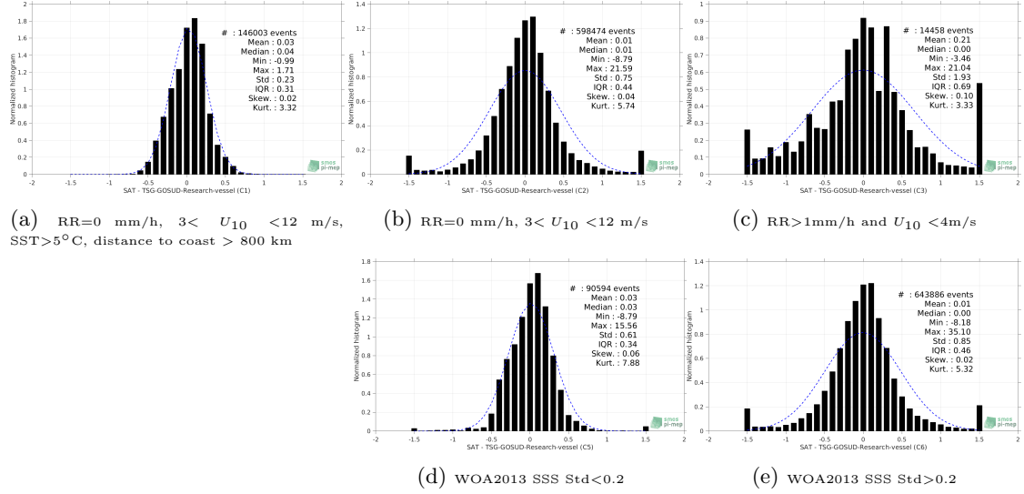
Figure 13: Normalized histogram of \Delta SSS (SMOS-L3-CATDS-CECOS-LOCEAN-V3-9DAYS-25KM - TSG-GOSUD-Research-vessel) for 5 different subdatasets corresponding to: RR=0 mm/h, 3 < U_{10} < 12 m/s, SST > 5°C, distance to coast > 800 km (a), RR=0 mm/h, 3 < U_{10} < 12 m/s (b), RR > 1mm/h and U_{10} < 4 m/s (c), WOA2013 SSS Std < 0.2 (d), WOA2013 SSS Std > 0.2 (e).
