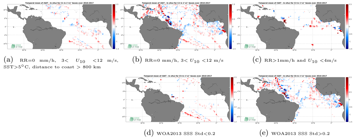
Figure 12: Temporal mean gridded over spatial boxes of size 1^\circ \times 1^\circ of \Delta SSS (SMOS-L3-CATDS-CECOS-LOCEAN-V3-9DAYS-25KM - TSG-GOSUD-Research-vessel) for 5 different subdatasets corresponding to:RR=0 mm/h, 3 < U_{10} < 12 m/s, SST >5^\circ\text{C} , distance to coast > 800 km (a), RR=0 mm/h, 3 < U_{10} < 12 m/s (b), RR >1 mm/h and U_{10} < 4 m/s (c), WOA2013 SSS Std <0.2 (d), WOA2013 SSS Std >0.2 (e).
