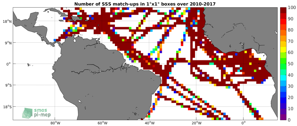
Figure 4: Number of SSS match-ups between TSG-GOSUD-Research-vessel SSS and the SMOS-L3-CATDS-CECOS-LOCEAN-V3-9DAYS-25KM SSS product for the Tropical Atlantic Ocean Pi-MEP region over 1°x1° boxes and for the full satellite product period.
