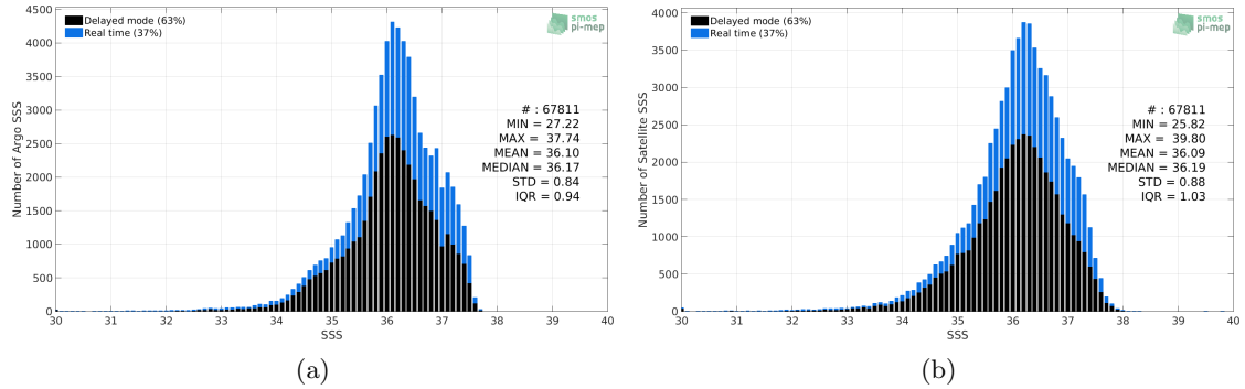
Figure 2: Histograms of SSS from Argo (a) and SMOS-L3-CATDS-CECOS-LOCEAN-V3-9DAYS-25KM (b) considering all match-up pairs per bins of 0.1 over the Tropical Atlantic Ocean Pi-MEP region and for the full satellite product period.
