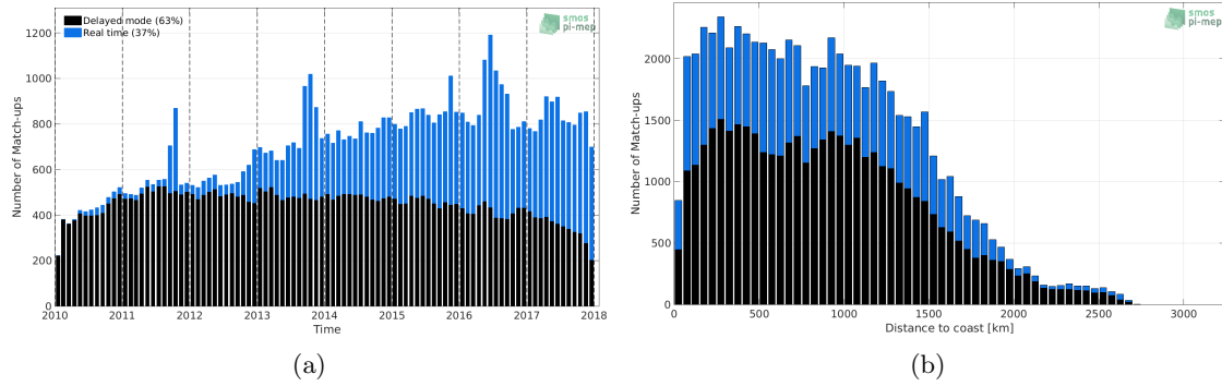
Figure 1: Number of match-ups between Argo and SMOS-L3-CATDS-CECOS-LOCEAN-V3-9DAYS-25KM SSS as a function of time (a) and as function of the distance to coast (b) over the Tropical Atlantic Ocean Pi-MEP region and for the full satellite product period.
