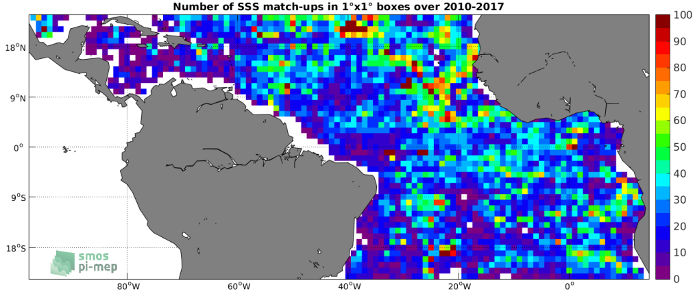
Figure 4: Number of SSS match-ups between Argo SSS and the SMOS-L3-CATDS-CECOS-LOCEAN-V3-9DAYS-25KM SSS product for the Tropical Atlantic Ocean Pi-MEP region over 1^\circ \times 1^\circ boxes and for the full satellite product period.
