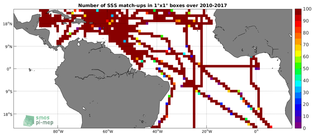
Figure 4: Number of SSS match-ups between TSG-SAMOS SSS and the SMOS-L3-CATDS-CECOS-LOCEAN-V3-18DAYS-25KM SSS product for the Tropical Atlantic Ocean Pi-MEP region over 1^\circ \times 1^\circ boxes and for the full satellite product period.
