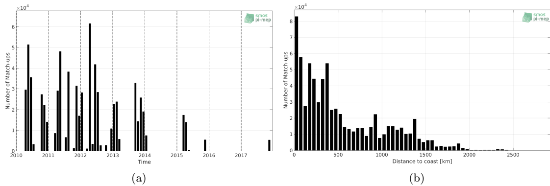
Figure 1: Number of match-ups between TSG-SAMOS and SMOS-L3-CATDS-CECOS-LOCEAN-V3-18DAYS-25KM SSS as a function of time (a) and as function of the distance to coast (b) over the Tropical Atlantic Ocean Pi-MEP region and for the full satellite product period.
