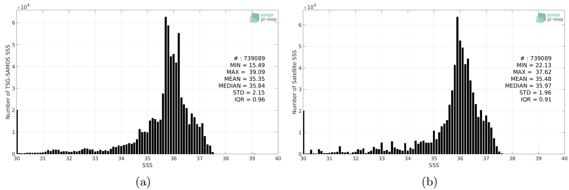
Figure 2: Histograms of SSS from TSG-SAMOS (a) and SMOS-L3-CATDS-CECOS-LOCEAN-V3-18DAYS-25KM (b) considering all match-up pairs per bins of 0.1 over the Tropical Atlantic Ocean Pi-MEP region and for the full satellite product period.
