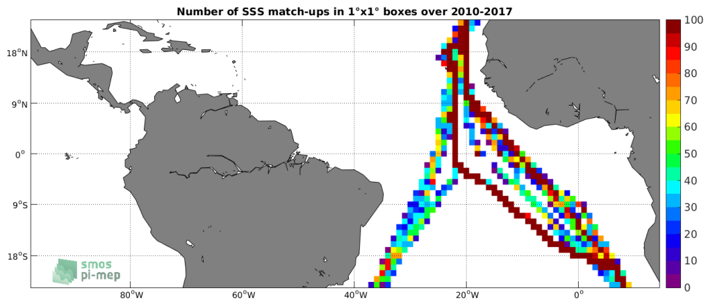
Figure 4: Number of SSS match-ups between TSG-POLARSTERN SSS and the SMOS-L3-CATDS-CECOS-LOCEAN-V3-18DAYS-25KM SSS product for the Tropical Atlantic Ocean Pi-MEP region over 1^\circ \times 1^\circ boxes and for the full satellite product period.
