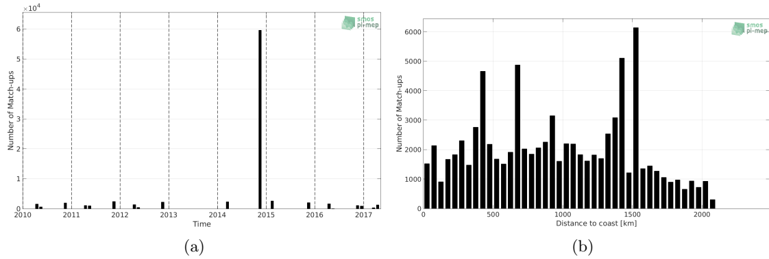
Figure 1: Number of match-ups between TSG-POLARSTERN and SMOS-L3-CATDS-CECOS-LOCEAN-V3-18DAYS-25KM SSS as a function of time (a) and as function of the distance to coast (b) over the Tropical Atlantic Ocean Pi-MEP region and for the full satellite product period.
