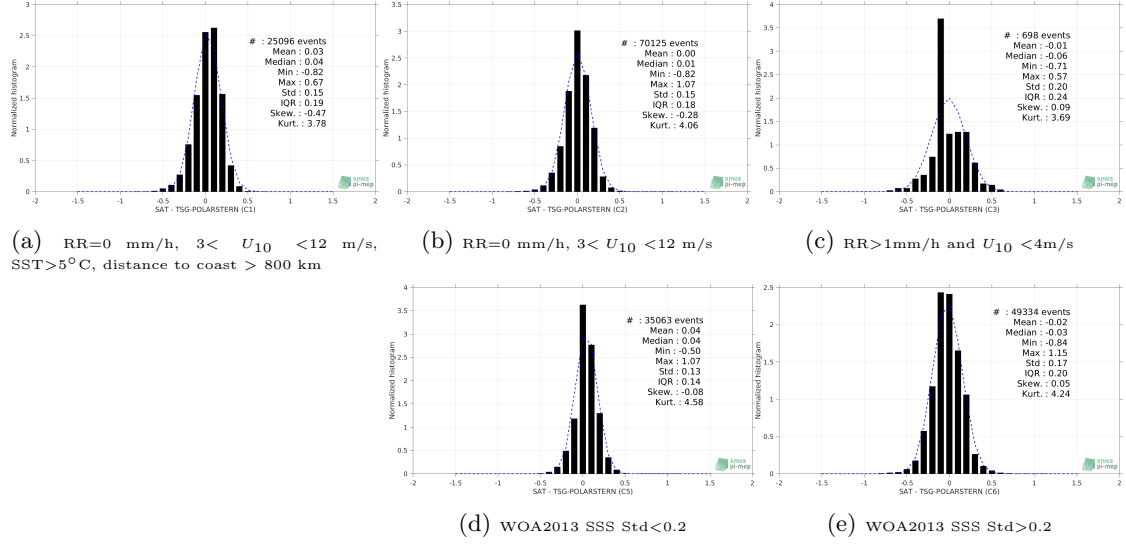
Figure 13: Normalized histogram of \Delta\text{SSS} (SMOS-L3-CATDS-CECOS-LOCEAN-V3-18DAYS-25KM - TSG-POLARSTERN) for 5 different subdatasets corresponding to: RR=0 mm/h, 3 < U_{10} < 12 m/s, SST > 5^{\circ}\text{C} , distance to coast > 800 km (a), RR=0 mm/h, 3 < U_{10} < 12 m/s (b), RR > 1\text{mm/h} and U_{10} < 4\text{m/s} (c), WOA2013 SSS Std < 0.2 (d), WOA2013 SSS Std > 0.2 (e).
