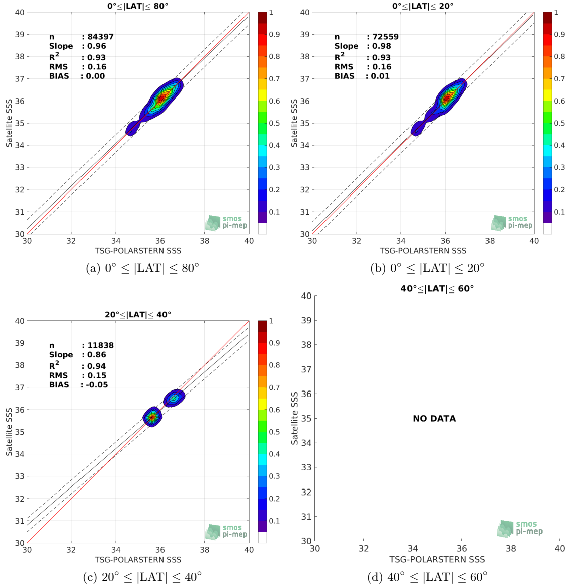
Figure 9: Contour maps of the concentration of SMOS-L3-CATDS-CECOS-LOCEAN-V3-18DAYS-25KM SSS (y-axis) versus TSG-POLARSTERN SSS (x-axis) at match-up pairs for different latitude bands. For each plot, the red line shows x=y . The black thin and dashed lines indicate a linear fit through the data cloud and the \pm 95\% confidence levels, respectively. The number match-up pairs n , the slope and R^2 coefficient of the linear fit, the root mean square (RMS) and the mean bias between satellite and in situ data are indicated for each latitude band in each plots.
