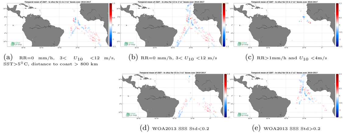
Figure 12: Temporal mean gridded over spatial boxes of size 1^\circ \times 1^\circ of \Delta SSS (SMOS-L3-CATDS-CECOS-LOCEAN-V3-18DAYS-25KM - TSG-POLARSTERN) for 5 different subdatasets corresponding to:RR=0 mm/h, 3 < U_{10} < 12 m/s, SST >5^\circ\text{C} , distance to coast > 800 km (a), RR=0 mm/h, 3 < U_{10} < 12 m/s (b), RR >1 mm/h and U_{10} < 4 m/s (c), WOA2013 SSS Std <0.2 (d), WOA2013 SSS Std >0.2 (e).
