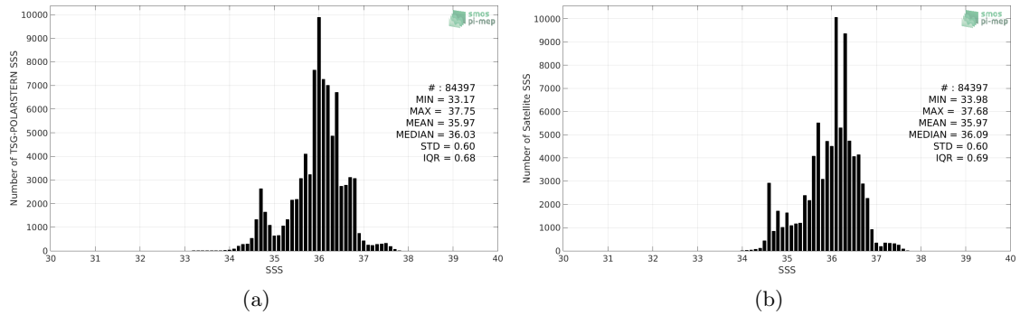
Figure 2: Histograms of SSS from TSG-POLARSTERN (a) and SMOS-L3-CATDS-CECOS-LOCEAN-V3-18DAYS-25KM (b) considering all match-up pairs per bins of 0.1 over the Tropical Atlantic Ocean Pi-MEP region and for the full satellite product period.
