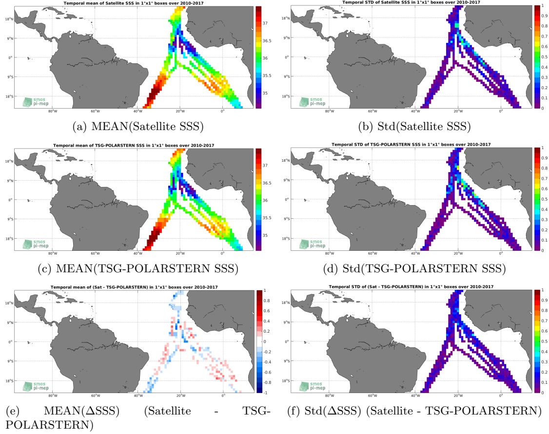
Figure 6: Temporal mean (left) and Std (right) of SSS from SMOS-L3-CATDS-CECOS-LOCEAN-V3-18DAYS-25KM (top), TSG-POLARSTERN (middle), and of \Delta SSS (Satellite - TSG-POLARSTERN). Only match-up pairs are used to generate these maps.
