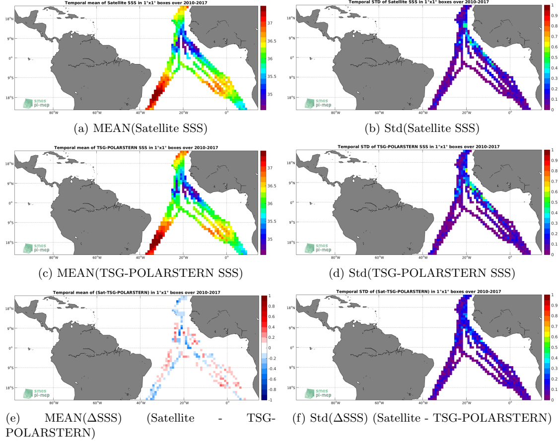
Figure 6: Temporal mean (left) and Std (right) of SSS from SMOS-L3-CATDS-CECOS-LOCEAN-V3-18DAYS-25KM (top), TSG-POLARSTERN (middle), and of \Delta\text{SSS} (Satellite - TSG-POLARSTERN). Only match-up pairs are used to generate these maps.
