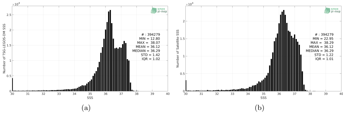
Figure 2: Histograms of SSS from TSG-LEGOS-DM (a) and SMOS-L3-CATDS-CECOS-LOCEAN-V3-18DAYS-25KM (b) considering all match-up pairs per bins of 0.1 over the Tropical Atlantic Ocean Pi-MEP region and for the full satellite product period.
