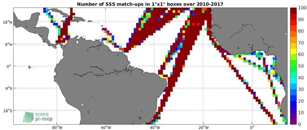
Figure 4: Number of SSS match-ups between TSG-LEGOS-DM SSS and the SMOS-L3-CATDS-CECOS-LOCEAN-V3-18DAYS-25KM SSS product for the Tropical Atlantic Ocean Pi-MEP region over 1°x1° boxes and for the full satellite product period.
