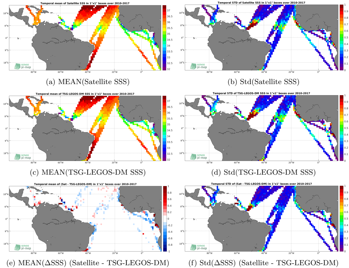
Figure 6: Temporal mean (left) and Std (right) of SSS from SMOS-L3-CATDS-CECOS-LOCEAN-V3-18DAYS-25KM (top), TSG-LEGOS-DM (middle), and of \Delta SSS (Satellite - TSG-LEGOS-DM). Only match-up pairs are used to generate these maps.
