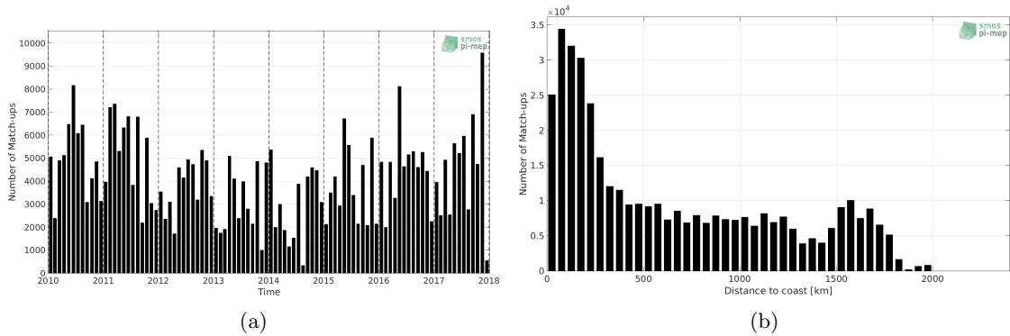
Figure 1: Number of match-ups between TSG-LEGOS-DM and SMOS-L3-CATDS-CECOS-LOCEAN-V3-18DAYS-25KM SSS as a function of time (a) and as function of the distance to coast (b) over the Tropical Atlantic Ocean Pi-MEP region and for the full satellite product period.
