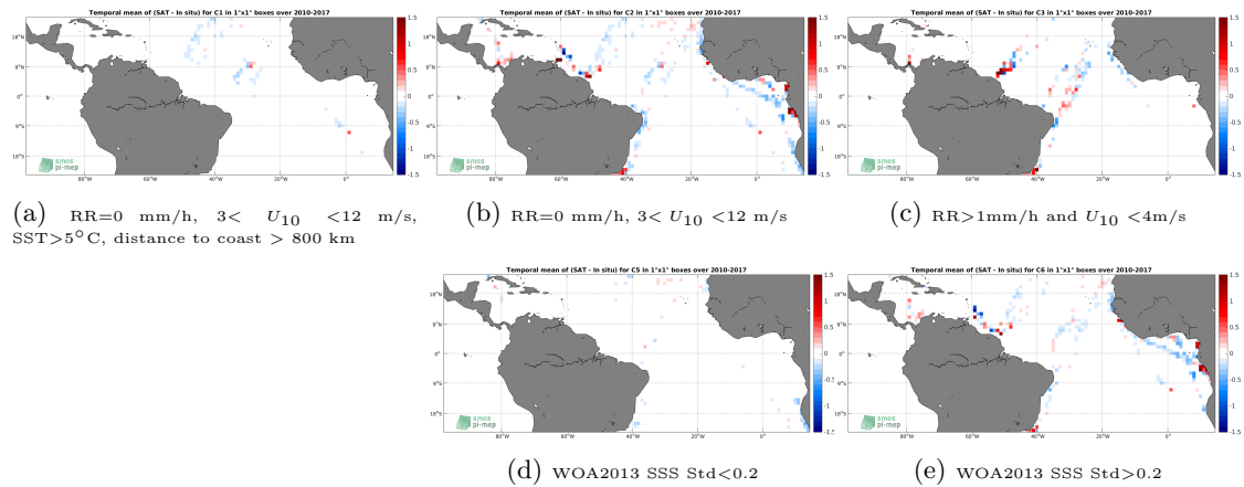
Figure 12: Temporal mean gridded over spatial boxes of size 1^\circ \times 1^\circ of \Delta SSS (SMOS-L3-CATDS-CECOS-LOCEAN-V3-18DAYS-25KM - TSG-LEGOS-DM) for 5 different subdatasets corresponding to:RR=0 mm/h, 3 < U_{10} < 12 m/s, SST >5^\circ\text{C} , distance to coast > 800 km (a), RR=0 mm/h, 3 < U_{10} < 12 m/s (b), RR >1 mm/h and U_{10} < 4 m/s (c), WOA2013 SSS Std <0.2 (d), WOA2013 SSS Std >0.2 (e).
