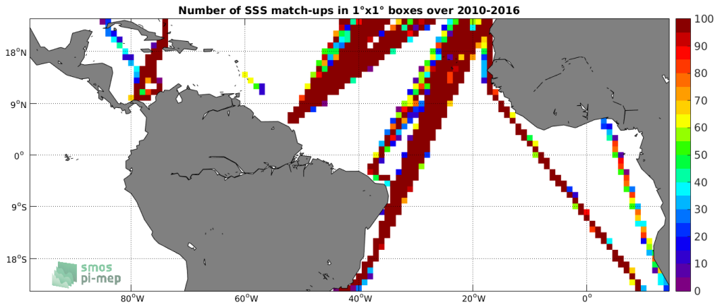
Figure 4: Number of SSS match-ups between TSG-LEGOS-DM SSS and the SMOS-L3-CATDS-CECOS-LOCEAN-V3-18DAYS-25KM SSS product for the Tropical Atlantic Ocean Pi-MEP region over 1^\circ \times 1^\circ boxes and for the full satellite product period.
