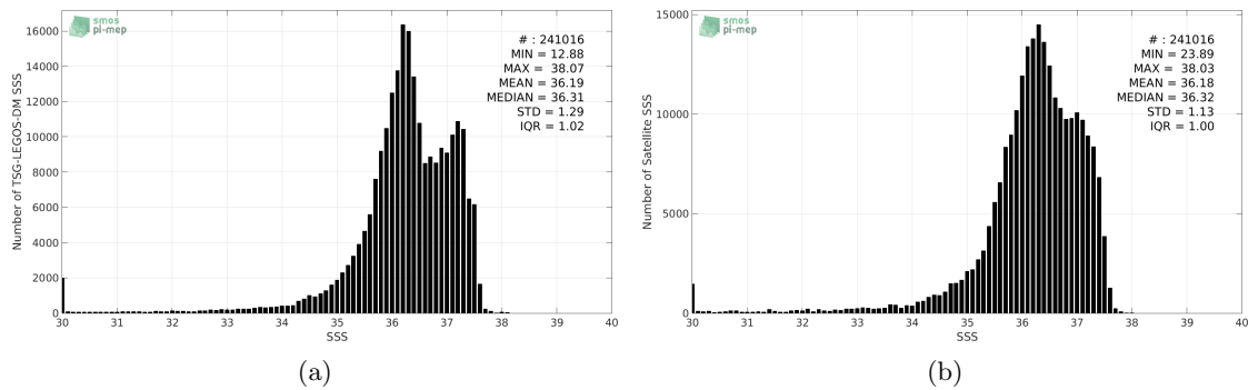
Figure 2: Histograms of SSS from TSG-LEGOS-DM (a) and SMOS-L3-CATDS-CECOS-LOCEAN-V3-18DAYS-25KM (b) considering all match-up pairs per bins of 0.1 over the Tropical Atlantic Ocean Pi-MEP region and for the full satellite product period.
