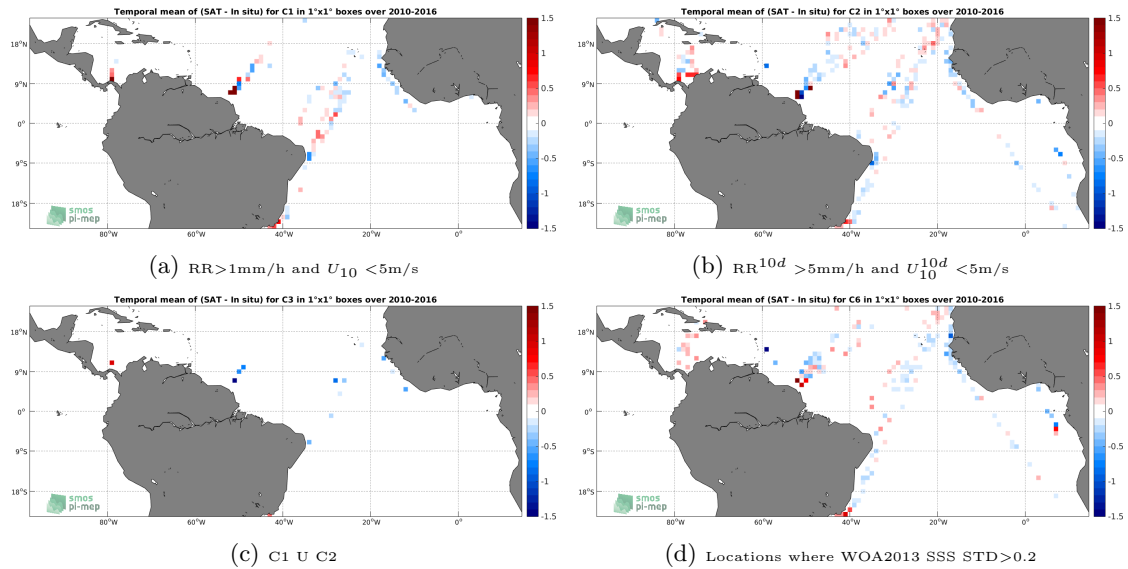
Figure 12: Temporal mean gridded over spatial boxes of size 1^\circ \times 1^\circ of \Delta SSS (SMOS-L3-CATDS-CECOS-LOCEAN-V3-18DAYS-25KM - TSG-LEGOS-DM) for 4 different subdatasets corresponding to:RR >1 mm/h and U_{10} < 5 m/s (a), RR 10d > 5 mm/h and U_{10}^{10d} < 5 m/s (b), C1 U C2 (c),Locations where WOA2013 SSS STD >0.2 (d).
