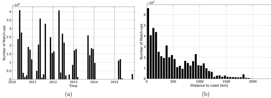
Figure 1: Number of match-ups between TSG-SAMOS and SMOS-L3-CATDS-CECOS-LOCEAN-V2-9DAYS-25KM SSS as a function of time (a) and as function of the distance to coast (b) over the Tropical Atlantic Ocean Pi-MEP region and for the full satellite product period.
