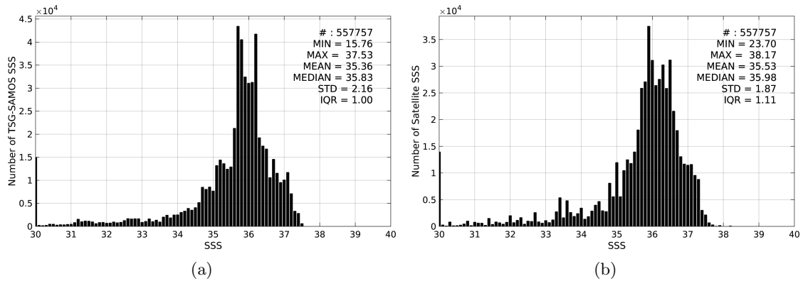
Figure 2: Histograms of SSS from TSG-SAMOS (a) and SMOS-L3-CATDS-CECOS-LOCEAN-V2-9DAYS-25KM (b) considering all match-up pairs per bins of 0.1 over the Tropical Atlantic Ocean Pi-MEP region and for the full satellite product period.
