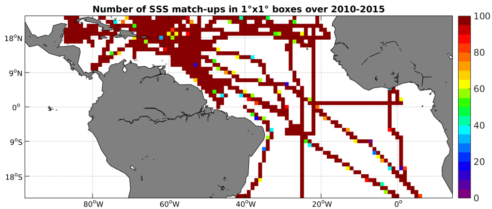
Figure 4: Number of SSS match-ups between TSG-SAMOS SSS and the SMOS-L3-CATDS-CECOS-LOCEAN-V2-9DAYS-25KM SSS product for the Tropical Atlantic Ocean Pi-MEP region over 1^\circ \times 1^\circ boxes and for the full satellite product period.
