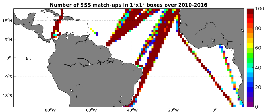
Figure 4: Number of SSS match-ups between TSG-LEGOS-DM SSS and the SMOS-L3-CATDS-CECOS-LOCEAN-V2-9DAYS-25KM SSS product for the Tropical Atlantic Ocean Pi-MEP region over 1^\circ \times 1^\circ boxes and for the full satellite product period.
