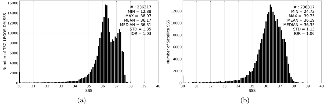
Figure 2: Histograms of SSS from TSG-LEGOS-DM (a) and SMOS-L3-CATDS-CECOS-LOCEAN-V2-9DAYS-25KM (b) considering all match-up pairs per bins of 0.1 over the Tropical Atlantic Ocean Pi-MEP region and for the full satellite product period.
