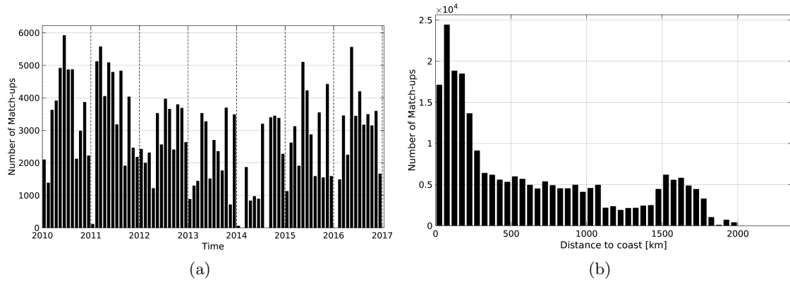
Figure 1: Number of match-ups between TSG-LEGOS-DM and SMOS-L3-CATDS-CECOS-LOCEAN-V2-9DAYS-25KM SSS as a function of time (a) and as function of the distance to coast (b) over the Tropical Atlantic Ocean Pi-MEP region and for the full satellite product period.
