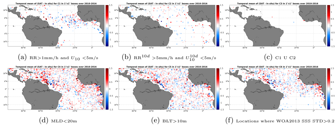
Figure 12: Temporal mean gridded over spatial boxes of size 1^\circ \times 1^\circ of \Delta SSS (SMOS-L3-CATDS-CECOS-LOCEAN-V2-9DAYS-25KM - Argo) for 6 different subdatasets corresponding to: RR > 1\text{mm/h} and U_{10} < 5\text{m/s} (a), RR^{10d} > 5\text{mm/h} and U_{10}^{10d} < 5\text{m/s} (b), C1 U C2 (c), MLD < 20\text{m} (d), BLT > 10\text{m} (e), Locations where WOA2013 SSS STD > 0.2 (f).
