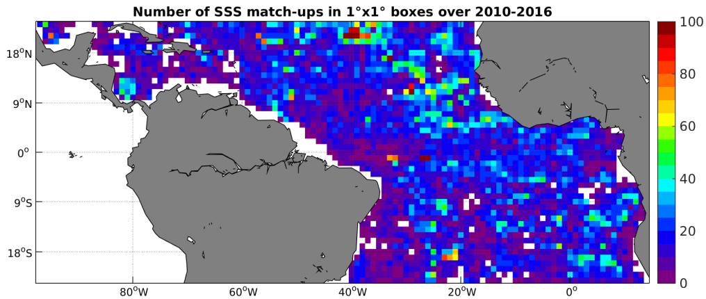
Figure 4: Number of SSS match-ups between Argo SSS and the SMOS-L3-CATDS-CECOS-LOCEAN-V2-9DAYS-25KM SSS product for the Tropical Atlantic Ocean Pi-MEP region over 1^\circ \times 1^\circ boxes and for the full satellite product period.
