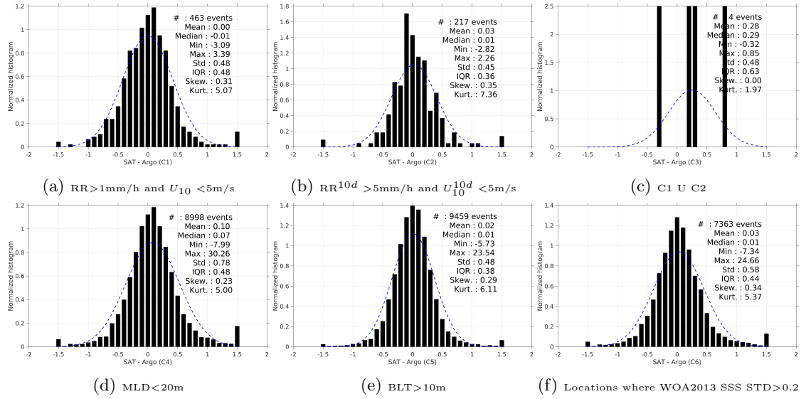
Figure 13: Normalized histogram of \Delta SSS (SMOS-L3-CATDS-CECOS-LOCEAN-V2-9DAYS-25KM - Argo) for 6 different subdatasets corresponding to: RR>1mm/h and U_{10} <5m/s (a), RR 10d >5mm/h and U_{10}^{10d} <5m/s (b), C1 U C2 (c),MLD<20m (d),BLT>10m (e),Locations where WOA2013 SSS STD>0.2 (f).
