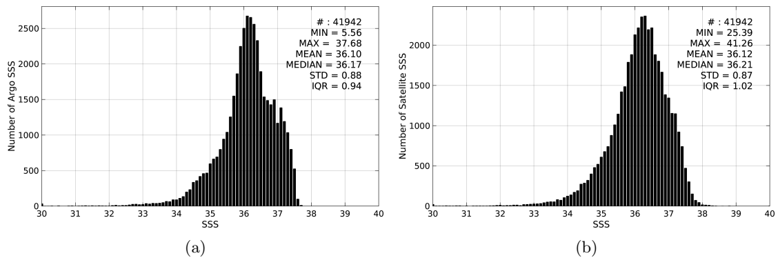
Figure 2: Histograms of SSS from Argo (a) and SMOS-L3-CATDS-CECOS-LOCEAN-V2-9DAYS-25KM (b) considering all match-up pairs per bins of 0.1 over the Tropical Atlantic Ocean Pi-MEP region and for the full satellite product period.
