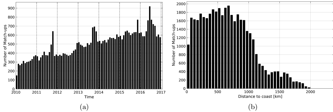
Figure 1: Number of match-ups between Argo and SMOS-L3-CATDS-CECOS-LOCEAN-V2-9DAYS-25KM SSS as a function of time (a) and as function of the distance to coast (b) over the Tropical Atlantic Ocean Pi-MEP region and for the full satellite product period.
