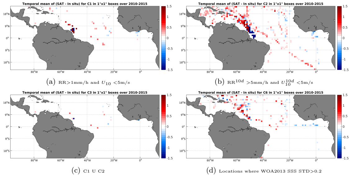
Figure 12: Temporal mean gridded over spatial boxes of size 1^\circ \times 1^\circ of \Delta SSS (SMOS-L3-CATDS-CECOS-LOCEAN-V2-18DAYS-25KM - TSG-SAMOS) for 4 different subdatasets corresponding to: RR > 1\text{mm/h} and U_{10} < 5\text{m/s} (a), RR^{10d} > 5\text{mm/h} and U_{10}^{10d} < 5\text{m/s} (b), C1 U C2 (c), Locations where WOA2013 SSS STD > 0.2 (d).
