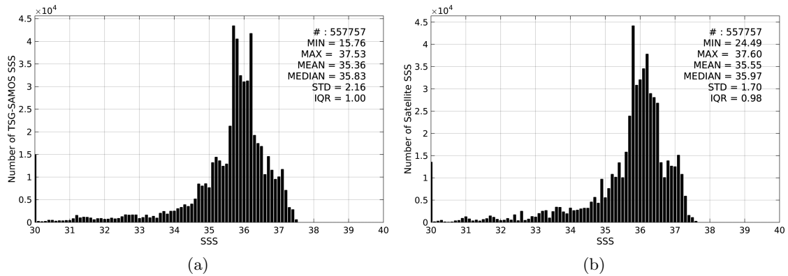
Figure 2: Histograms of SSS from TSG-SAMOS (a) and SMOS-L3-CATDS-CECOS-LOCEAN-V2-18DAYS-25KM (b) considering all match-up pairs per bins of 0.1 over the Tropical Atlantic Ocean Pi-MEP region and for the full satellite product period.
