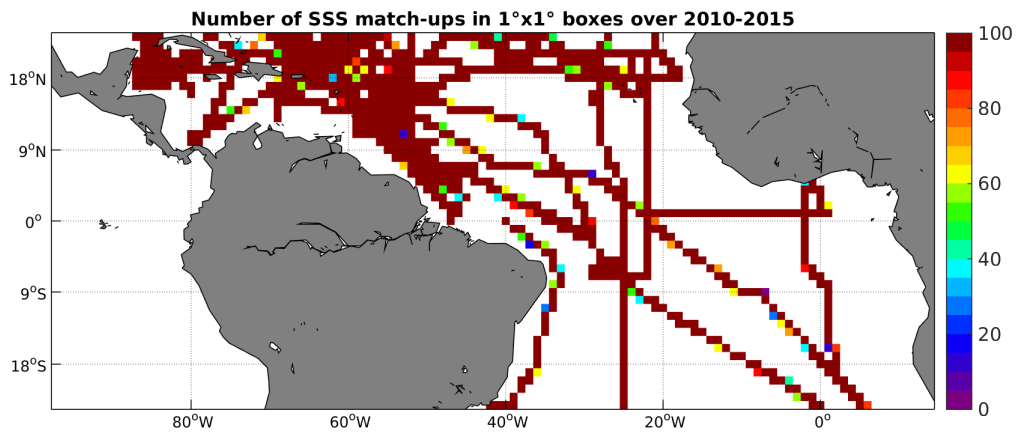
Figure 4: Number of SSS match-ups between TSG-SAMOS SSS and the SMOS-L3-CATDS-CECOS-LOCEAN-V2-18DAYS-25KM SSS product for the Tropical Atlantic Ocean Pi-MEP region over 1^\circ \times 1^\circ boxes and for the full satellite product period.
