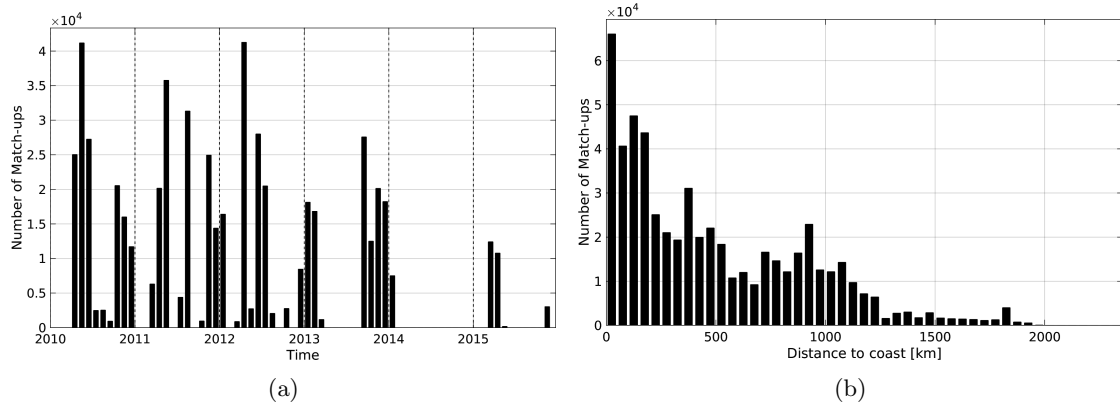
Figure 1: Number of match-ups between TSG-SAMOS and SMOS-L3-CATDS-CECOS-LOCEAN-V2-18DAYS-25KM SSS as a function of time (a) and as function of the distance to coast (b) over the Tropical Atlantic Ocean Pi-MEP region and for the full satellite product period.
