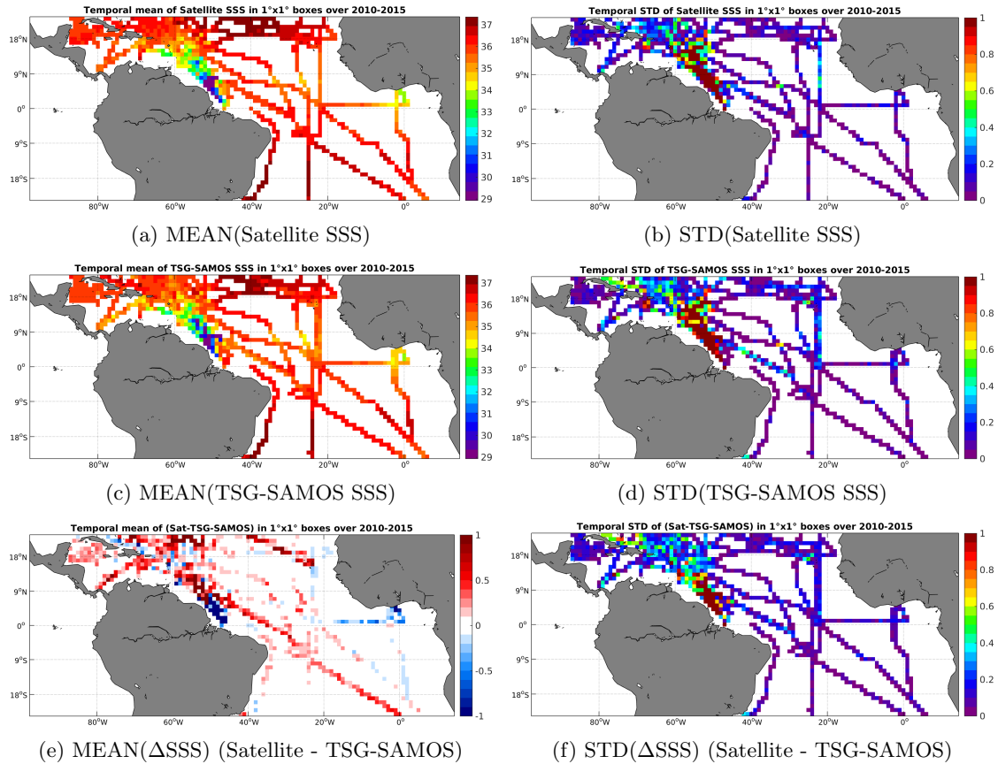
Figure 6: Temporal mean (left) and STD (right) of SSS from SMOS-L3-CATDS-CECOS-LOCEAN-V2-18DAYS-25KM (top), TSG-SAMOS (middle), and of \Delta SSS (Satellite - TSG-SAMOS). Only match-up pairs are used to generate these maps.
