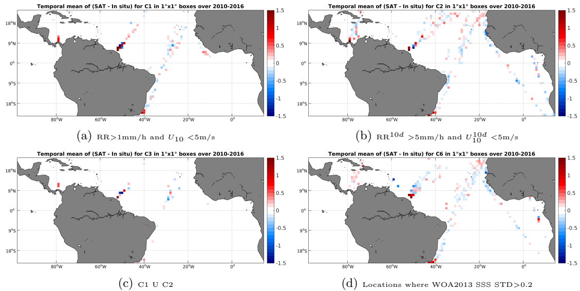
Figure 12: Temporal mean gridded over spatial boxes of size 1^\circ \times 1^\circ of \Delta SSS (SMOS-L3-CATDS-CECOS-LOCEAN-V2-18DAYS-25KM - TSG-LEGOS-DM) for 4 different subdatasets corresponding to:RR>1mm/h and U_{10} < 5 m/s (a), RR^{10d} > 5 mm/h and U_{10}^{10d} < 5 m/s (b), C1 U C2 (c),Locations where WOA2013 SSS STD>0.2 (d).
