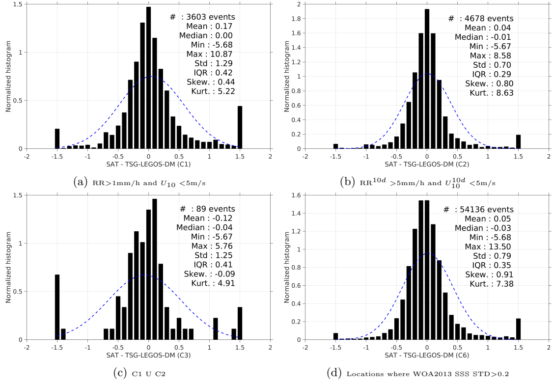
Figure 13: Normalized histogram of \Delta\text{SSS} (SMOS-L3-CATDS-CECOS-LOCEAN-V2-18DAYS-25KM - TSG-LEGOS-DM) for 6 different subdatasets corresponding to: RR > 1mm/h and U_{10} < 5\text{m/s} (a), RR^{10d} > 5\text{mm/h} and U_{10}^{10d} < 5\text{m/s} (b), C1 U C2 (c), Locations where WOA2013 SSS STD > 0.2 (d).
