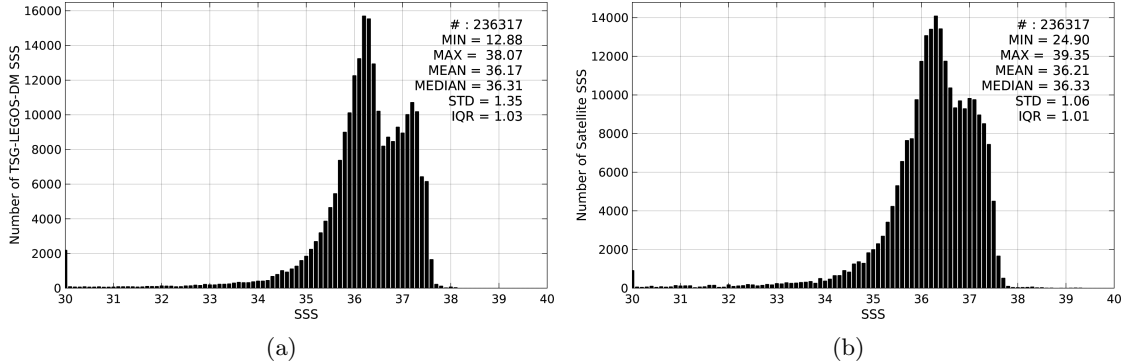
Figure 2: Histograms of SSS from TSG-LEGOS-DM (a) and SMOS-L3-CATDS-CECOS-LOCEAN-V2-18DAYS-25KM (b) considering all match-up pairs per bins of 0.1 over the Tropical Atlantic Ocean Pi-MEP region and for the full satellite product period.
