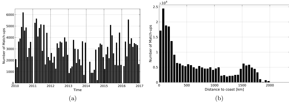
Figure 1: Number of match-ups between TSG-LEGOS-DM and SMOS-L3-CATDS-CECOS-LOCEAN-V2-18DAYS-25KM SSS as a function of time (a) and as function of the distance to coast (b) over the Tropical Atlantic Ocean Pi-MEP region and for the full satellite product period.
