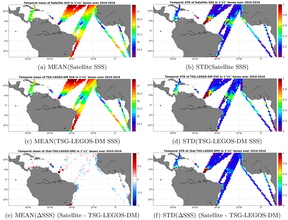
Figure 6: Temporal mean (left) and STD (right) of SSS from SMOS-L3-CATDS-CECOS-LOCEAN-V2-18DAYS-25KM (top), TSG-LEGOS-DM (middle), and of \Delta SSS (Satellite - TSG-LEGOS-DM). Only match-up pairs are used to generate these maps.
