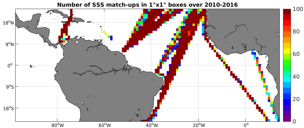
Figure 4: Number of SSS match-ups between TSG-LEGOS-DM SSS and the SMOS-L3-CATDS-CECOS-LOCEAN-V2-18DAYS-25KM SSS product for the Tropical Atlantic Ocean Pi-MEP region over 1^\circ \times 1^\circ boxes and for the full satellite product period.
