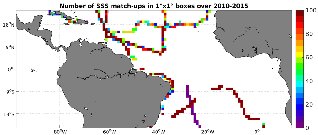
Figure 4: Number of SSS match-ups between TSG-GOSUD-Sailing-ship SSS and the SMOS-L3-CATDS-CECOS-LOCEAN-V2-18DAYS-25KM SSS product for the Tropical Atlantic Ocean Pi-MEP region over 1^\circ \times 1^\circ boxes and for the full satellite product period.
