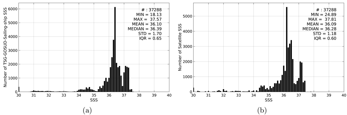
Figure 2: Histograms of SSS from TSG-GOSUD-Sailing-ship (a) and SMOS-L3-CATDS-CECOS-LOCEAN-V2-18DAYS-25KM (b) considering all match-up pairs per bins of 0.1 over the Tropical Atlantic Ocean Pi-MEP region and for the full satellite product period.
