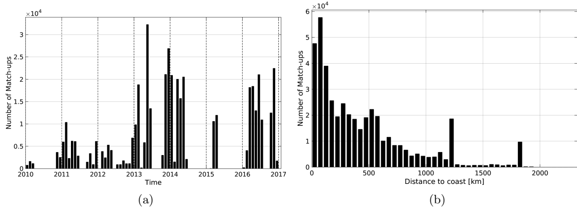
Figure 1: Number of match-ups between TSG-GOSUD-Research-vessel and SMOS-L3-CATDS-CECOS-LOCEAN-V2-18DAYS-25KM SSS as a function of time (a) and as function of the distance to coast (b) over the Tropical Atlantic Ocean Pi-MEP region and for the full satellite product period.
