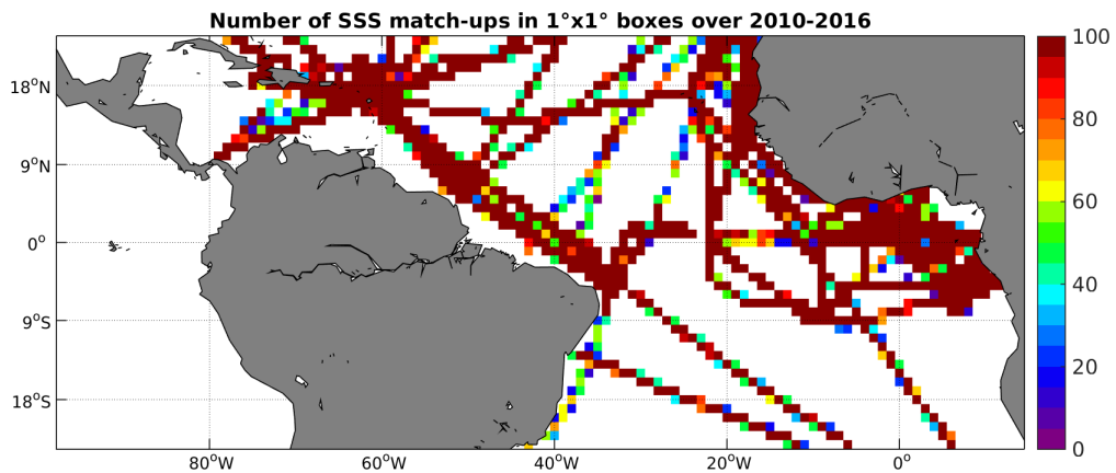
Figure 4: Number of SSS match-ups between TSG-GOSUD-Research-vessel SSS and the SMOS-L3-CATDS-CECOS-LOCEAN-V2-18DAYS-25KM SSS product for the Tropical Atlantic Ocean Pi-MEP region over 1^\circ \times 1^\circ boxes and for the full satellite product period.
