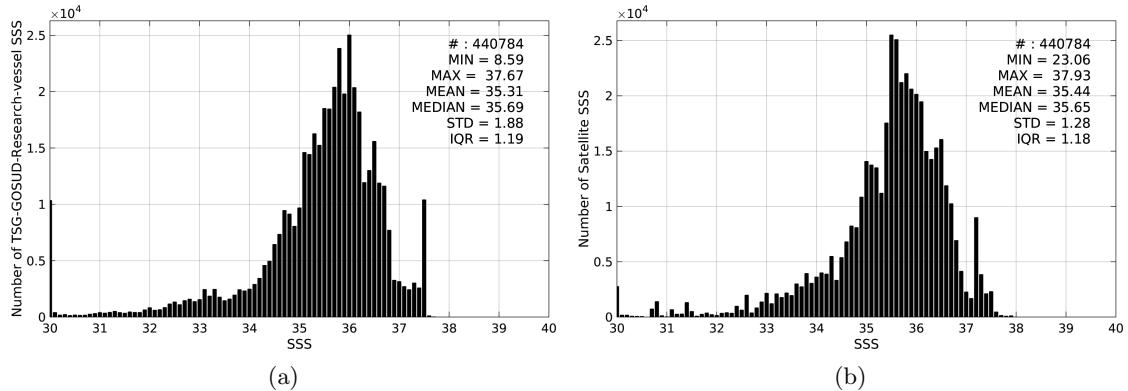
Figure 2: Histograms of SSS from TSG-GOSUD-Research-vessel (a) and SMOS-L3-CATDS-CECOS-LOCEAN-V2-18DAYS-25KM (b) considering all match-up pairs per bins of 0.1 over the Tropical Atlantic Ocean Pi-MEP region and for the full satellite product period.
