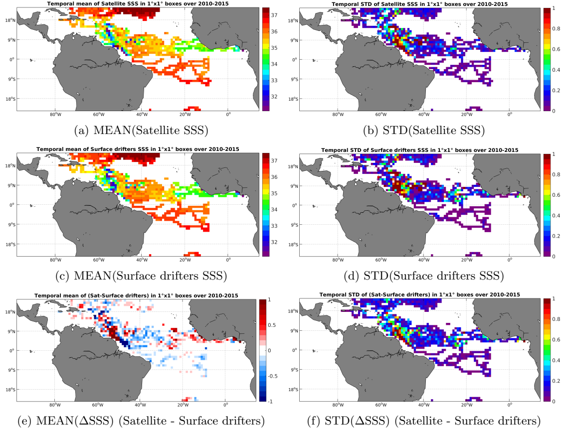
Figure 5: Temporal mean (left) and STD (right) of SSS from SMOS-L3-CATDS-CECOS-LOCEAN-V2-18DAYS-25KM (top), Surface drifters (middle), and of \Delta SSS (Satellite - Surface drifters). Only match-up pairs are used to generate these maps.
