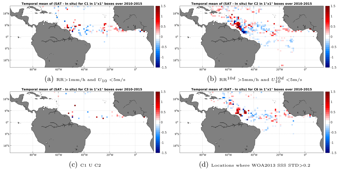
Figure 11: Temporal mean gridded over spatial boxes of size 1^\circ \times 1^\circ of \Delta SSS (SMOS-L3-CATDS-CECOS-LOCEAN-V2-18DAYS-25KM - Surface drifters) for 4 different subdatasets corresponding to: RR > 1mm/h and U_{10} < 5 m/s (a), RR^{10d} > 5 mm/h and U_{10}^{10d} < 5 m/s (b), C1 U C2 (c), Locations where WOA2013 SSS STD > 0.2 (d).
