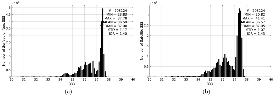
Figure 2: Histograms of SSS from Surface drifters (a) and SMOS-L3-CATDS-CECOS-LOCEAN-V2-18DAYS-25KM (b) considering all match-up pairs per bins of 0.1 over the Tropical Atlantic Ocean Pi-MEP region and for the full satellite product period.
