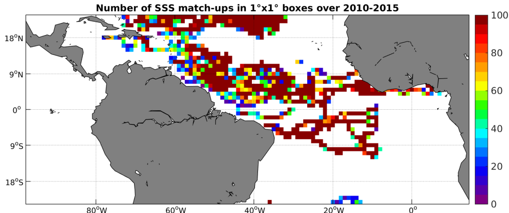
Figure 3: Number of SSS match-ups between Surface drifters SSS and the SMOS-L3-CATDS-CECOS-LOCEAN-V2-18DAYS-25KM SSS product for the Tropical Atlantic Ocean Pi-MEP region over 1^\circ \times 1^\circ boxes and for the full satellite product period.
