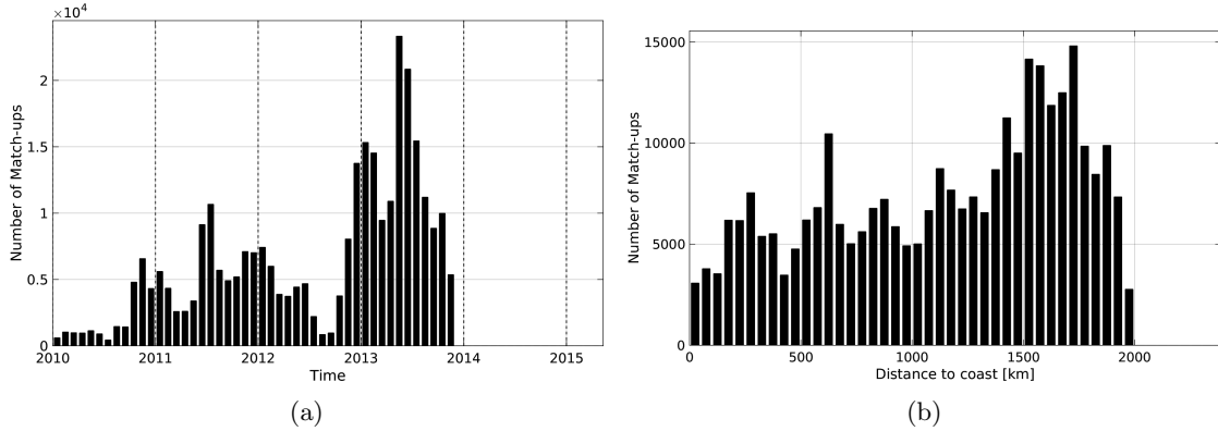
Figure 1: Number of match-ups between Surface drifters and SMOS-L3-CATDS-CECOS-LOCEAN-V2-18DAYS-25KM SSS as a function of time (a) and as function of the distance to coast (b) over the Tropical Atlantic Ocean Pi-MEP region and for the full satellite product period.
