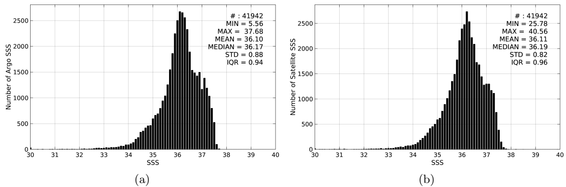
Figure 2: Histograms of SSS from Argo (a) and SMOS-L3-CATDS-CECOS-LOCEAN-V2-18DAYS-25KM (b) considering all match-up pairs per bins of 0.1 over the Tropical Atlantic Ocean Pi-MEP region and for the full satellite product period.
