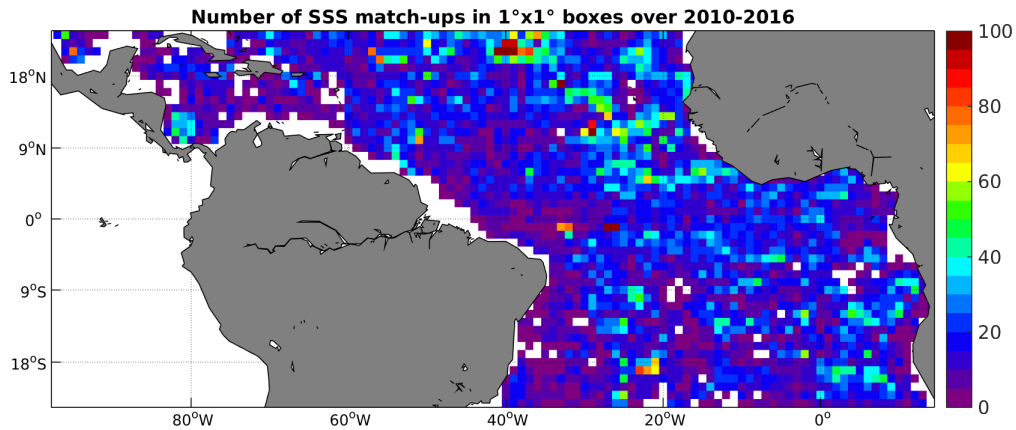
Figure 4: Number of SSS match-ups between Argo SSS and the SMOS-L3-CATDS-CECOS-LOCEAN-V2-18DAYS-25KM SSS product for the Tropical Atlantic Ocean Pi-MEP region over 1^\circ \times 1^\circ boxes and for the full satellite product period.
