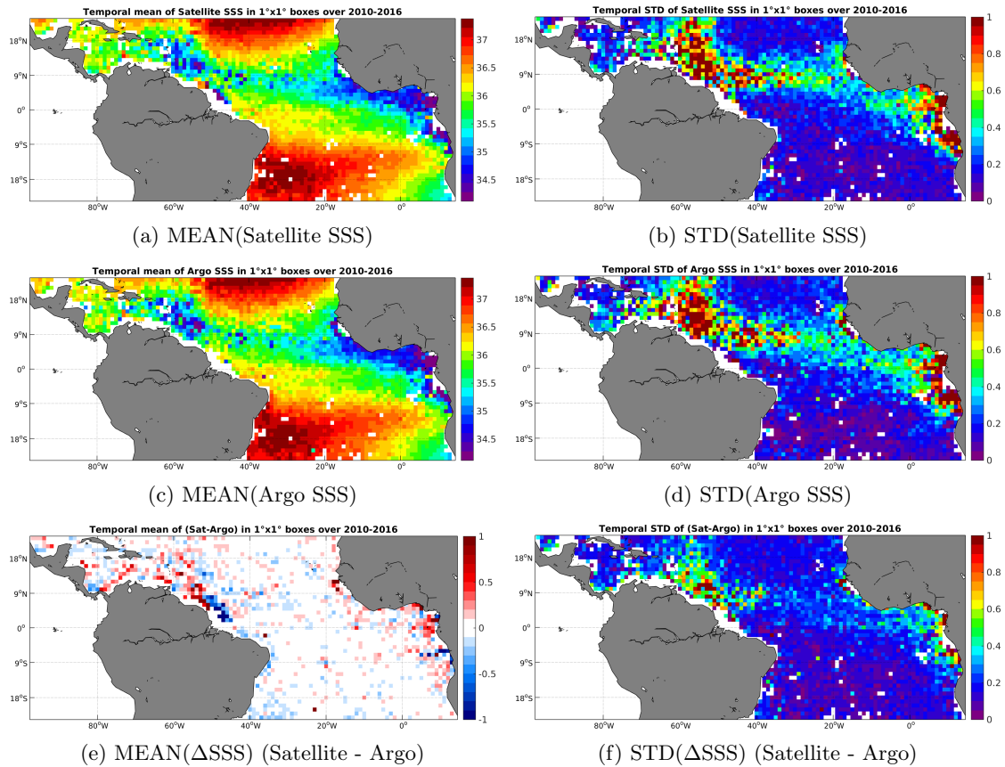
Figure 6: Temporal mean (left) and STD (right) of SSS from SMOS-L3-CATDS-CECOS-LOCEAN-V2-18DAYS-25KM (top), Argo (middle), and of \Delta SSS (Satellite - Argo). Only match-up pairs are used to generate these maps.
