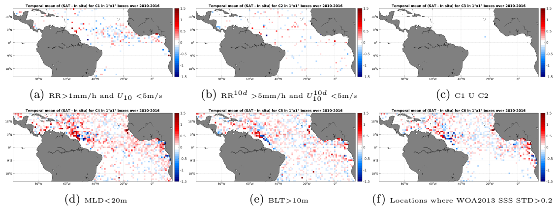
Figure 12: Temporal mean gridded over spatial boxes of size 1^\circ \times 1^\circ of \Delta SSS (SMOS-L3-CATDS-CECOS-LOCEAN-V2-18DAYS-25KM - Argo) for 6 different subdatasets corresponding to: RR > 1 mm/h and U_{10} < 5 m/s (a), RR^{10d} > 5 mm/h and U_{10}^{10d} < 5 m/s (b), C1 U C2 (c), MLD < 20 m (d), BLT > 10 m (e), Locations where WOA2013 SSS STD > 0.2 (f).
