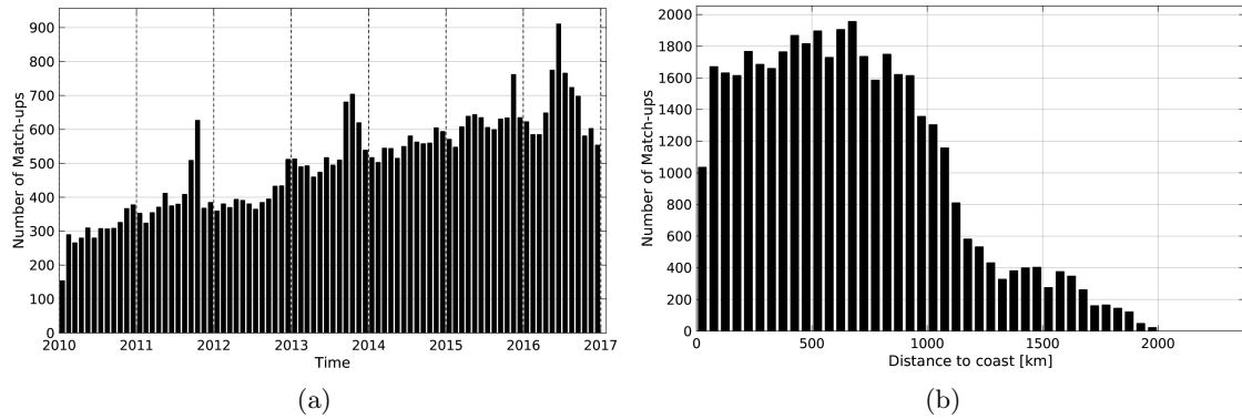
Figure 1: Number of match-ups between Argo and SMOS-L3-CATDS-CECOS-LOCEAN-V2-18DAYS-25KM SSS as a function of time (a) and as function of the distance to coast (b) over the Tropical Atlantic Ocean Pi-MEP region and for the full satellite product period.
