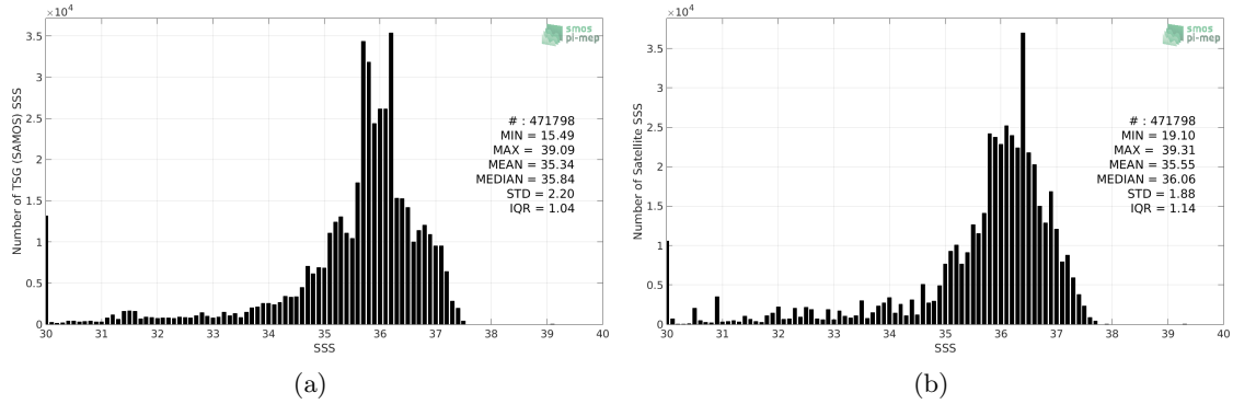
Figure 2: Histograms of SSS from TSG (SAMOS) (a) and SMOS SSS L3 v2 - Monthly - 0.25 Deg (CATDS-CECOS-IFREMER) (b) considering all match-up pairs per bins of 0.1 over the Tropical Atlantic Ocean Pi-MEP region and for the full satellite product period.
