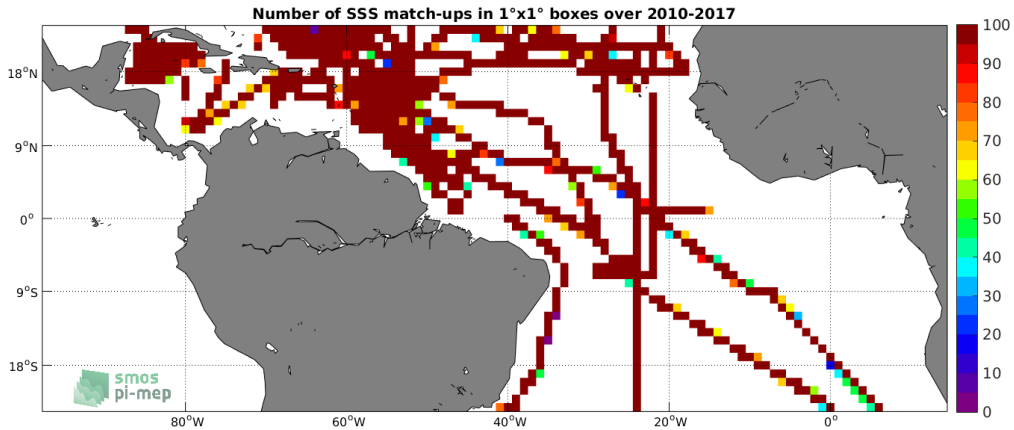
Figure 4: Number of SSS match-ups between TSG (SAMOS) SSS and the SMOS SSS L3 v2 - Monthly - 0.25 Deg (CATDS-CECOS-IFREMER) SSS product for the Tropical Atlantic Ocean Pi-MEP region over 1^\circ \times 1^\circ boxes and for the full satellite product period.
