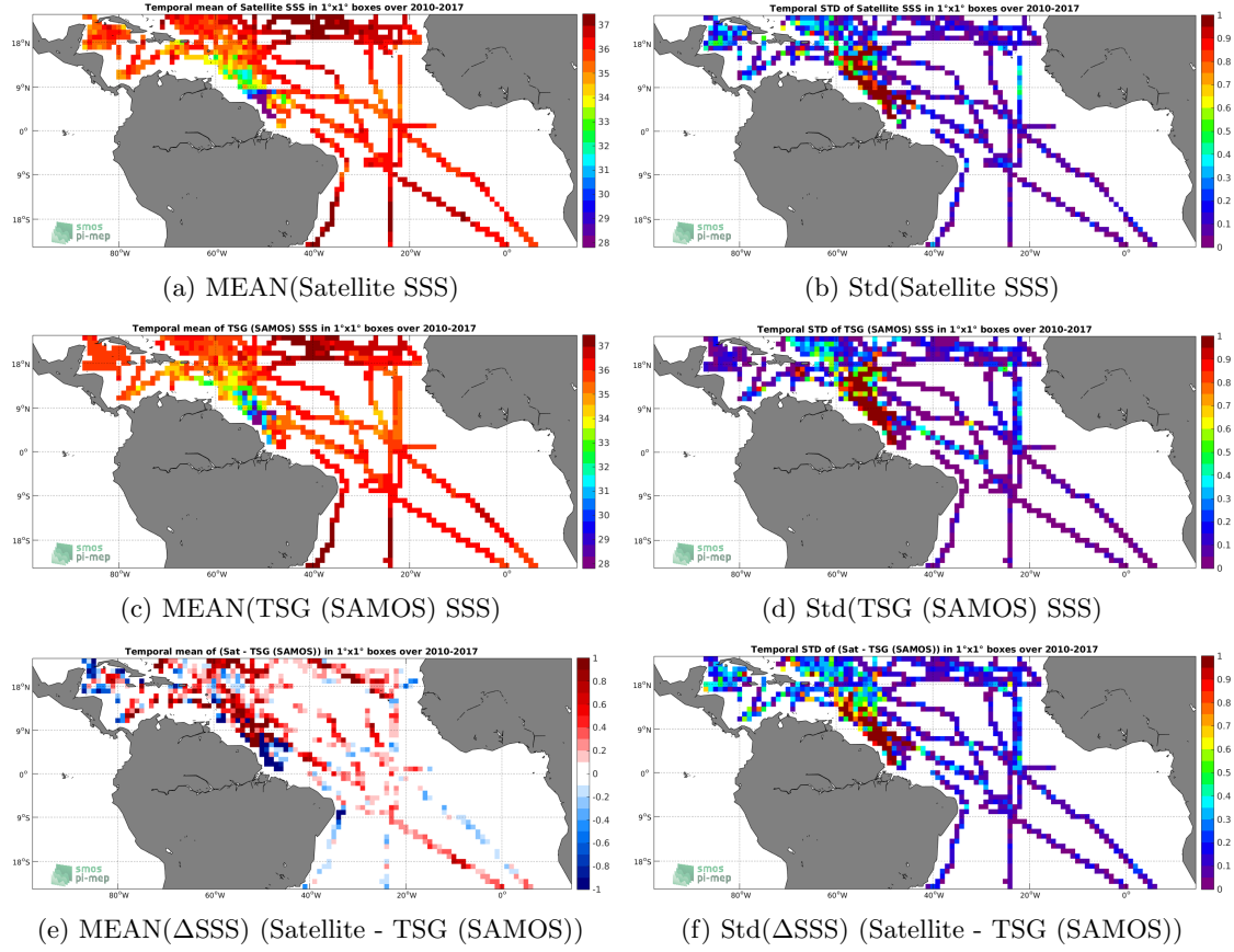
Figure 6: Temporal mean (left) and Std (right) of SSS from SMOS SSS L3 v2 - Monthly - 0.25 Deg (CATDS-CECOS-IFREMER) (top), TSG (SAMOS) (middle), and of \Delta SSS (Satellite - TSG (SAMOS)). Only match-up pairs are used to generate these maps.
