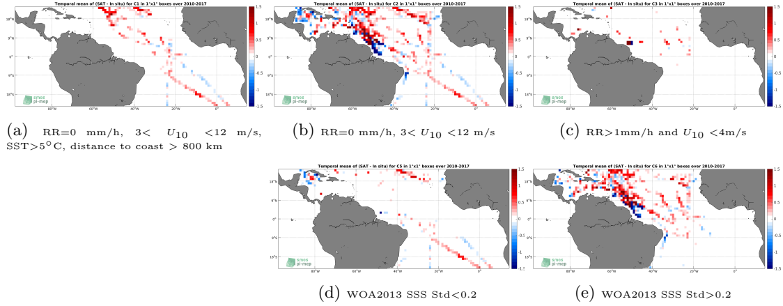
Figure 12: Temporal mean gridded over spatial boxes of size 1^{\circ}\times 1^{\circ} of \Delta\text{SSS} (SMOS SSS L3 v2 - Monthly - 0.25 Deg (CATDS-CECOS-IFREMER) - TSG (SAMOS)) for 5 different subdatasets corresponding to:RR=0 mm/h, 3 < U_{10} < 12 m/s, SST >5^{\circ}\text{C} , distance to coast > 800 km (a), RR=0 mm/h, 3 < U_{10} < 12 m/s (b), RR >1 mm/h and U_{10} < 4 m/s (c), WOA2013 SSS Std <0.2 (d), WOA2013 SSS Std >0.2 (e).
