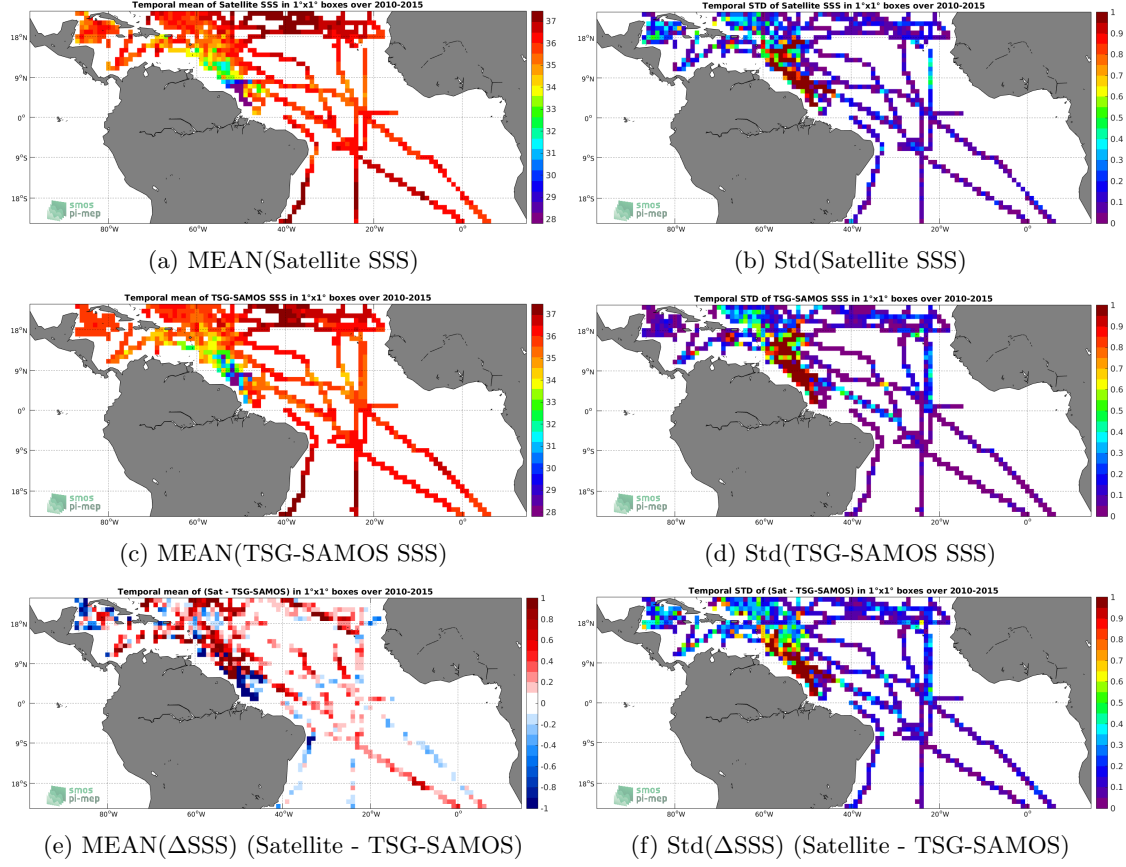
Figure 6: Temporal mean (left) and Std (right) of SSS from SMOS L3 v2 - Monthly - 0.25 Deg (CATDS-CECOS-IFREMER) (top), TSG-SAMOS (middle), and of \Delta SSS (Satellite - TSG-SAMOS). Only match-up pairs are used to generate these maps.
