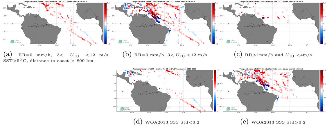
Figure 12: Temporal mean gridded over spatial boxes of size 1^{\circ}\times 1^{\circ} of \Delta\text{SSS} (SMOS L3 v2 - Monthly - 0.25 Deg (CATDS-CECOS-IFREMER) - TSG-SAMOS) for 5 different subdatasets corresponding to: RR=0 mm/h, 3 < U_{10} < 12 m/s, SST > 5^{\circ}\text{C} , distance to coast > 800 km (a), RR=0 mm/h, 3 < U_{10} < 12 m/s (b), RR > 1\text{mm/h} and U_{10} < 4\text{m/s} (c), WOA2013 SSS Std < 0.2 (d), WOA2013 SSS Std > 0.2 (e).
