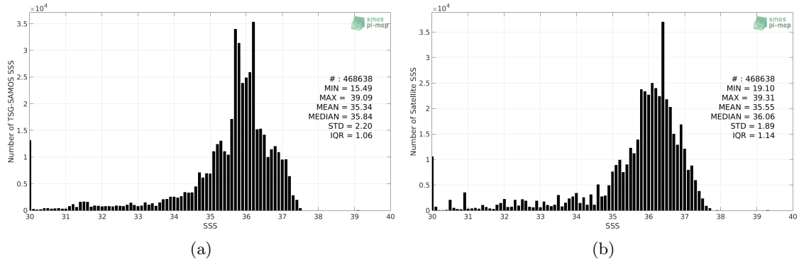
Figure 2: Histograms of SSS from TSG-SAMOS (a) and SMOS L3 v2 - Monthly - 0.25 Deg (CATDS-CECOS-IFREMER) (b) considering all match-up pairs per bins of 0.1 over the Tropical Atlantic Ocean Pi-MEP region and for the full satellite product period.
