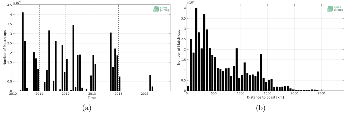
Figure 1: Number of match-ups between TSG-SAMOS and SMOS L3 v2 - Monthly - 0.25 Deg (CATDS-CECOS-IFREMER) SSS as a function of time (a) and as function of the distance to coast (b) over the Tropical Atlantic Ocean Pi-MEP region and for the full satellite product period.
