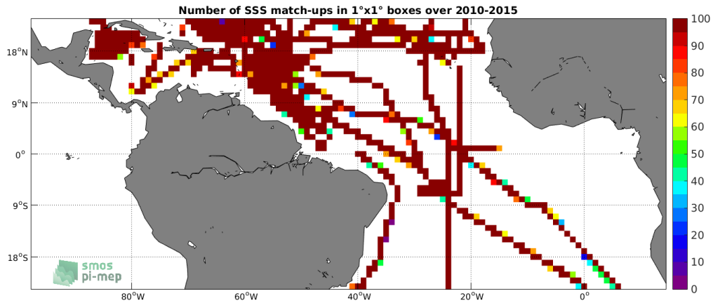
Figure 4: Number of SSS match-ups between TSG-SAMOS SSS and the SMOS L3 v2 - Monthly - 0.25 Deg (CATDS-CECOS-IFREMER) SSS product for the Tropical Atlantic Ocean Pi-MEP region over 1^\circ \times 1^\circ boxes and for the full satellite product period.
