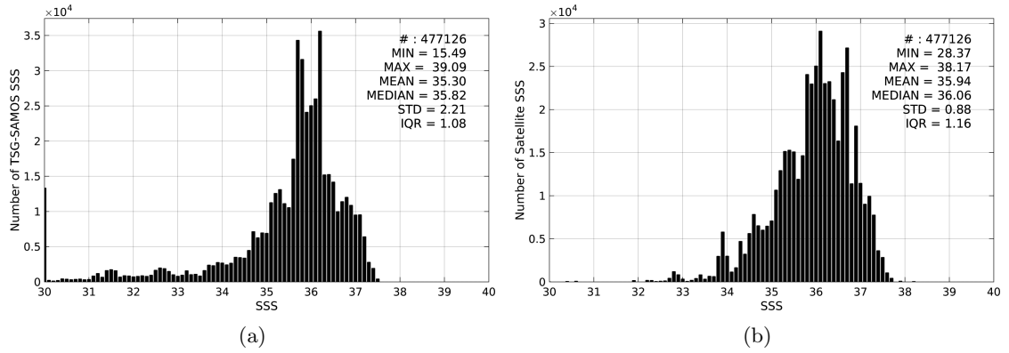
Figure 2: Histograms of SSS from TSG-SAMOS (a) and SMOS-L3-CATDS-IFREMER-CECOS-V2-MONTHLY-0.25DEG (b) considering all match-up pairs per bins of 0.1 over the Tropical Atlantic Ocean Pi-MEP region and for the full satellite product period.
