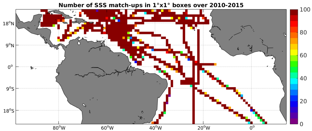
Figure 4: Number of SSS match-ups between TSG-SAMOS SSS and the SMOS-L3-CATDS-IFREMER-CECOS-V2-MONTHLY-0.25DEG SSS product for the Tropical Atlantic Ocean Pi-MEP region over 1^\circ \times 1^\circ boxes and for the full satellite product period.
