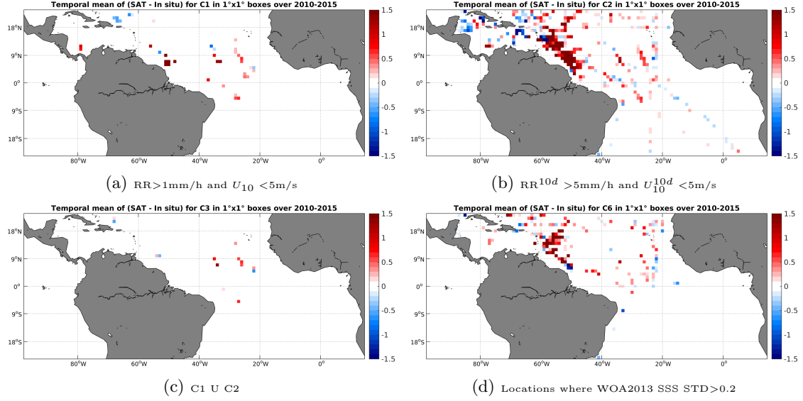
Figure 12: Temporal mean gridded over spatial boxes of size 1^\circ \times 1^\circ of \Delta SSS (SMOS-L3-CATDS-IFREMER-CECOS-V2-MONTHLY-0.25DEG - TSG-SAMOS) for 4 different subdatasets corresponding to: RR > 1\text{mm/h} and U_{10} < 5\text{m/s} (a), RR^{10d} > 5\text{mm/h} and U_{10}^{10d} < 5\text{m/s} (b), C1 U C2 (c), Locations where WOA2013 SSS STD > 0.2 (d).
