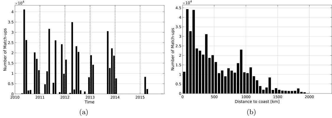
Figure 1: Number of match-ups between TSG-SAMOS and SMOS-L3-CATDS-IFREMER-CECOS-V2-MONTHLY-0.25DEG SSS as a function of time (a) and as function of the distance to coast (b) over the Tropical Atlantic Ocean Pi-MEP region and for the full satellite product period.
