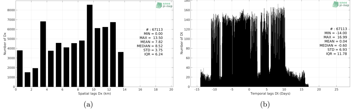
Figure 5: Histograms of the spatial (a) and temporal (b) lags between the time of the TSG (Polarstern) measurements and the date of the corresponding SMOS SSS L3 v2 - Monthly - 0.25 Deg (CATDS-CECOS-IFREMER) SSS product.
