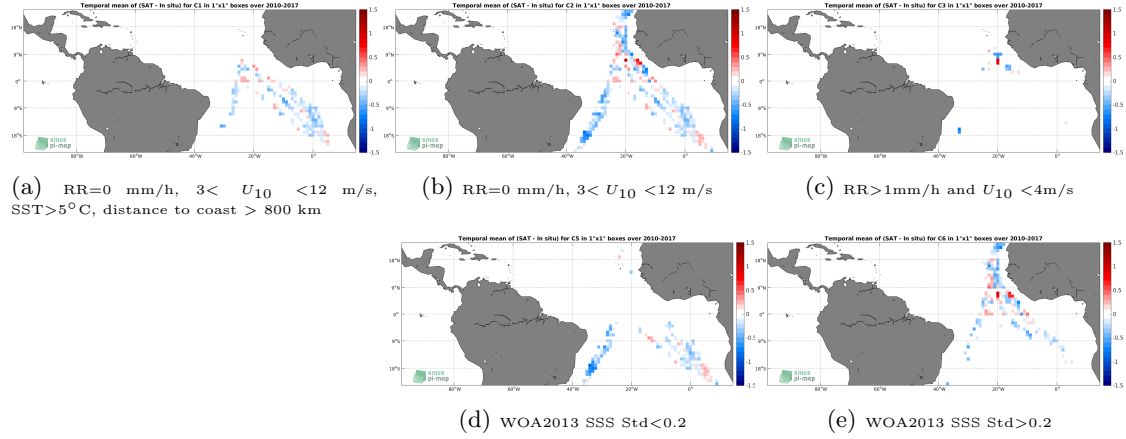
Figure 12: Temporal mean gridded over spatial boxes of size 1^{\circ}\times 1^{\circ} of \Delta\text{SSS} (SMOS SSS L3 v2 - Monthly - 0.25 Deg (CATDS-CECOS-IFREMER) - TSG (Polarstern)) for 5 different subdatasets corresponding to:RR=0 mm/h, 3 < U_{10} < 12 m/s, SST >5^{\circ}\text{C} , distance to coast > 800 km (a), RR=0 mm/h, 3 < U_{10} < 12 m/s (b), RR >1 mm/h and U_{10} < 4 m/s (c), WOA2013 SSS Std <0.2 (d), WOA2013 SSS Std >0.2 (e).
