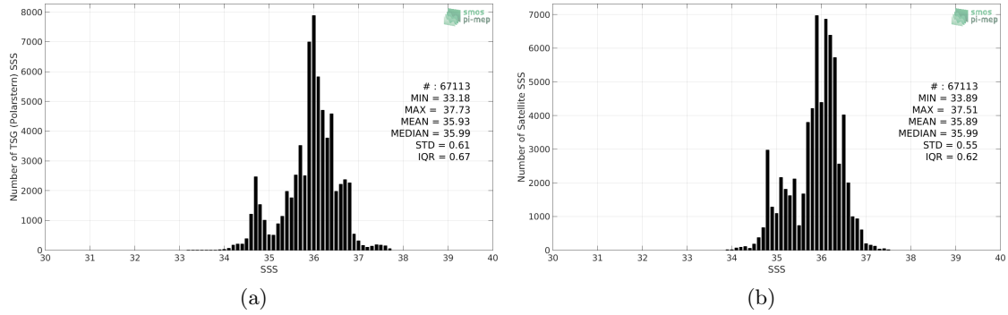
Figure 2: Histograms of SSS from TSG (Polarstern) (a) and SMOS SSS L3 v2 - Monthly - 0.25 Deg (CATDS-CECOS-IFREMER) (b) considering all match-up pairs per bins of 0.1 over the Tropical Atlantic Ocean Pi-MEP region and for the full satellite product period.
