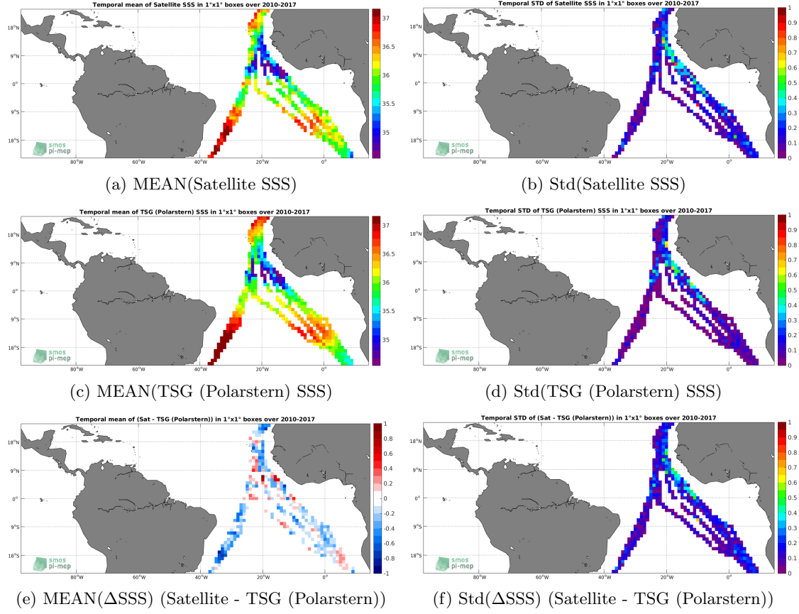
Figure 6: Temporal mean (left) and Std (right) of SSS from SMOS SSS L3 v2 - Monthly - 0.25 Deg (CATDS-CECOS-IFREMER) (top), TSG (Polarstern) (middle), and of \Delta SSS (Satellite - TSG (Polarstern)). Only match-up pairs are used to generate these maps.
