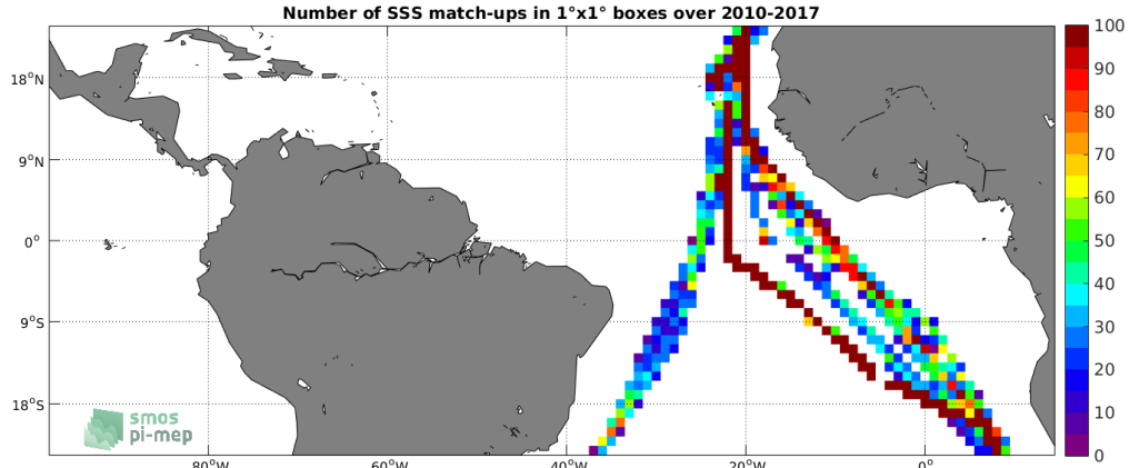
Figure 4: Number of SSS match-ups between TSG (Polarstern) SSS and the SMOS SSS L3 v2 - Monthly - 0.25 Deg (CATDS-CECOS-IFREMER) SSS product for the Tropical Atlantic Ocean Pi-MEP region over 1^\circ \times 1^\circ boxes and for the full satellite product period.
