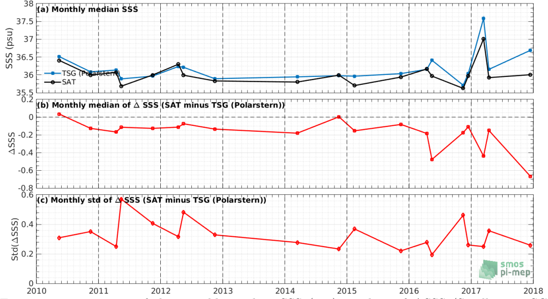
Figure 7: Time series of the monthly median SSS (top), median of \Delta\text{SSS} (Satellite - TSG (Polarstern)) and Std of \Delta\text{SSS} (Satellite - TSG (Polarstern)) over the Tropical Atlantic Ocean Pi-MEP region considering all match-ups collected by the Pi-MEP.
